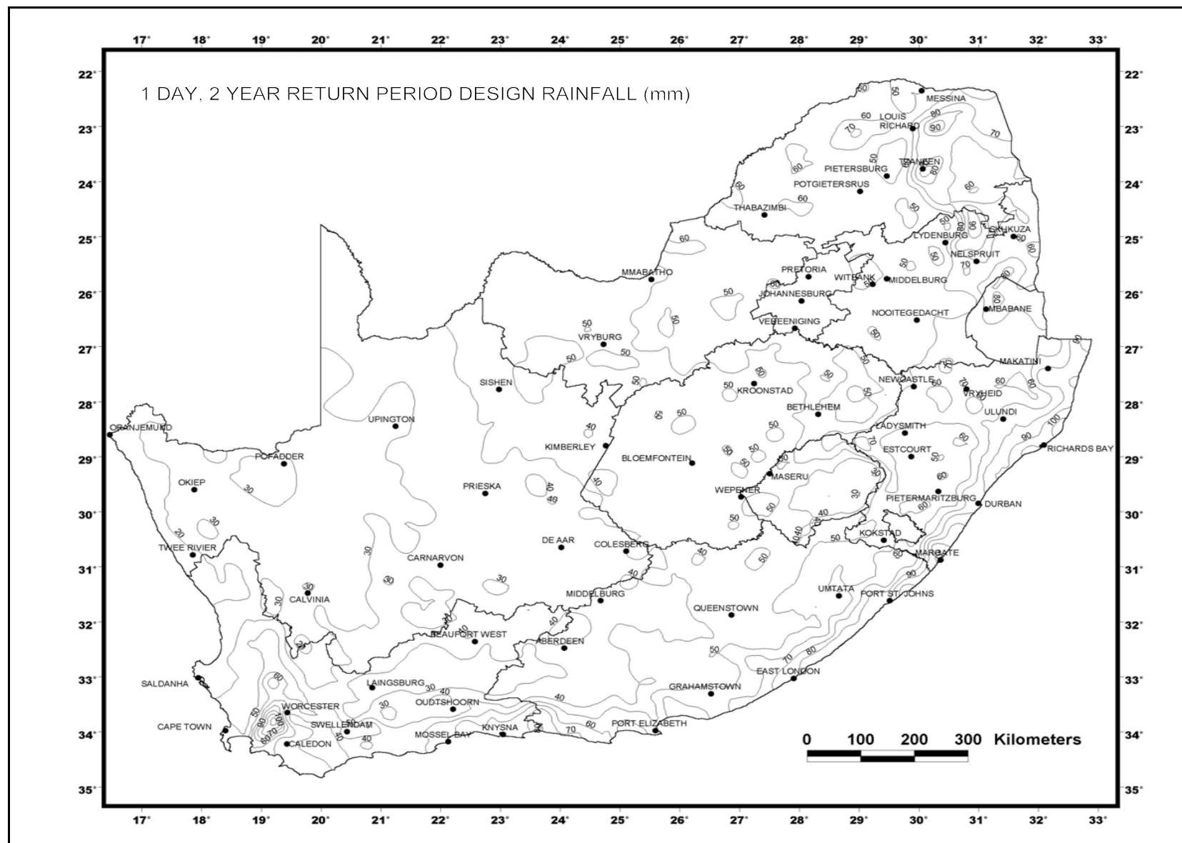
Figure 84 Contour map of 1 day, 2 year return period design rainfall in for South Africa
