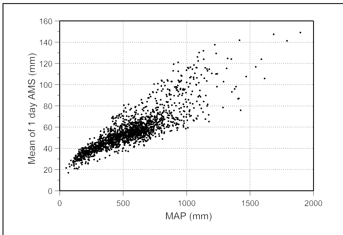
Figure 29 Relationship between the means of 1 day AMS and MAP (computed from the observed data) for concurrent periods calculated using records from 1 806 daily rainfall stations in South Africa which have at least 40 years of observed record
