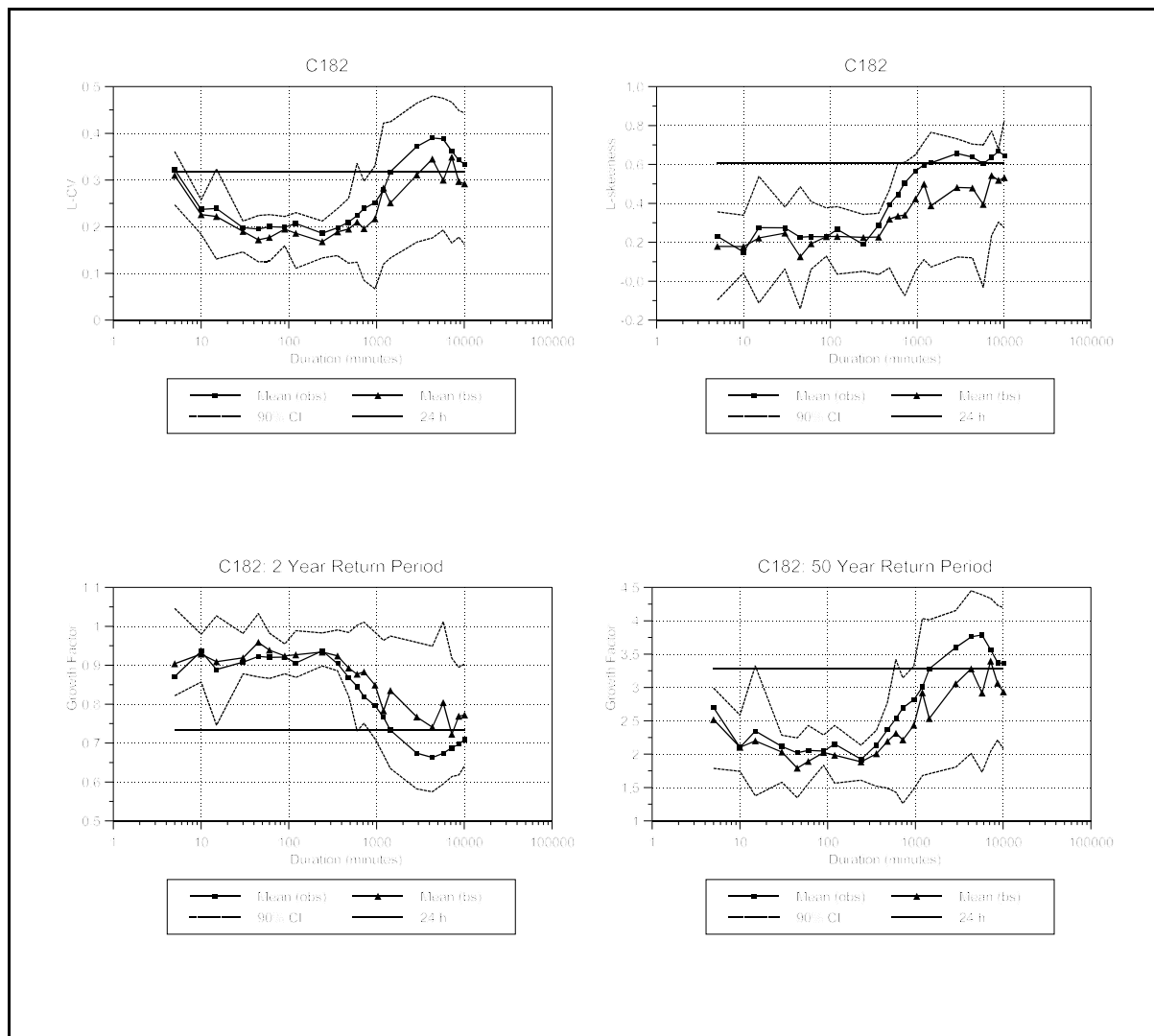
Figure 19 90% Confidence limits for L-moment ratios, 2 and 50 year return period growth factors established from 1000 bootstrapped samples at Raingauge C182 (Cedar)
