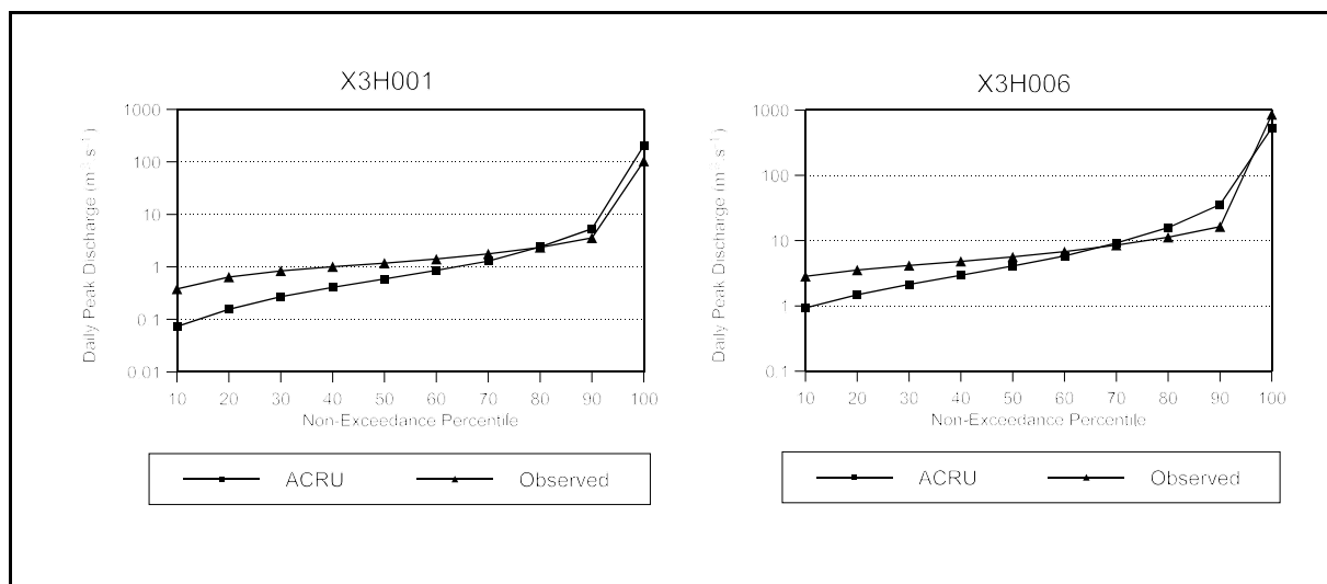
Figure 80 Frequency analysis of simulated and observed daily peak discharges at Gauging Weirs X3H001 and X3H006 (after Smithers et al. , 2001)
