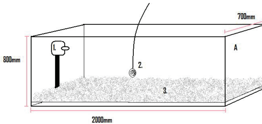
A - 350L Fibreglass tank
