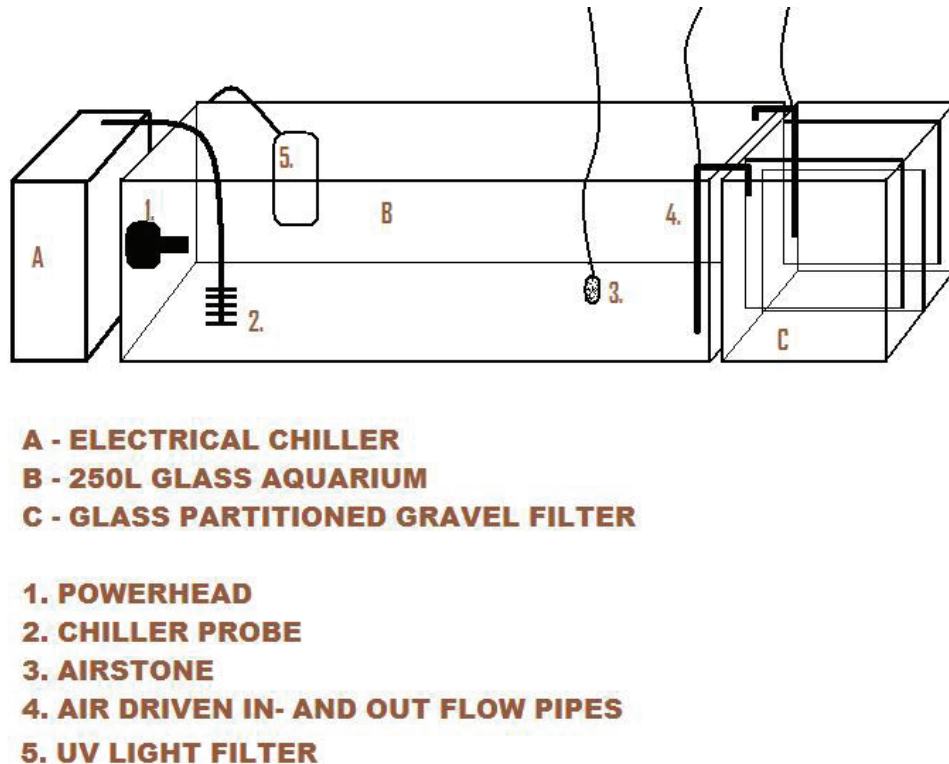
Figure 3.7.1: Technical layout of the brood stock housing tanks.
