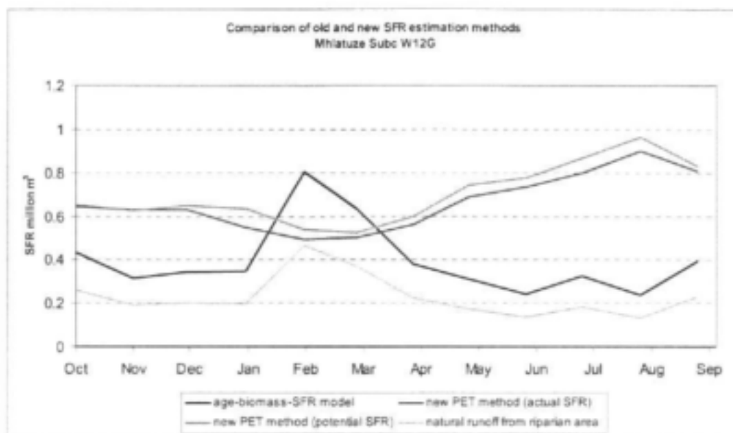
Figure 3-6: Comparison of Old and New Riparian SFR Estimation Models for a Subcatchment in the Mhlathuze
