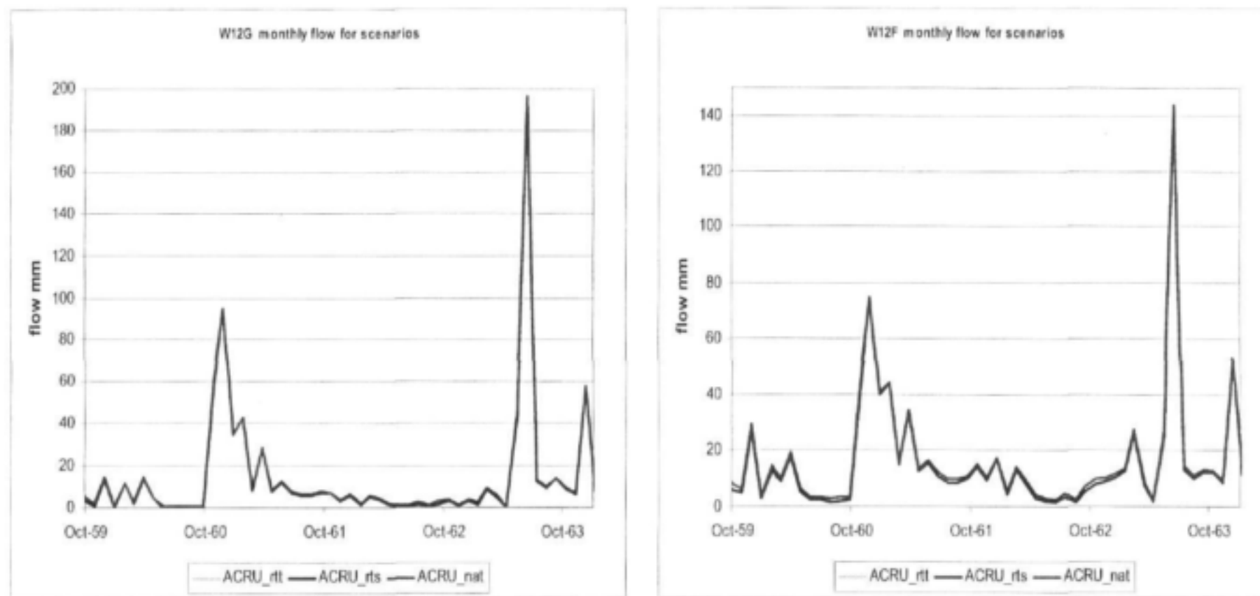
Figure 5-18: Monthly Time Series of Flow Produced by ACRU for Riparian Scenarios in Subcatchments W12F and W12G in Mhlathuze
