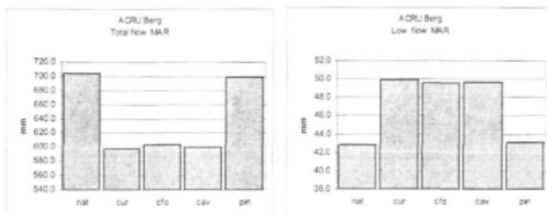
Figure 5-19: MAR Estimates Produced by ACRU for the Upper Berg
