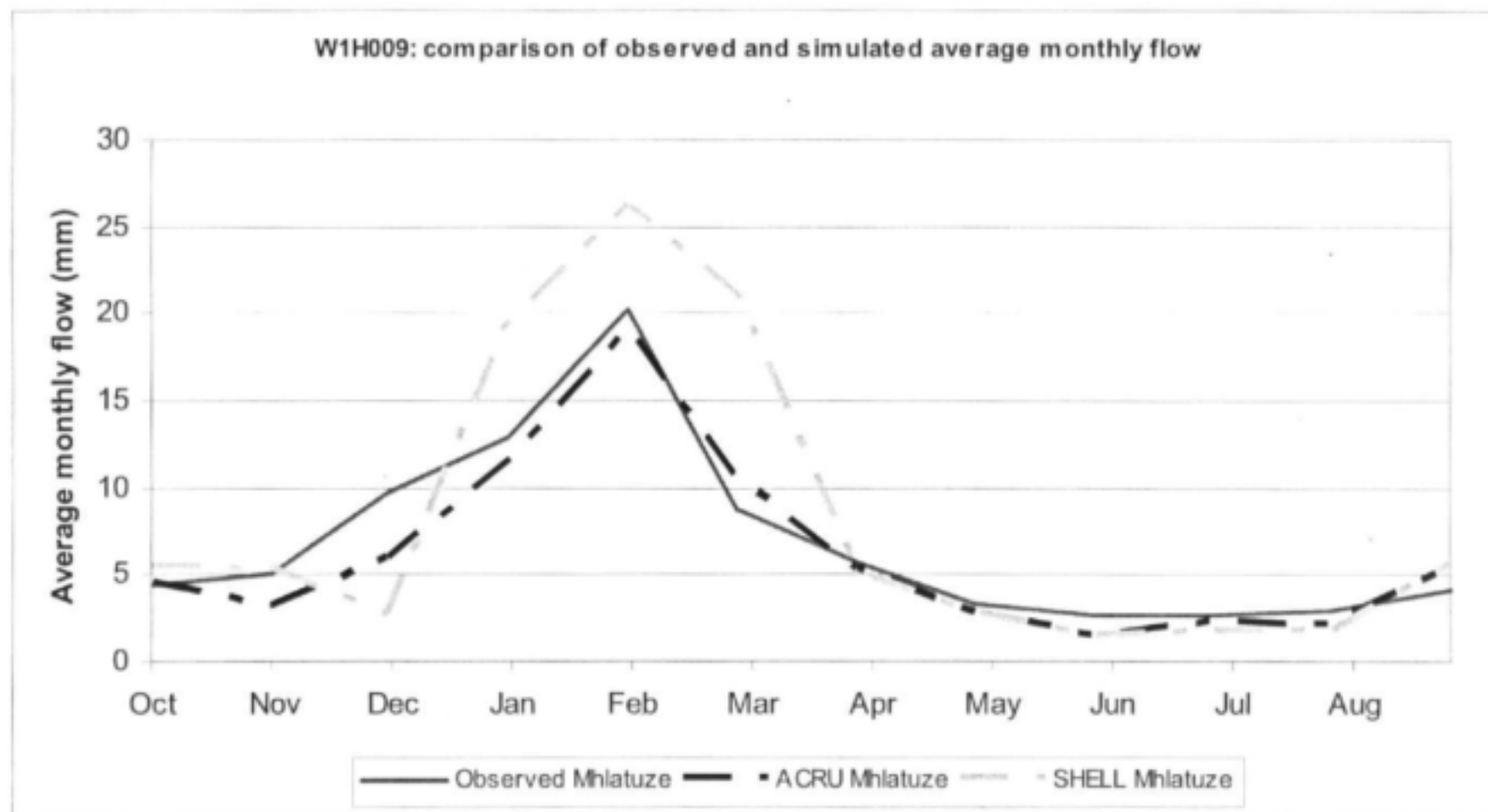
Figure 5-10: Average Monthly Plot of Observed and Simulated Flows from SHELL and ACRU at Gauge W1H009 in the Mhlatuze
