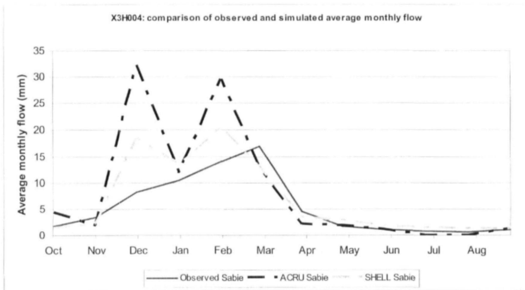
Figure 5-6: Average monthly plot of observed and simulated flows from SHELL and ACRU at gauge X3H004 in the Upper Sabie for a Ten Year Simulation Period (1986 to 1996)
