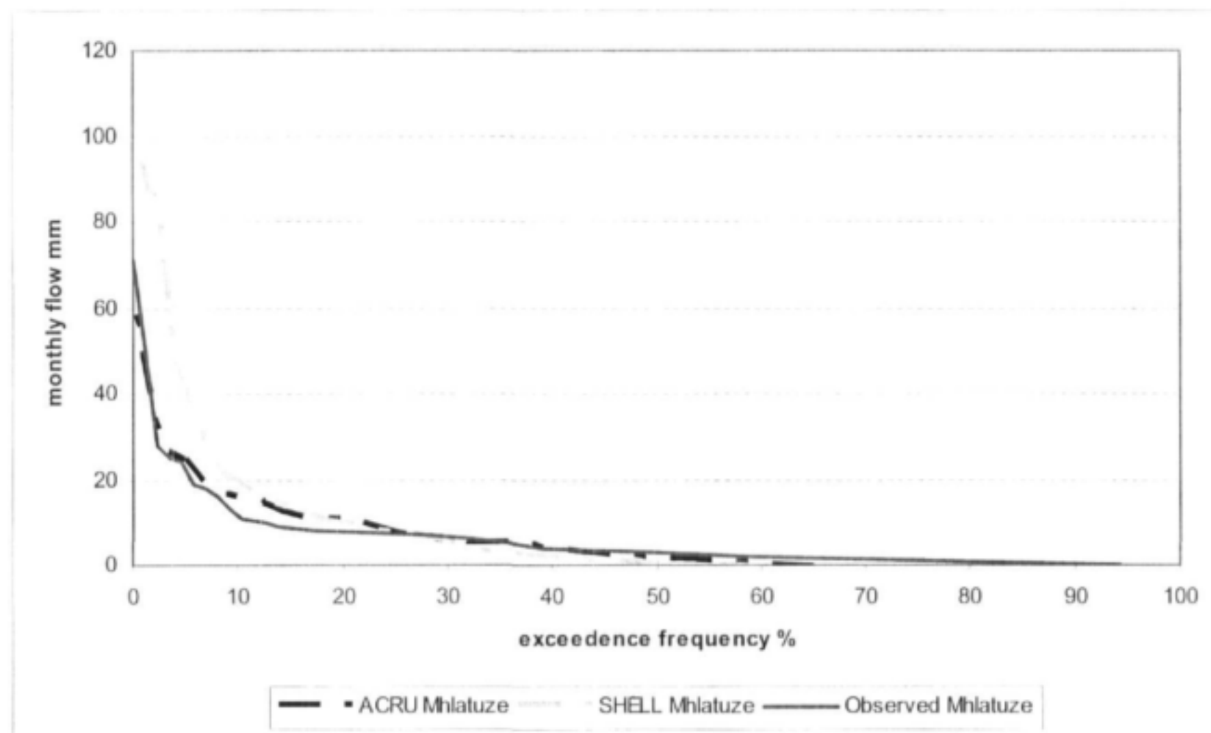
Figure 5-9: Cumulative Frequency Exceedence Plot of Monthly Observed and Simulated Flows from SHELL and ACRU at Gauge W1H009 in the Mhlatuze
