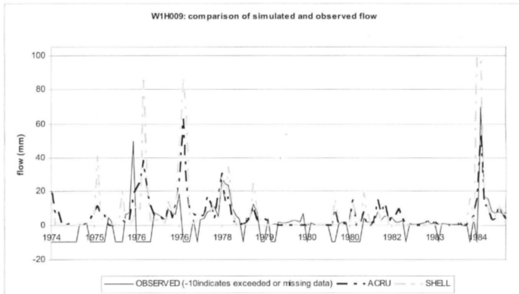
Figure 5-8: Monthly Observed and Simulated Flow for SHELL and ACRU at Gauge W1H009 in the Mhlatuze
