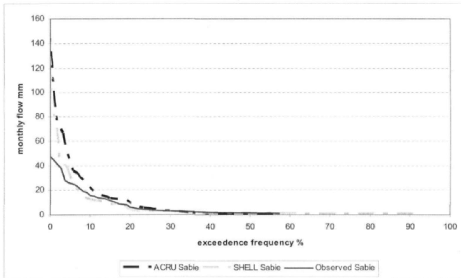
Figure 5-5: Cumulative Exceedence Frequency Plot of Monthly Observed and Simulated Flows from SHELL and ACRU at Gauge X3H004 in the Upper Sabie
