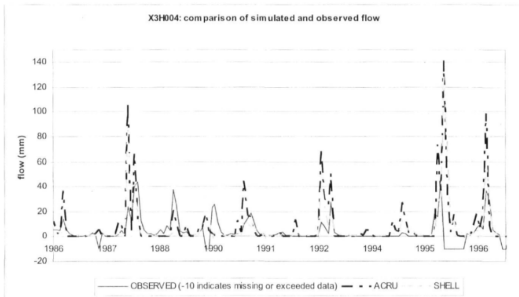
Figure 5-4: Monthly Observed and Simulated Flow for SHELL and ACRU at Gauge X3H004 in Upper Sabie
