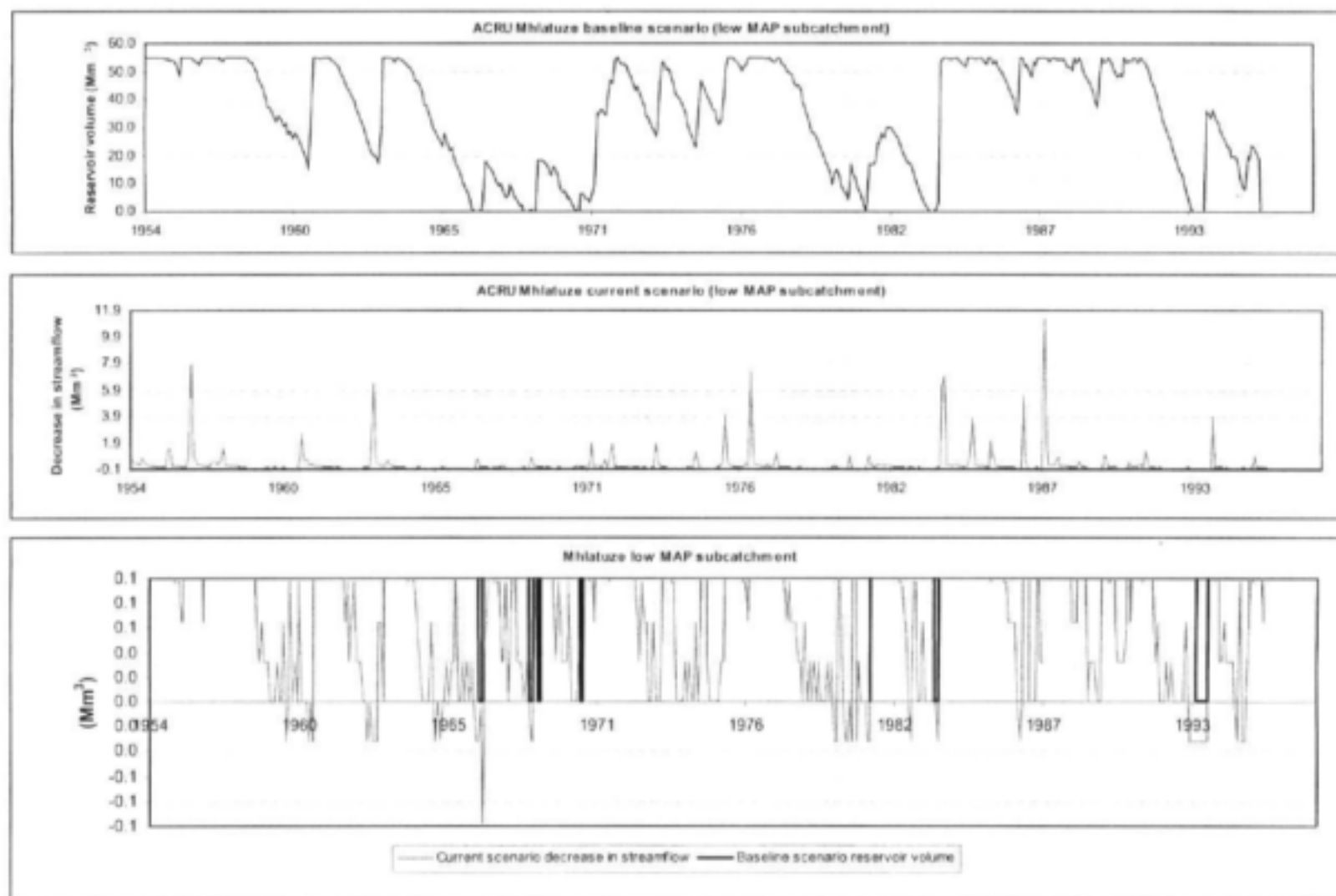
Figure 6-3: Comparison of Yield Reservoir Volume for the ACRU 1 in 5 year Baseline Scenario and Decrease in Baseline Streamflow for the ACRU Current Scenario for the Low MAP Mhlaluzi Catchment
