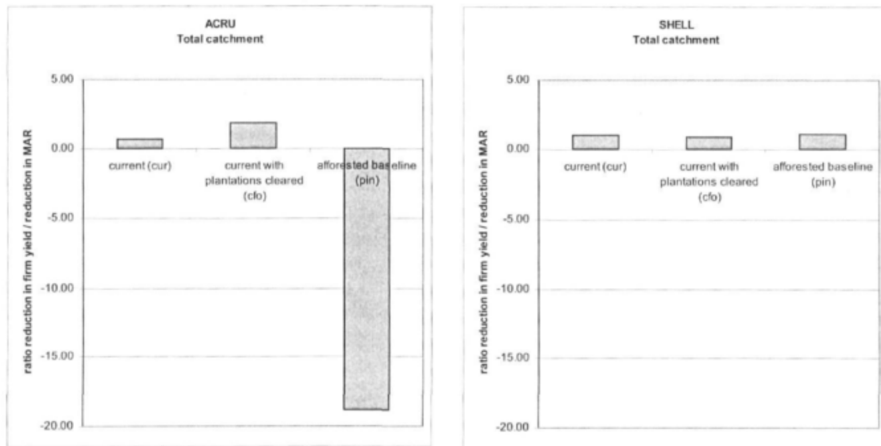
Figure 6-5: Summary of Yield Modelling Results for the Upper Sabie
