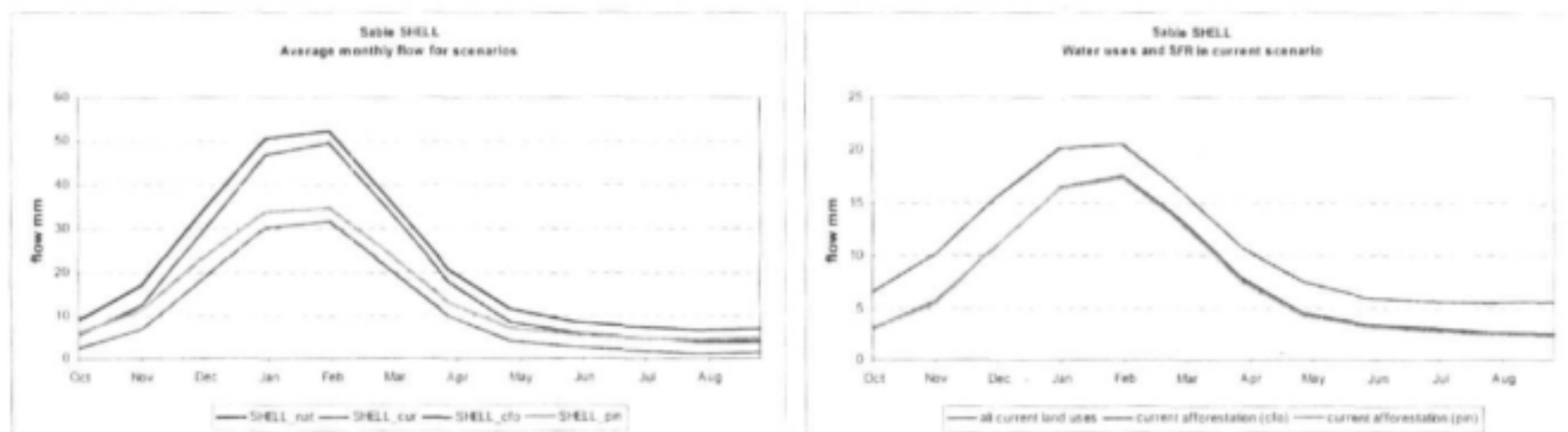
Figure 5-23: Seasonal Distribution of Flows and Reductions for Sabie ACRU Scenarios
