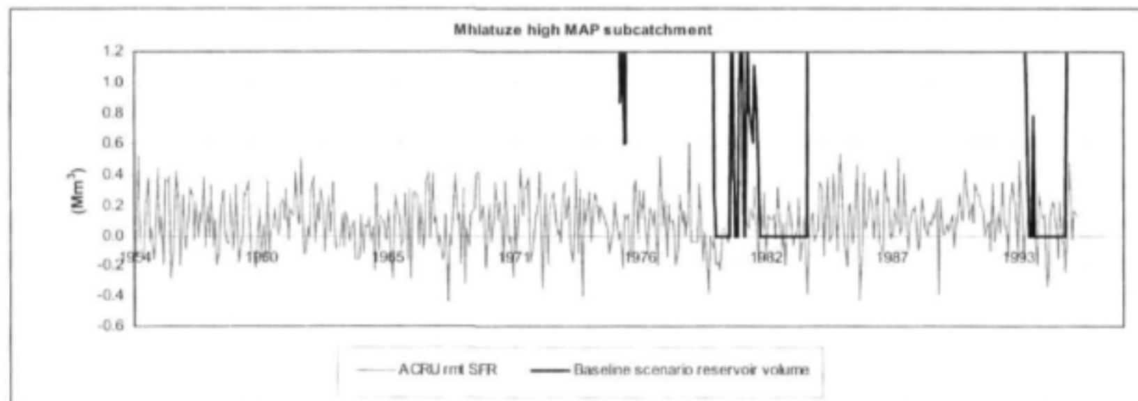
Figure 6-2: (continued) Comparison of Yield Reservoir Volume for the ACRU 1 in 5 year Baseline Scenario and SFR for ACRU Scenarios for the High MAP Mhlaluze Catchment
