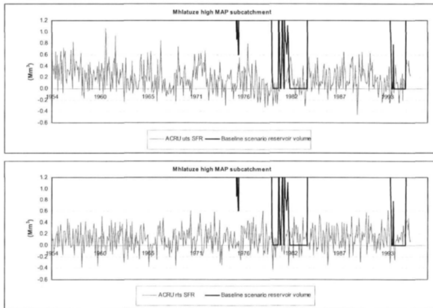
Figure 6-2: (continued) Comparison of Yield Reservoir Volume for the ACRU 1 in 5 year Baseline Scenario and SFR for ACRU Scenarios for the High MAP Mhlataze Catchment
