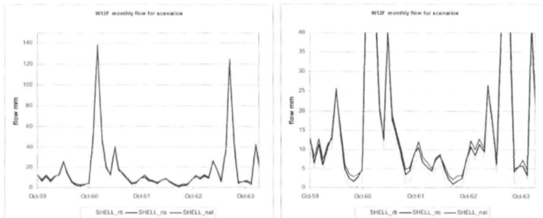
Figure 5-29: Monthly Time Series of Flow Produced by SHELL for Riparian Scenarios in Subcatchment W12F in the Mhlatuze
