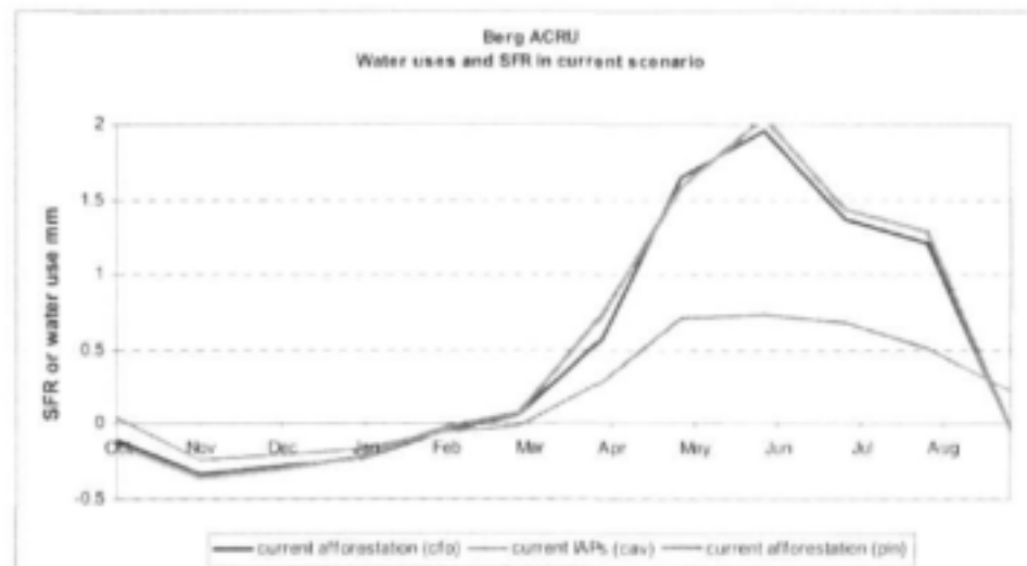
Figure 5-20: Seasonal Distribution of Flows and Reductions for the Upper Berg ACRU Scenarios
