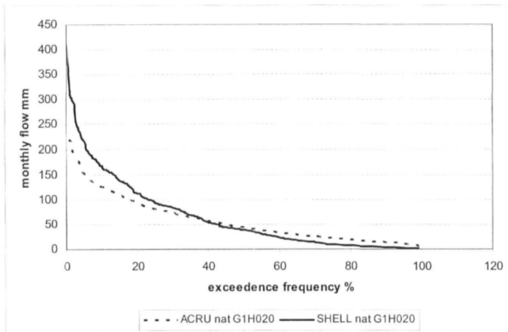
Figure 5-11: Cumulative Exceedence Frequency Plot of Baseline Monthly Flows Produced by SHELL and ACRU for the Total Upper Berg Catchment
