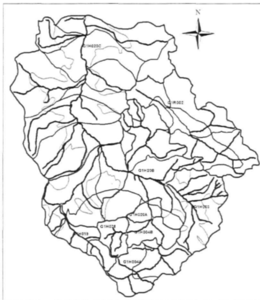
Figure 4-2: Subcatchment Configuration of the Upper Berg
