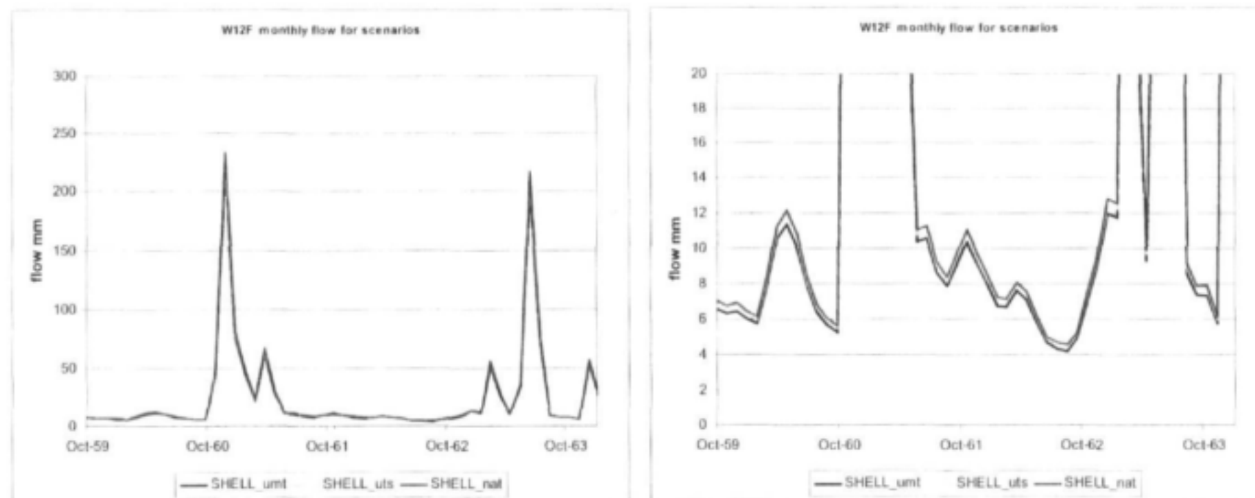
Figure 5-28: Monthly Time Series of Flow Produced by SHELL for Upland Scenarios in Subcatchment W12F in the Mhlaluze
