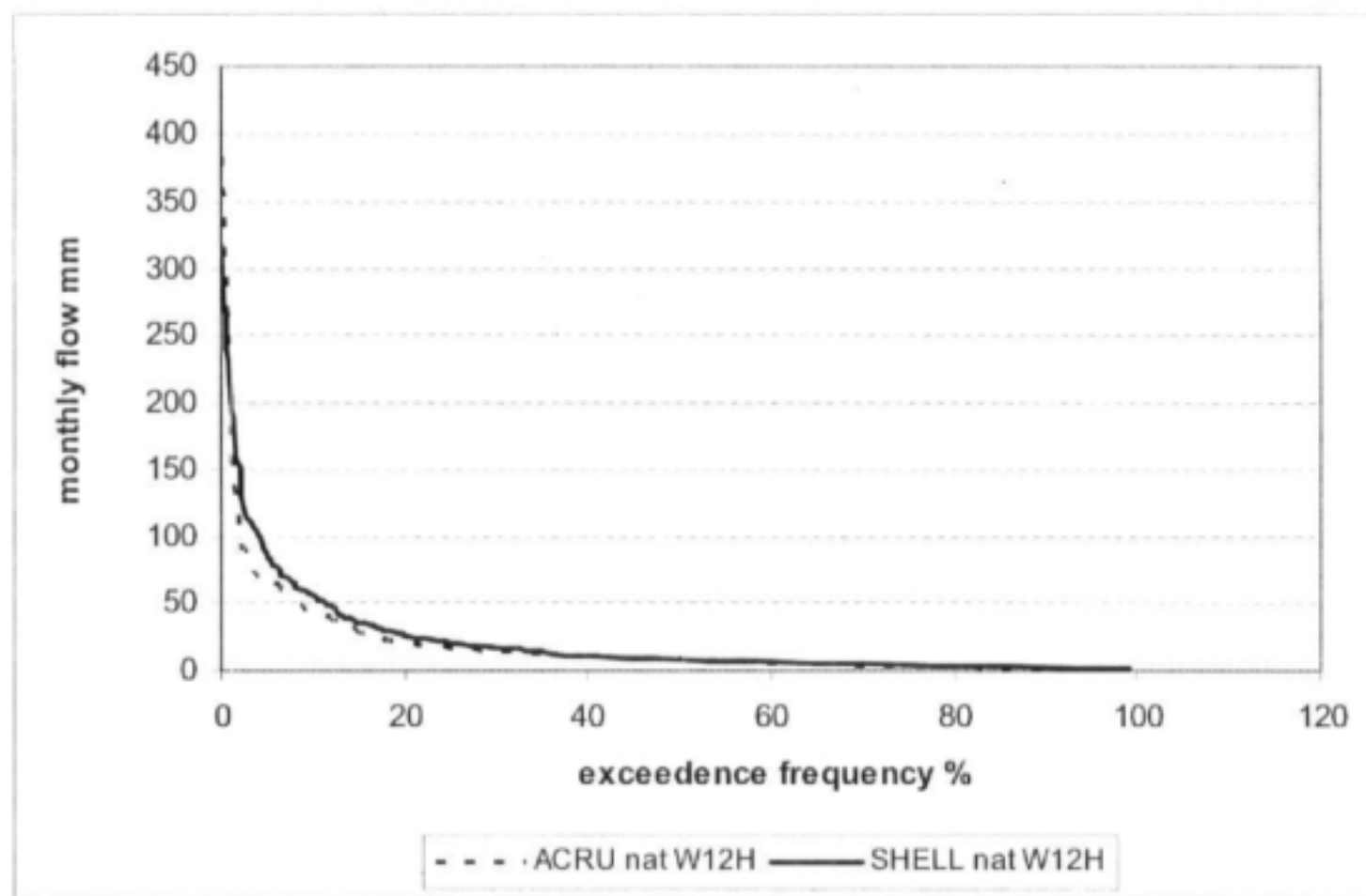
Figure 5-13: Cumulative Exceedence Frequency Plot of Baseline Monthly Flow Produced by SHELL and ACRU for the Total Mhlatauze Catchment
