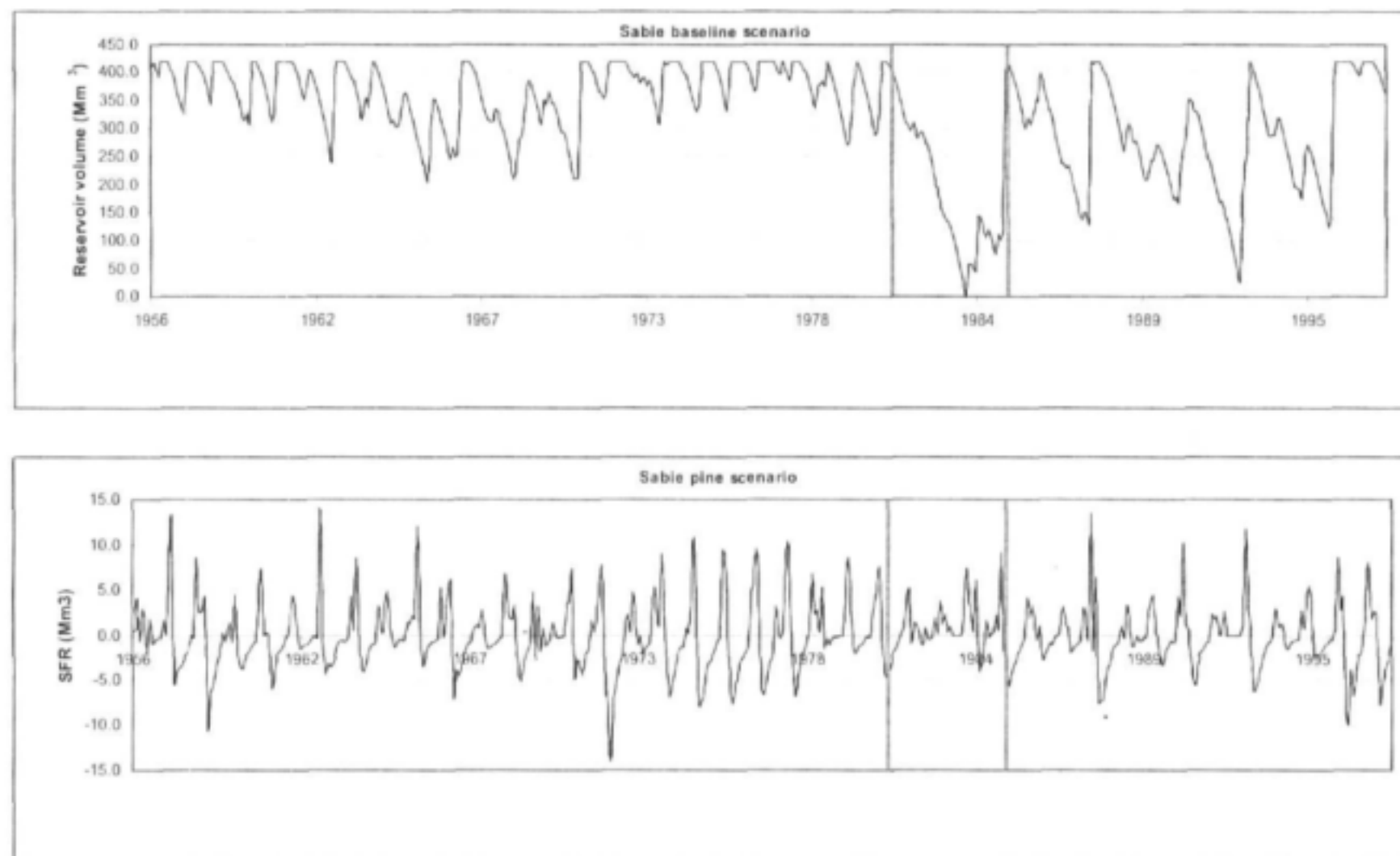
Figure 6-6: Comparison of Yield Reservoir Volume for the ACRU Baseline Scenario and SFR for the ACRU Pine Scenario for the Total Sable Catchment
