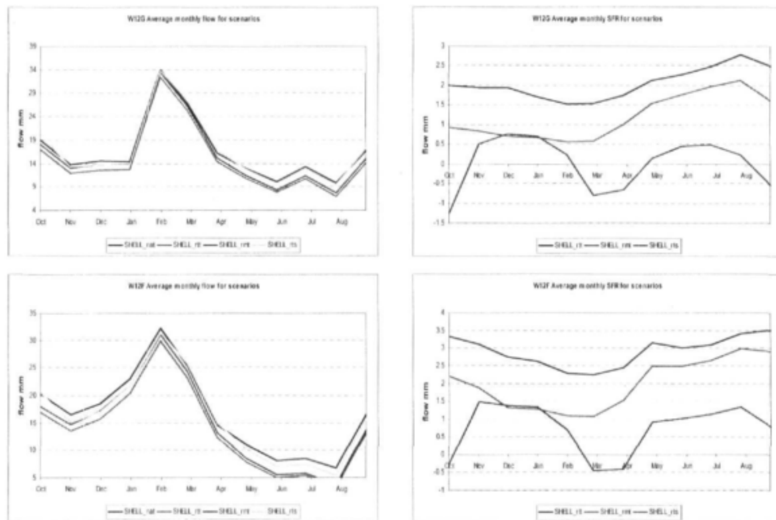
Figure 5-27 : Average Monthly SFR Produced by SHELL for Subcatchments in the Mhlathuze for Riparian IAP Scenarios
