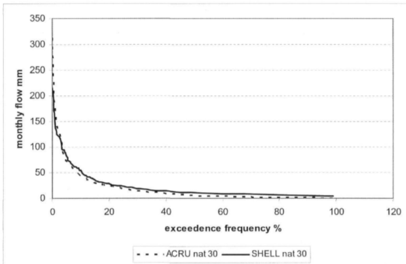
Figure 5-12: Cumulative Exceedence Frequency Plot of Baseline Monthly Flows Produced by SHELL and ACRU for the Total Upper Sabie Catchment
