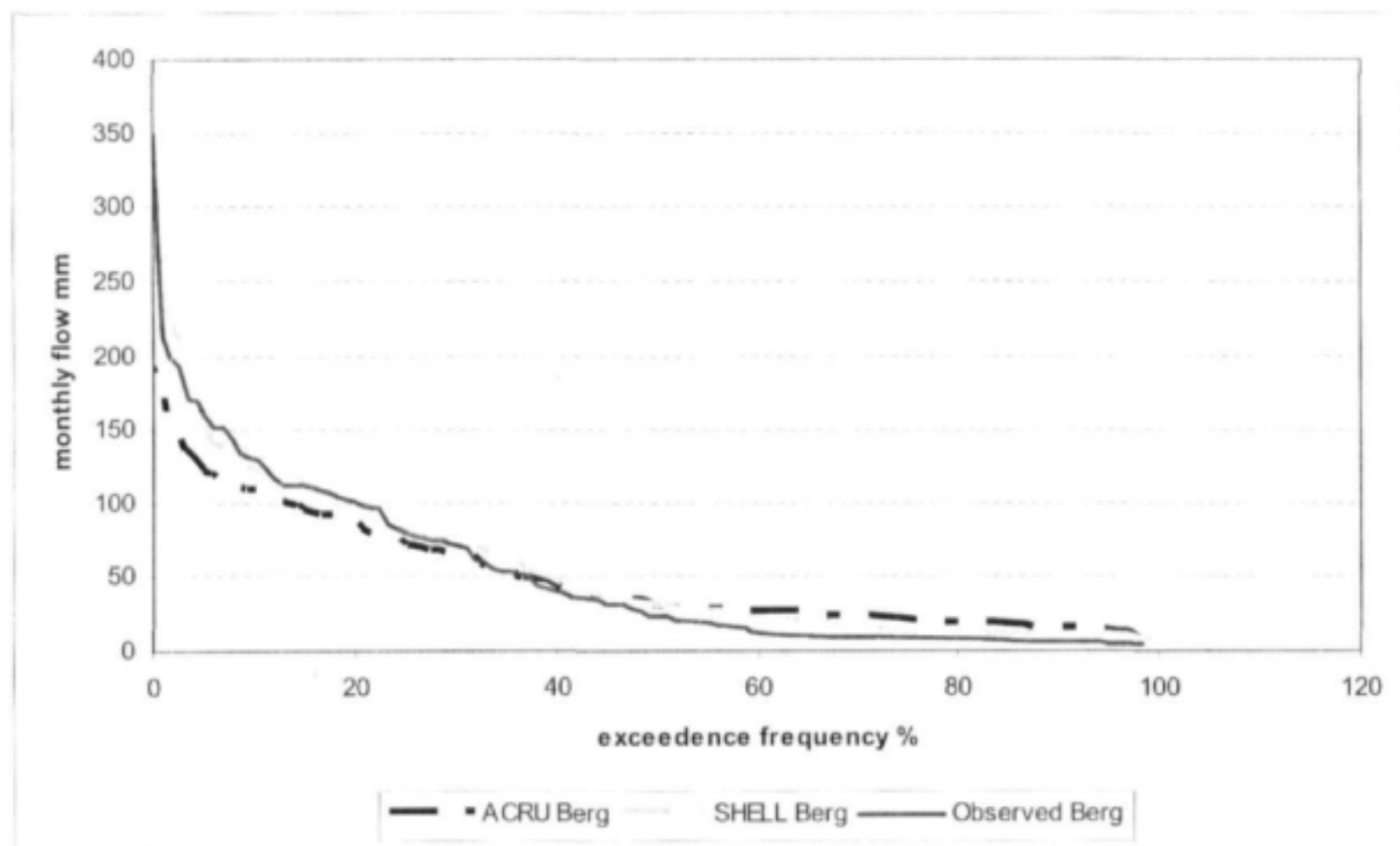
Figure 5-2: Cumulative Exceedence Frequency Plot of Monthly Observed and Simulated Flows from SHELL and ACRU at Gauge G1H020 in the Upper Berg
