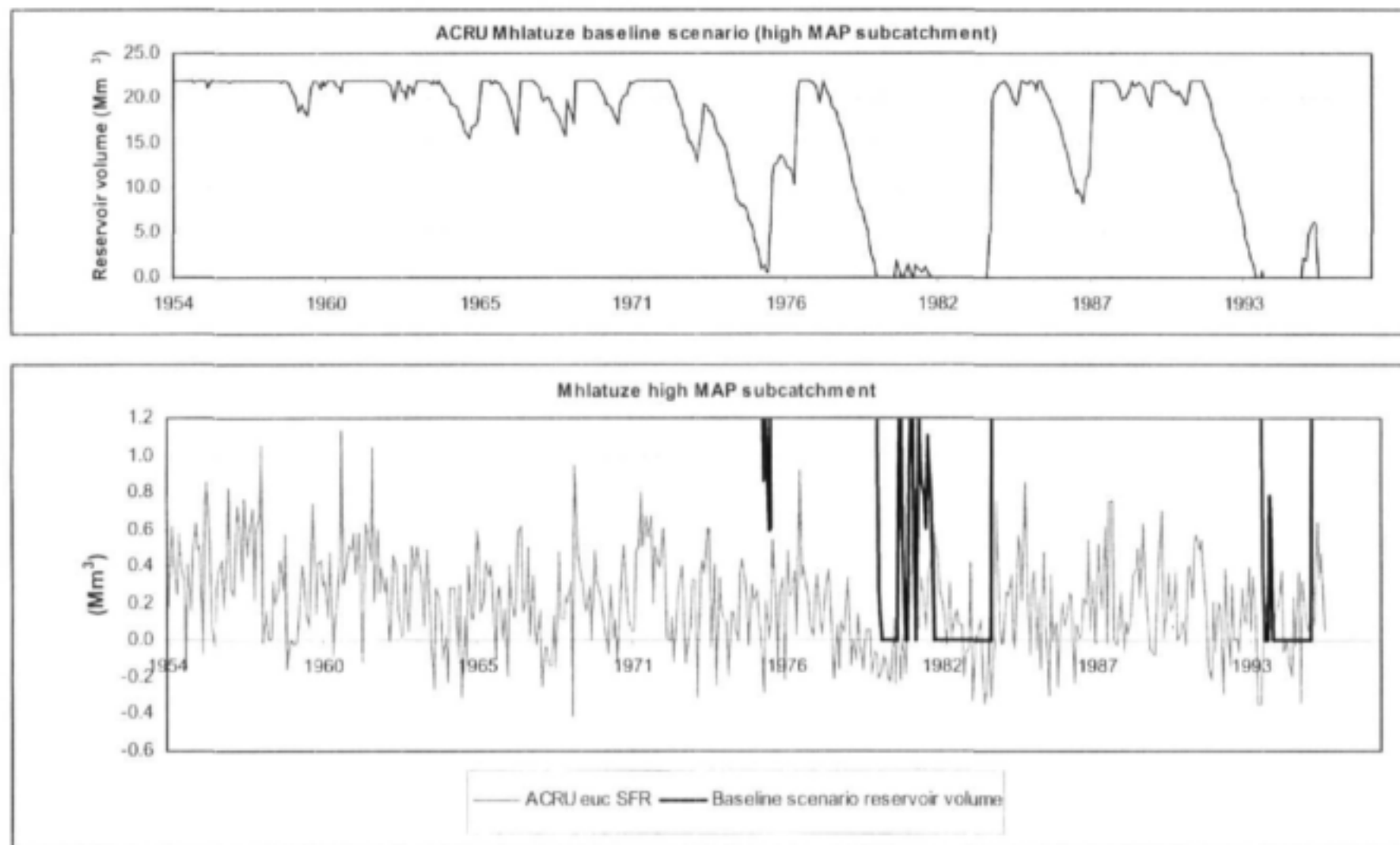
Figure 6-2: Comparison of Yield Reservoir Volume for the ACRU 1 in 5 year Baseline Scenario and SFR for ACRU Scenarios for the High MAP Mhlutuze Catchment
