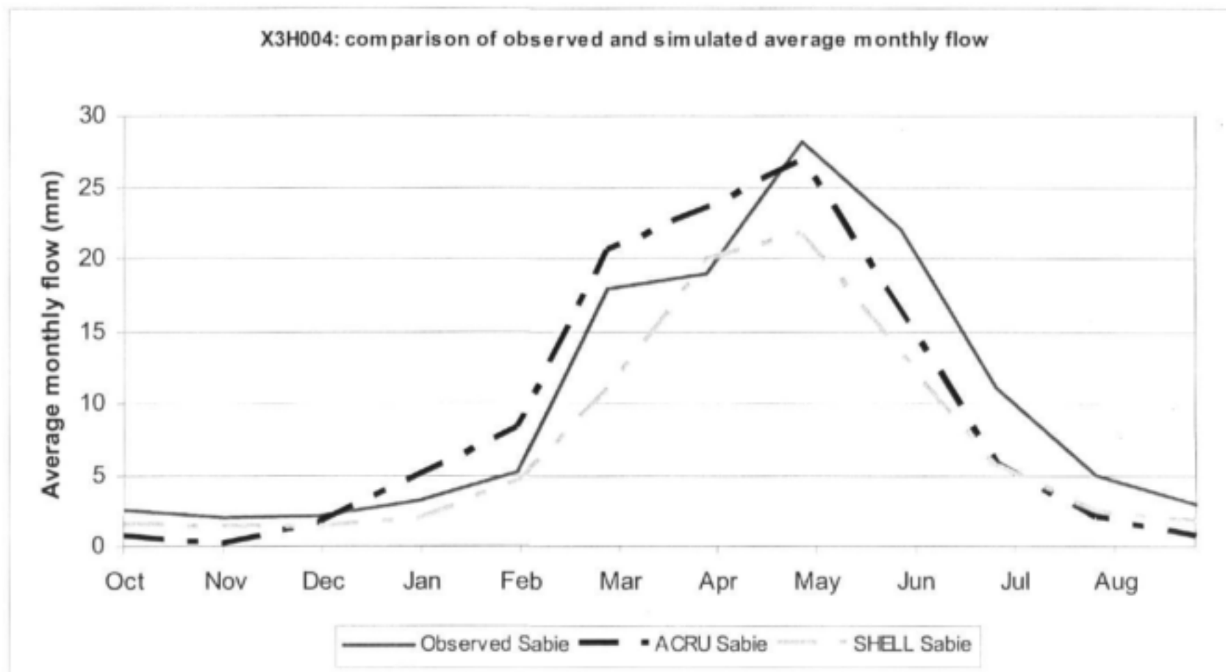
Figure 5-7: Average Monthly Plot of Observed and Simulated Flows from SHELL and ACRU at Gauge X3H004 in the Upper Sabie for a Forty Year Simulation Period (1956 to 1996)
