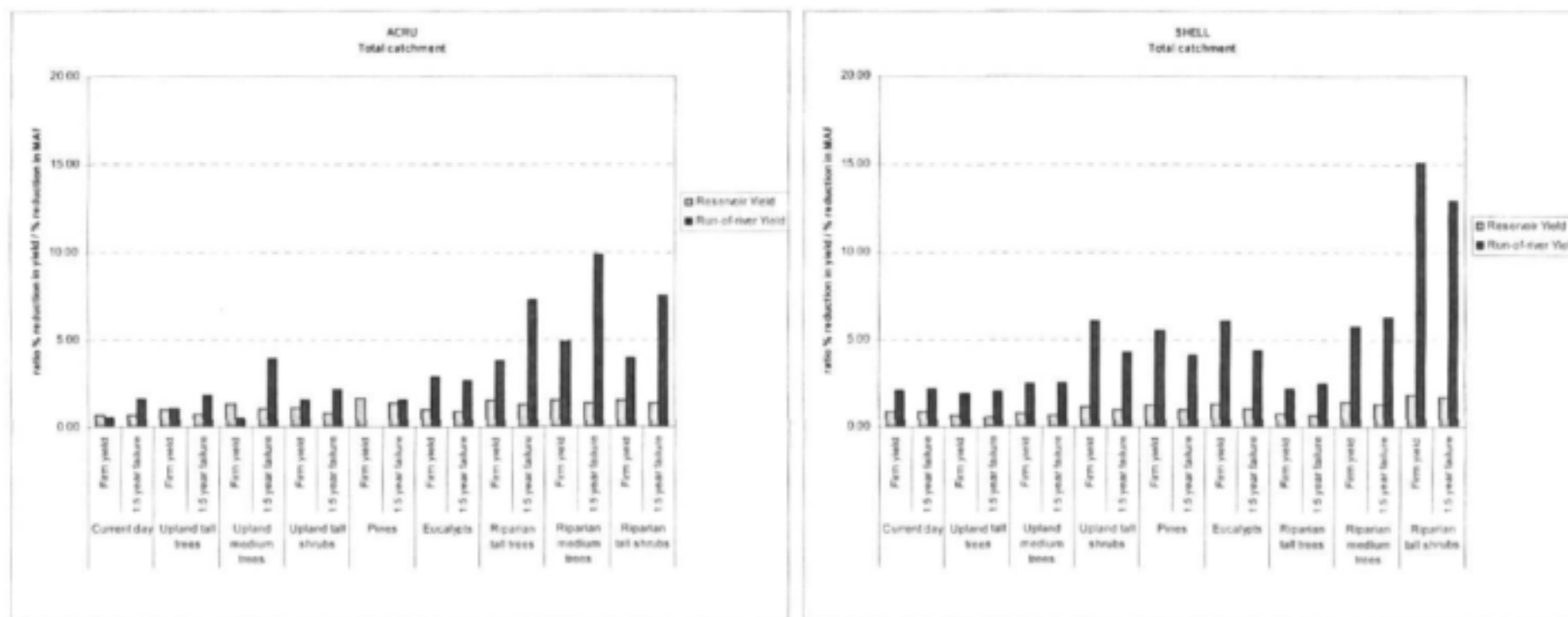
Figure 6-1: (continued) Summary of Yield Modelling Results for the Mhlathuze
