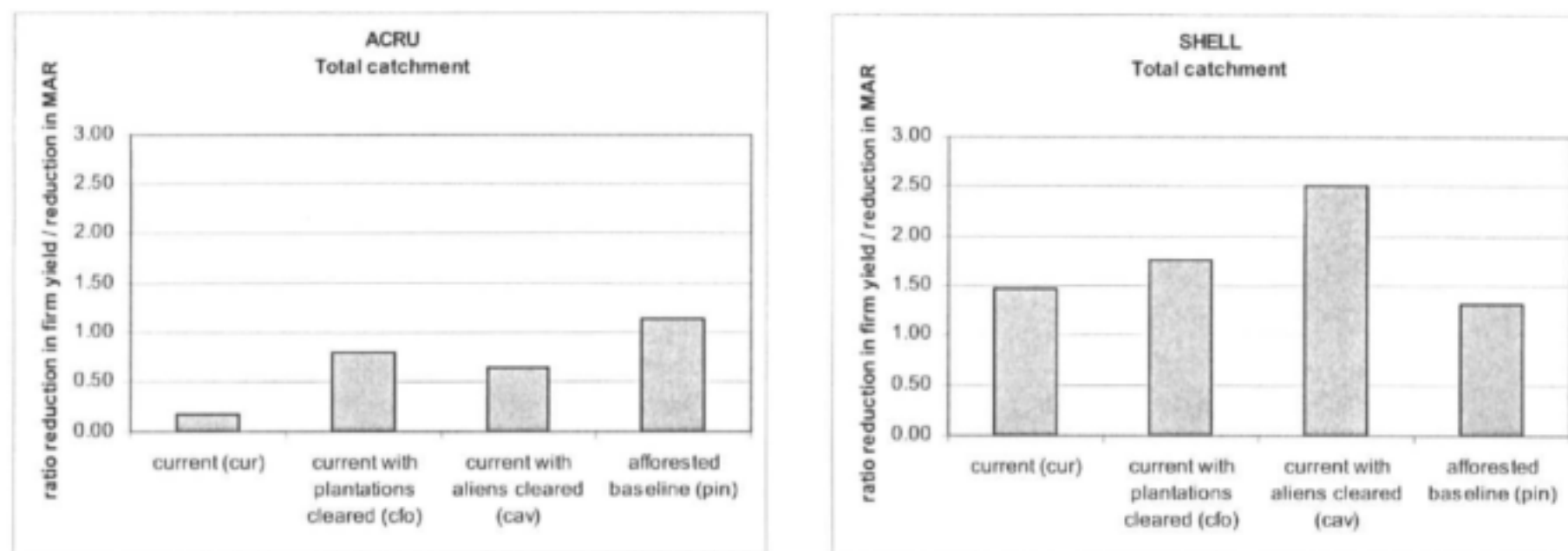
Figure 6-4: Summary of Yield Modelling Results for the Upper Berg
