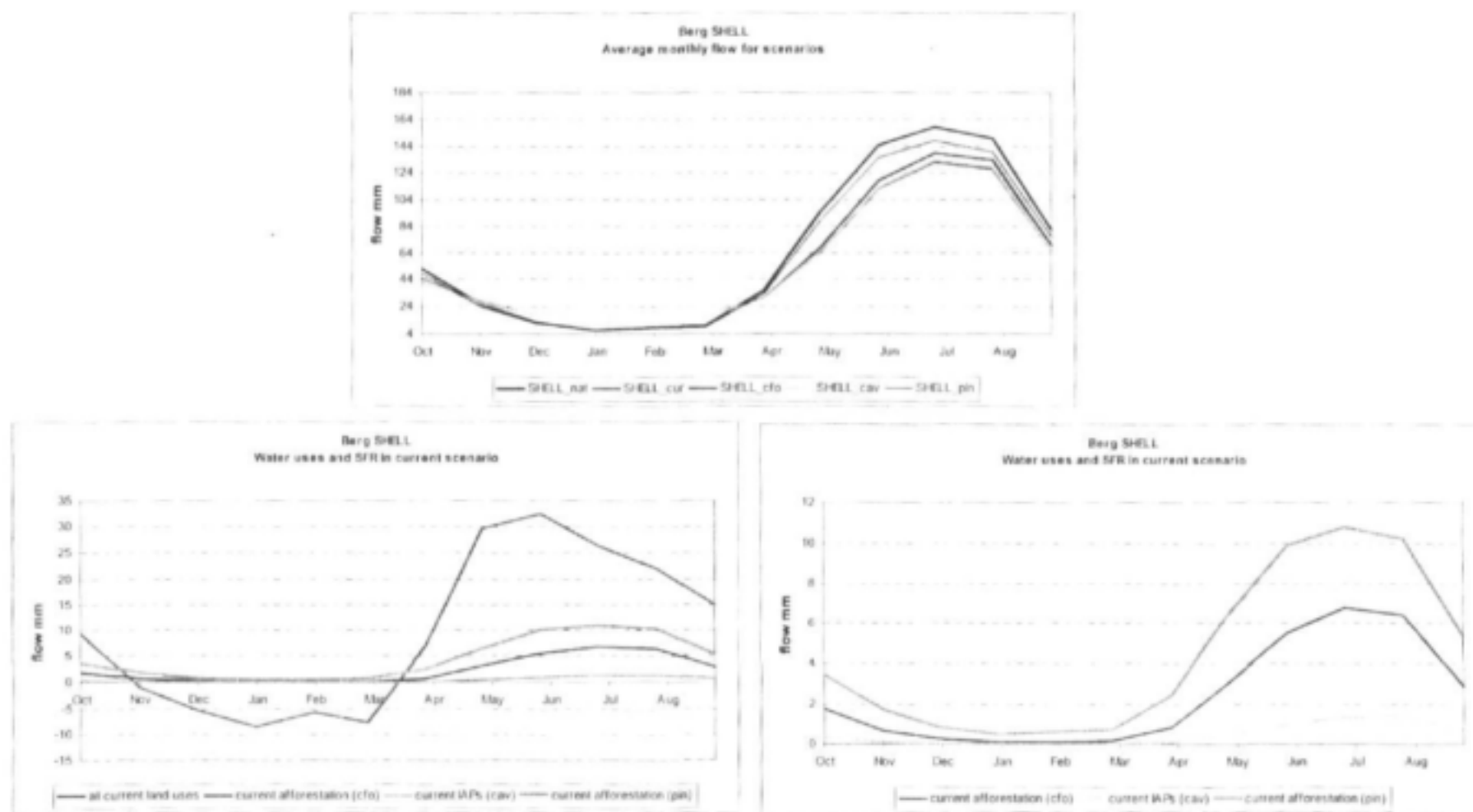
Figure 5-31: Seasonal Distribution of Flows and Reductions for Upper Berg SHELL Scenarios
