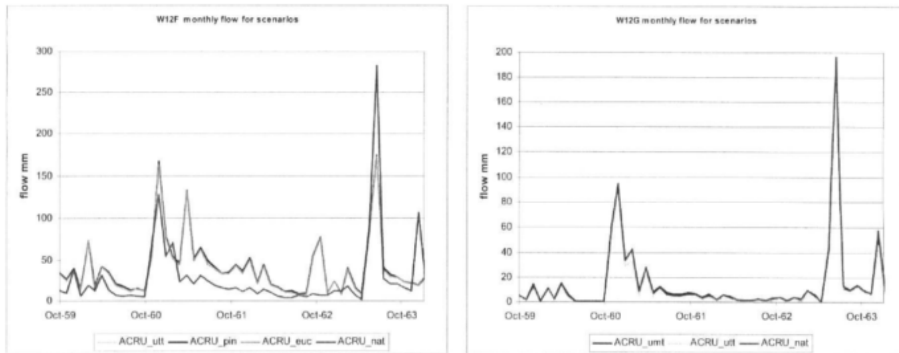
Figure 5-17: Monthly Time Series of Flow Produced by ACRU for Upland Scenarios in Subcatchments W12F and W12G in the Mhlathuze
