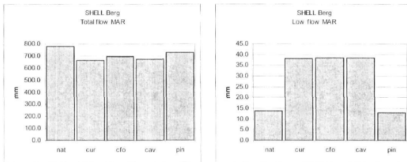
Figure 5-30: Summary of MAR Estimates Produced by SHELL for the Upper Berg
