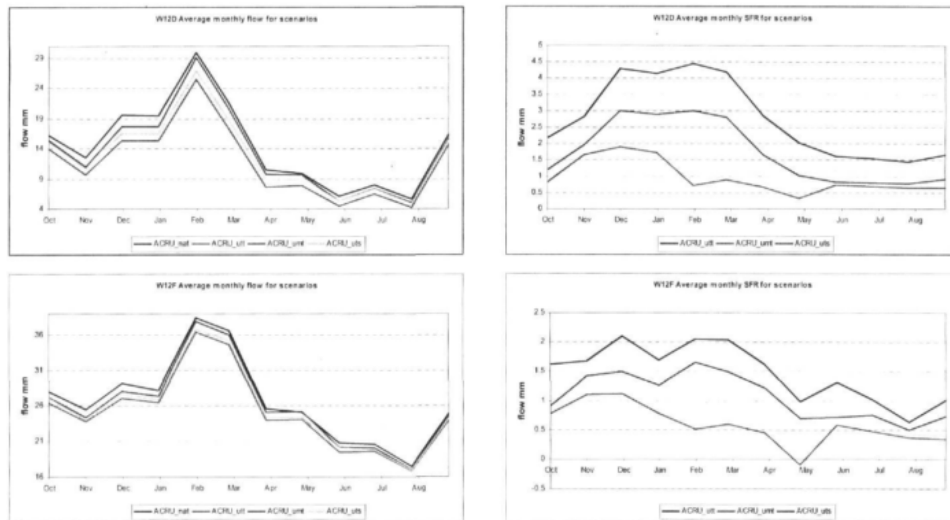
Figure 5-15 Average monthly SFR produced by ACRU for Subcatchments in the Mhlathuze for Upland Scenarios
