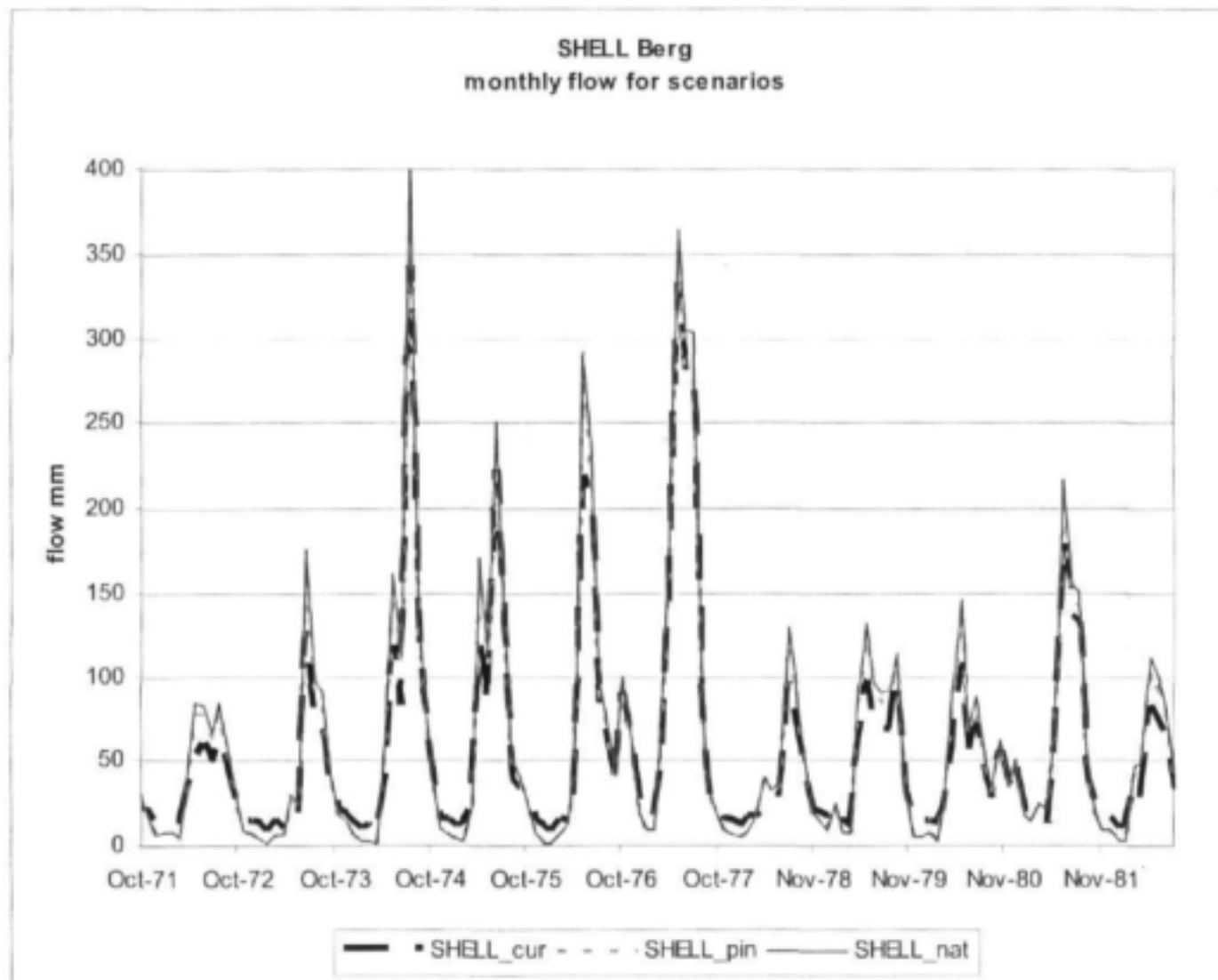
Figure 5-32: Monthly Time Series of Flows for Upper Berg SHELL Scenarios
