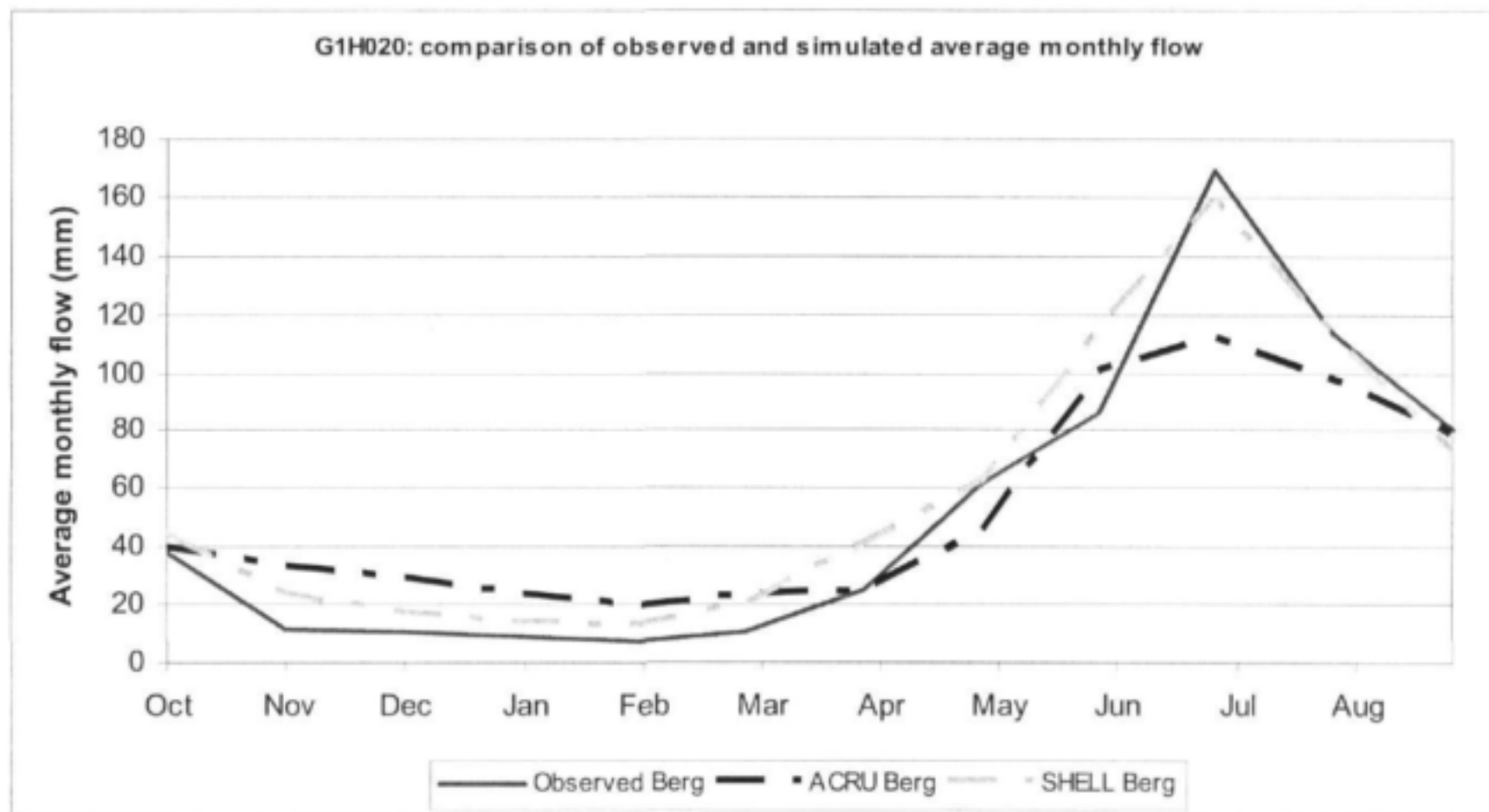
Figure 5-3: Average Monthly Plot of Observed and Simulated Flows from SHELL and ACRU at Gauge G1H020 in the Upper Berg
