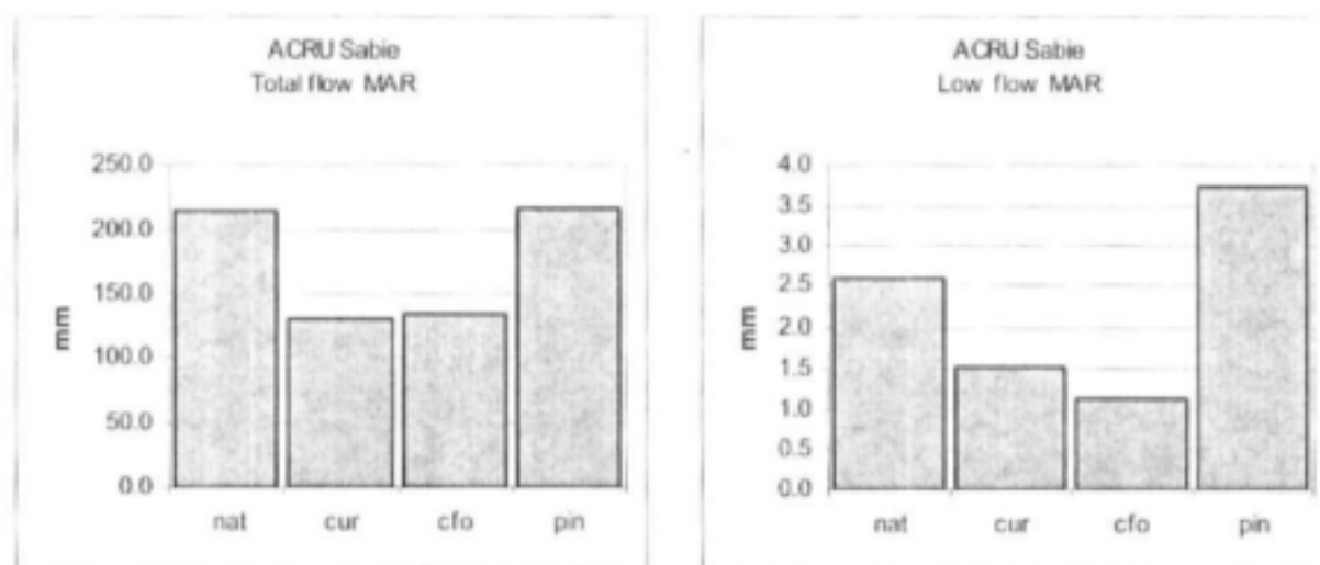
Figure 5-33: Summary of MAR Estimates Produced by SHELL for the Upper Sabie
