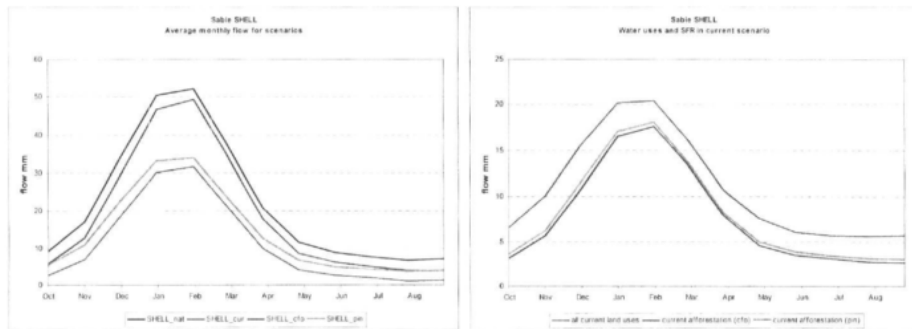
Figure 5-34: Seasonal Distribution of Flows and Reductions for Upper Sabie SHELL Scenarios
