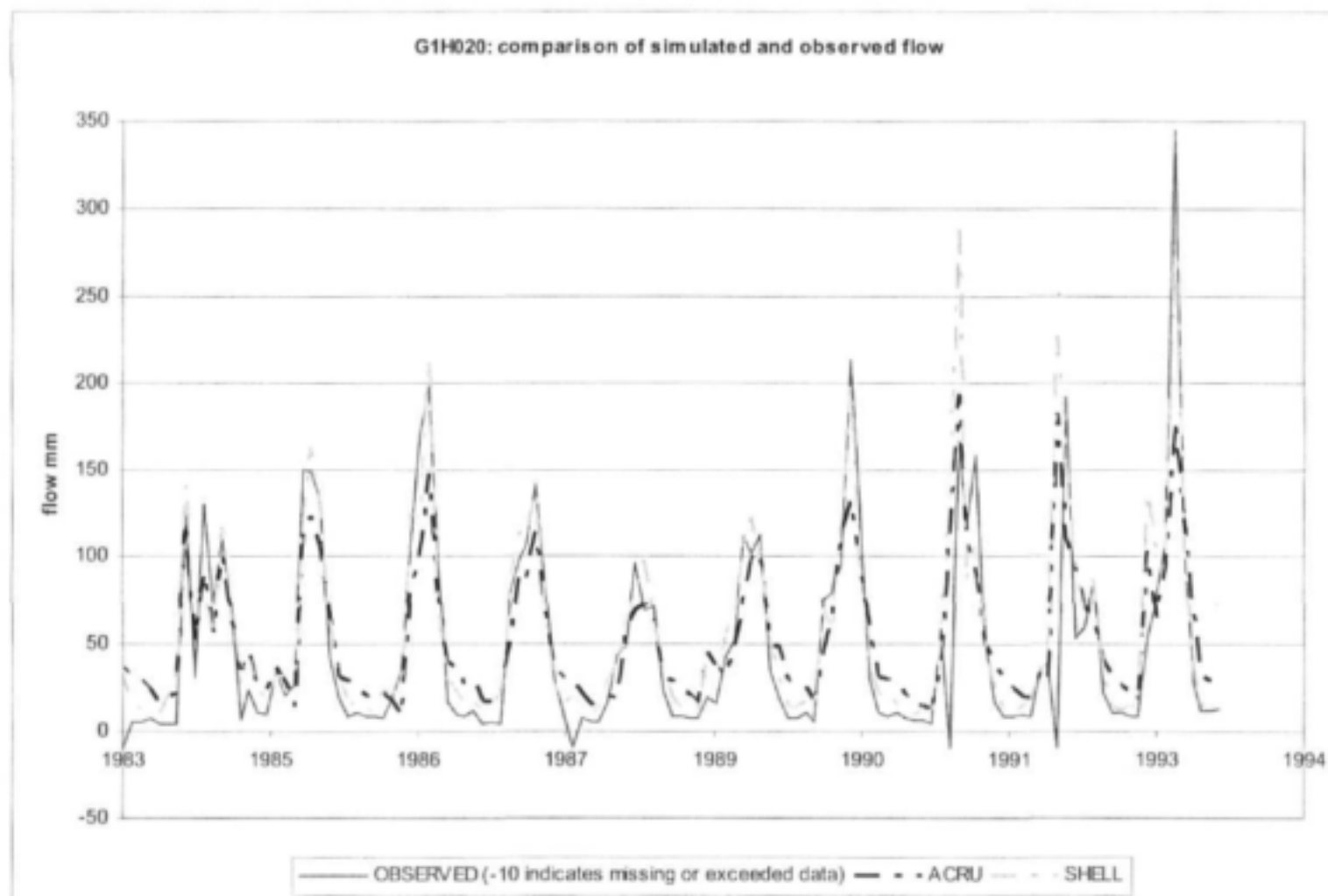
Figure 5-1: Monthly Observed and Simulated Flow for SHELL and ACRU at Gauge G1H020 in the Upper Berg
