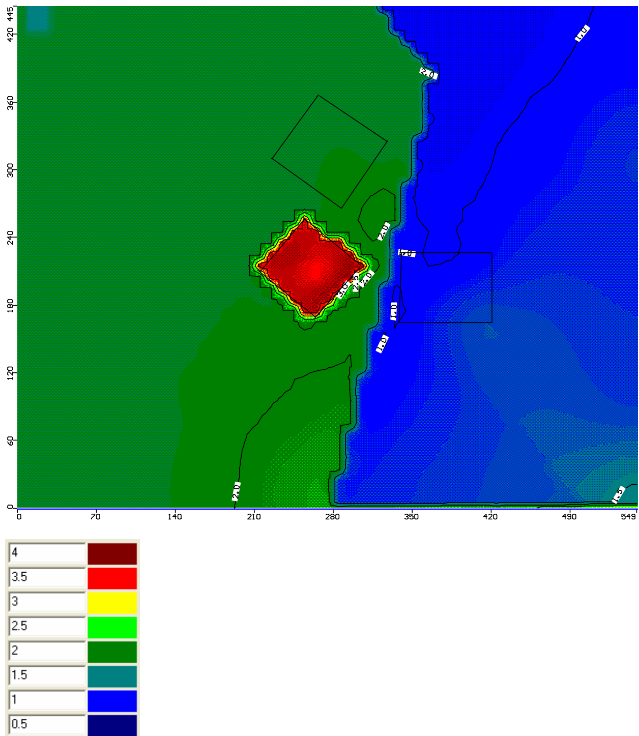
Figure 34: Spatial distribution of N concentration in groundwater in mg L -1 calculated with Visual MODFLOW.
