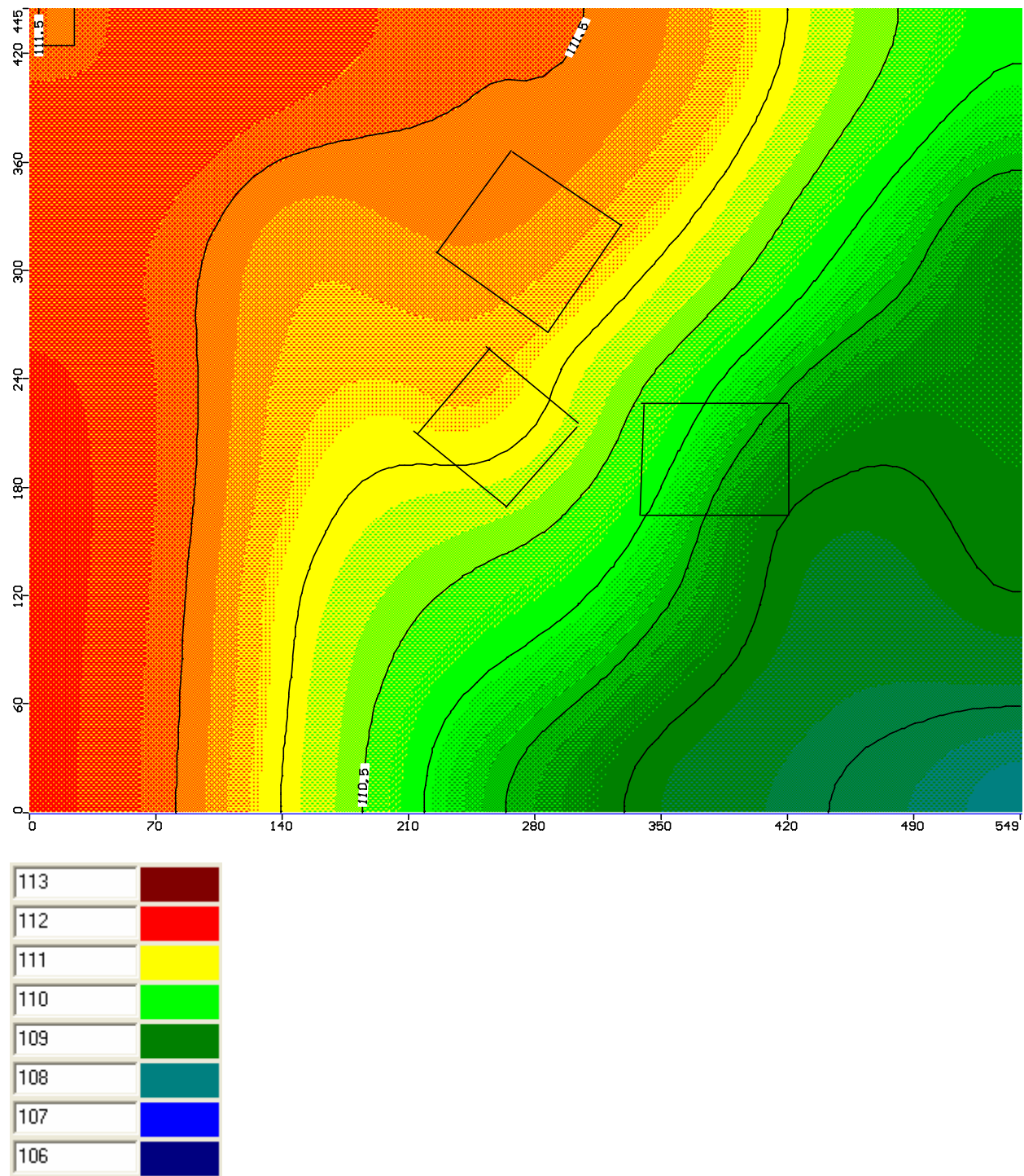
Figure 32: Spatial distribution of head equipotentials (water table elevations) in m amsl calculated with Visual MODFLOW.
