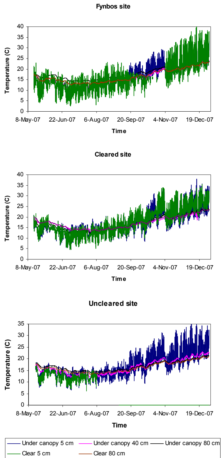
Figure 16: Soil temperatures measured with Echo-sensors at different soil depths and positions in the three treatments at Riverlands.
