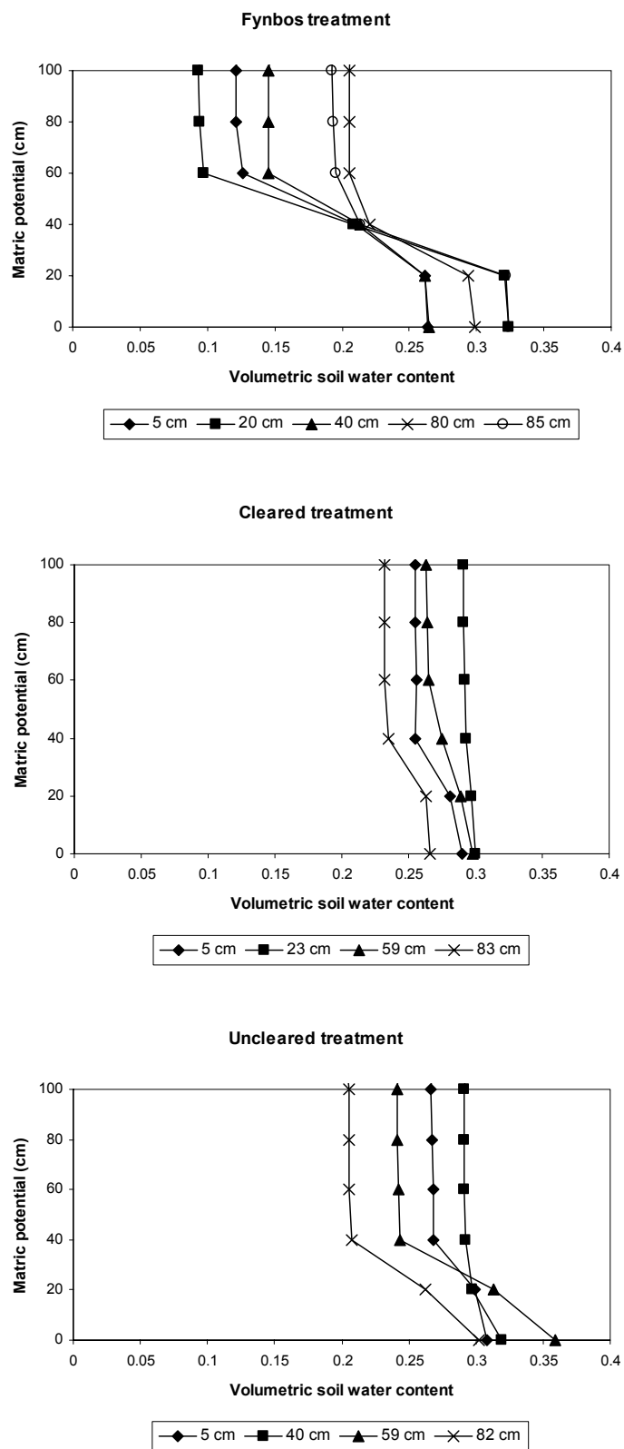
Figure 10: Soil water release curves for soil samples collected at different soil depths at Riverlands.
