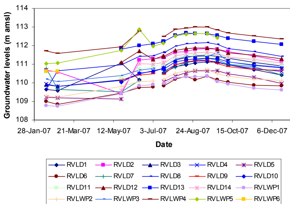
Figure 7: Groundwater levels measured manually at all boreholes in Riverlands during 2007.
