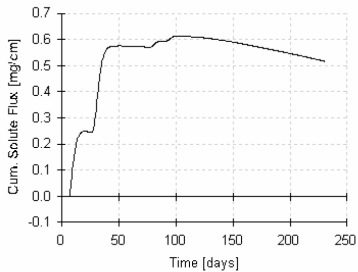
Figure 29: Simulated a) cumulative water fluxes (recharge) and b) solute fluxes (leaching) at the bottom constant pressure head boundary in the Uncleared treatment.
