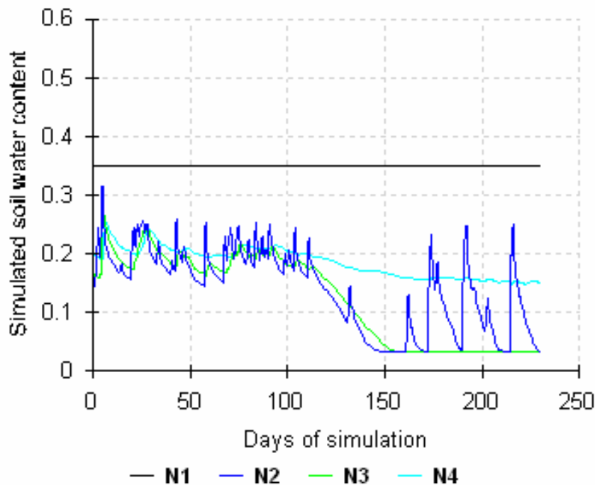
Figure 20: Simulated volumetric soil water contents in the Fynbos treatment during 2007. The observation nodes are: N1 – 150 cm; N2 – 5 cm; N3 – 40 cm; N4 – 80 cm.
