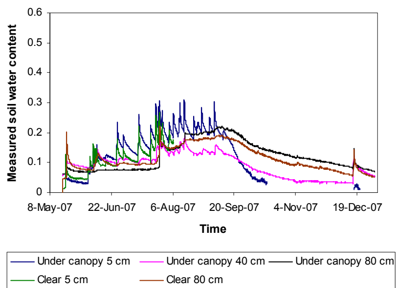
Figure 14: Volumetric soil water contents measured with Echo-sensors at different soil depths and positions in the Uncleared treatment at Riverlands.
