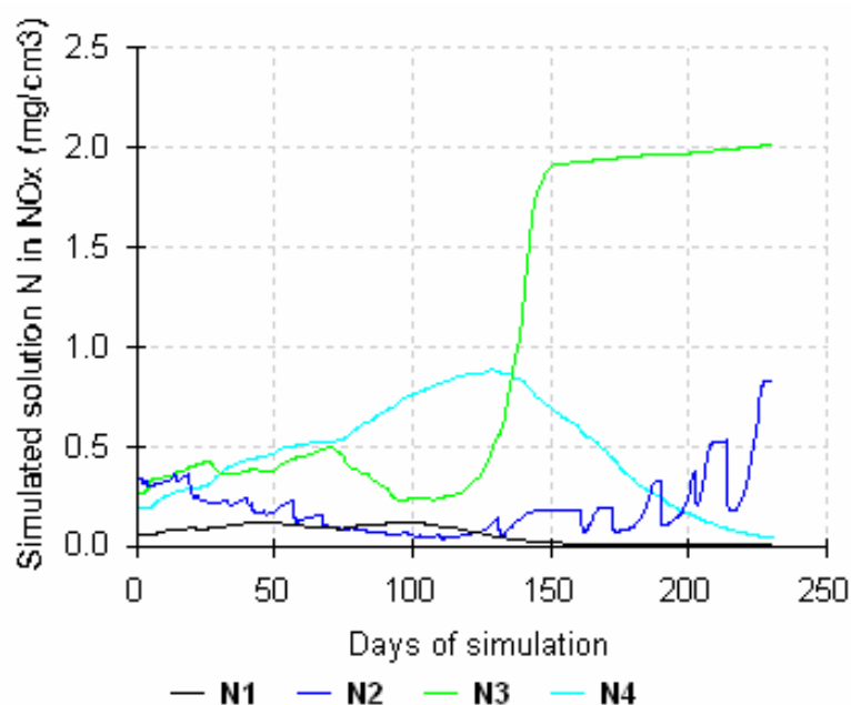
Figure 24: Simulated \text{NO}_3^- concentrations in the soil solution in the Uncleared treatment during 2007. The observation nodes are: N1 – 150 cm; N2 – 5 cm; N3 – 40 cm; N4 – 80 cm.
