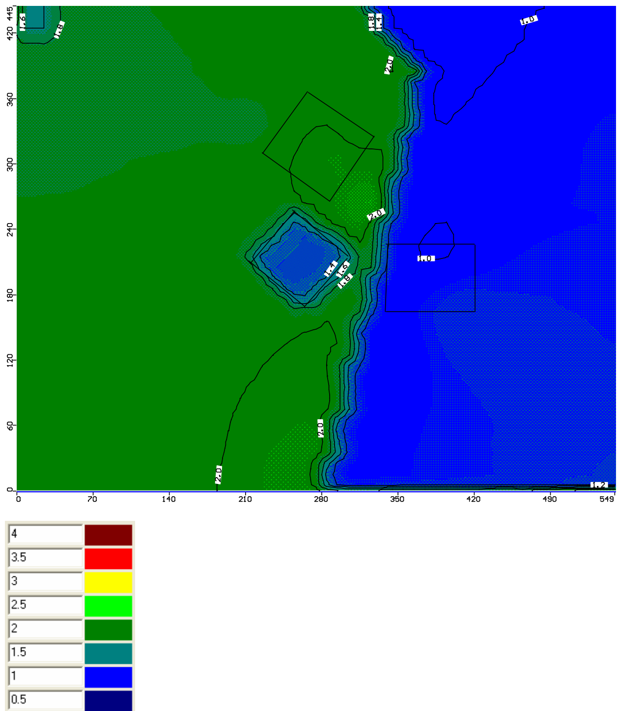
Figure 36: Spatial distribution of N concentration in groundwater in \text{mg L}^{-1} with initial N concentration in groundwater equal to 0.75 \text{ mg L}^{-1} and recharge concentration equal to 41 \text{ mg L}^{-1} in the Cleared treatment (same as for Fynbos treatment).
