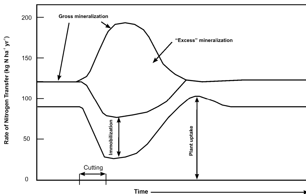
Figure 2: Hypothetical effects of clear-cutting on the internal N in deciduous forests (Vitousek, 1981).
