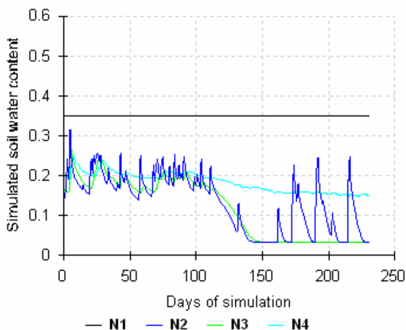
Figure 21: Simulated volumetric soil water contents in the Uncleared treatment during 2007. The observation nodes are: N1 – 150 cm; N2 – 5 cm; N3 – 40 cm; N4 – 80 cm.
