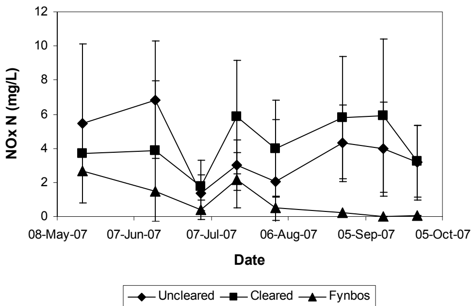
Figure 9: Nitrogen in nitrates and nitrites measured in groundwater boreholes at Riverlands during 2007.
