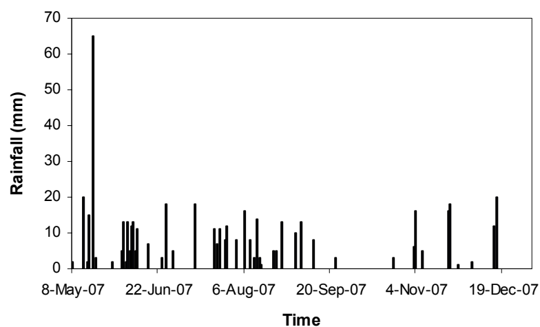
Figure 15: Rainfall data measured with manual rainmeters from May to December 2007 at Riverlands.
