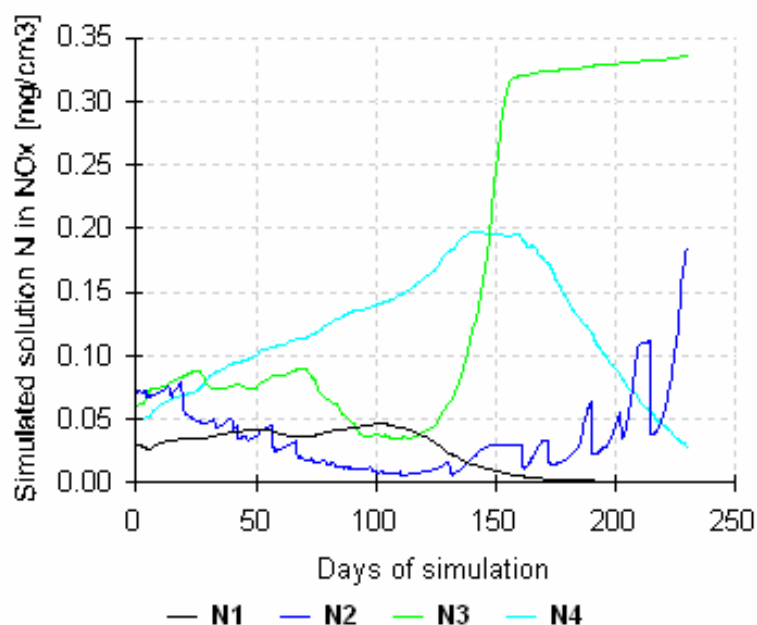
Figure 23: Simulated \text{NO}_3^- concentrations in the soil solution in the Fynbos treatment during 2007. The observation nodes are: N1 – 150 cm; N2 – 5 cm; N3 – 40 cm; N4 – 80 cm.
