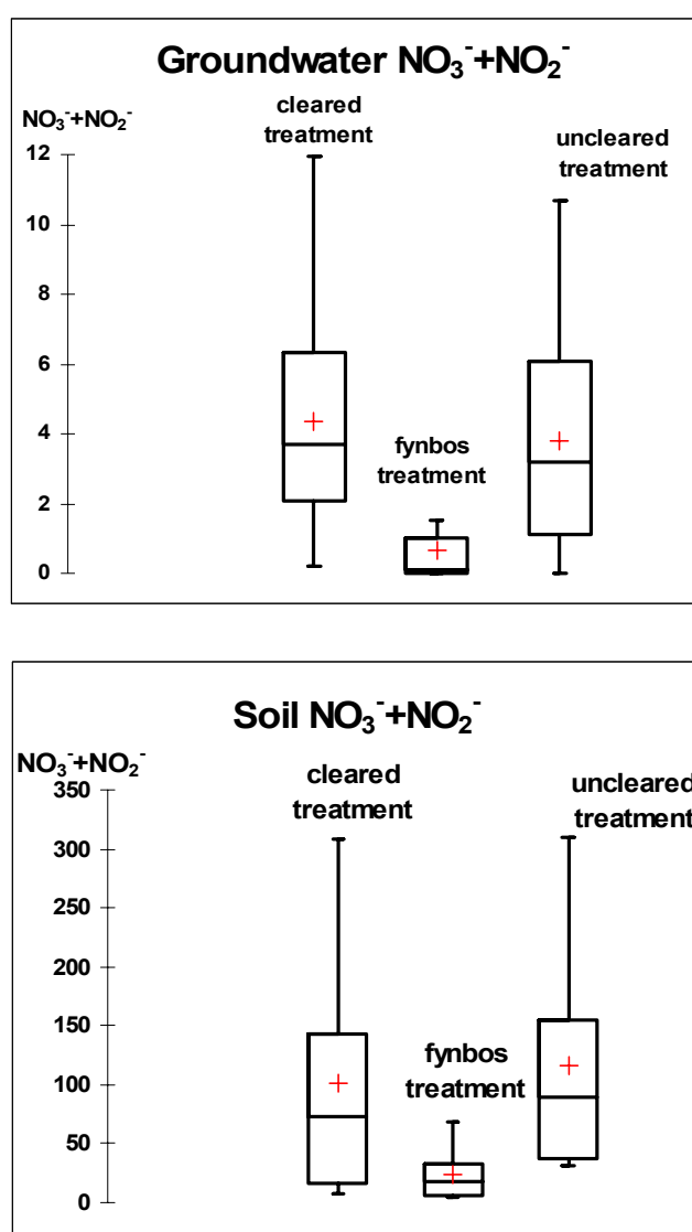
Figure 18: Descriptive statistical analysis of groundwater and soil nitrogen data (units are in \text{mg L}^{-1} ), showing maximum, minimum, 1 st and 3 rd quartiles, median and average (cross) values. The number of observations was 16 for the Fynbos treatment and 32 for the Cleared and Uncleared treatments.
