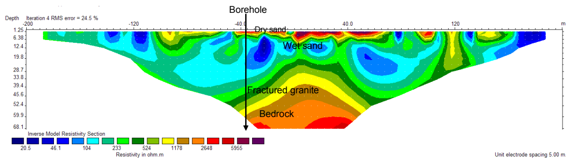
Figure 4: Deep resistivity survey profile next to the existing 120 m deep borehole.
