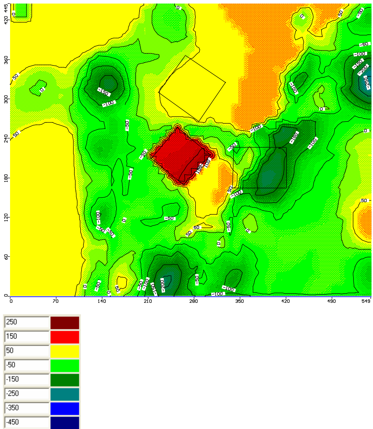
Figure 33: Spatial distribution of net recharge (recharge minus evapotranspiration) in mm calculated with Visual MODFLOW.
