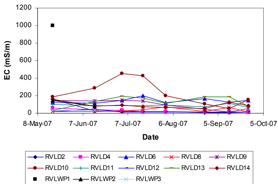
Figure 8: Electrical conductivity (EC) in groundwater measured during 2007.
