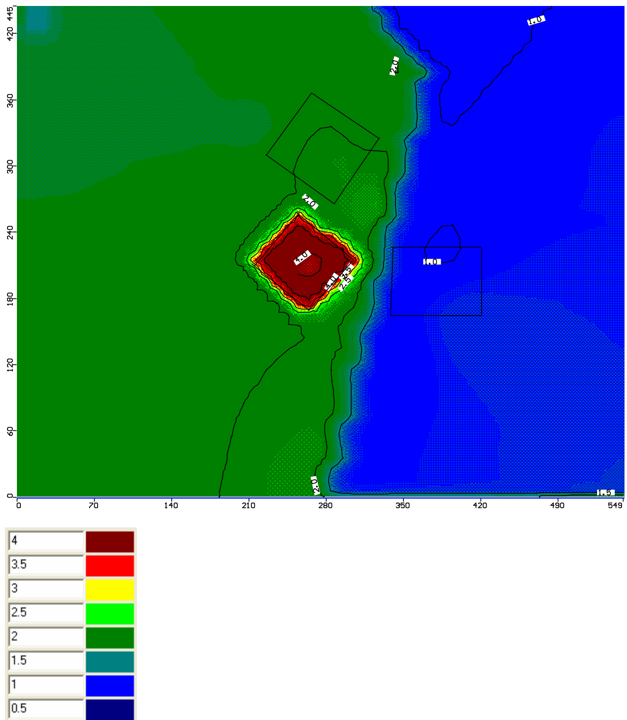
Figure 35: Spatial distribution of N concentration in groundwater in \text{mg L}^{-1} with saturated hydraulic conductivity equal to 0.000133 \text{ m s}^{-1} ( 11.46 \text{ m d}^{-1} ) calculated with Visual MODFLOW.
