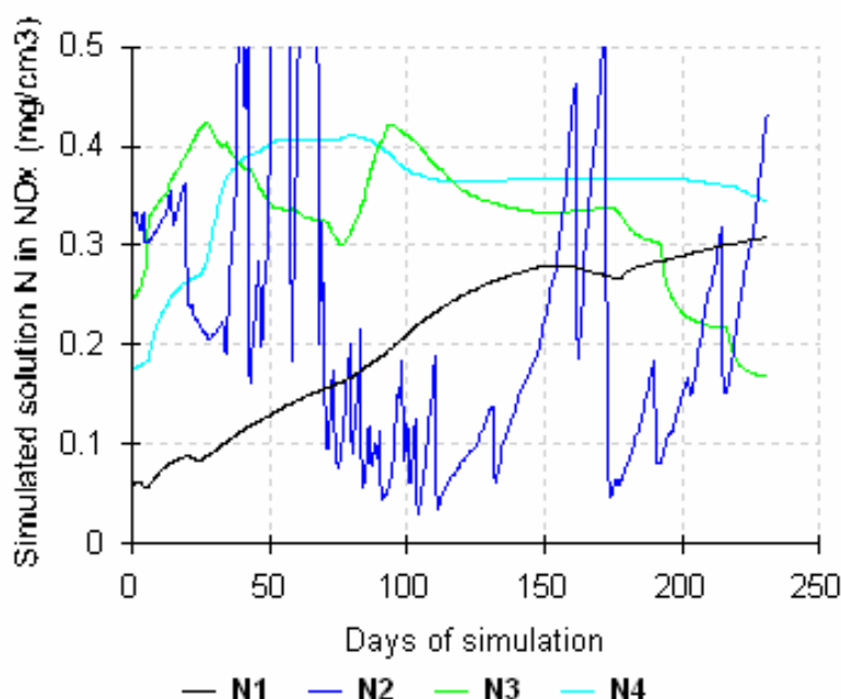
Figure 25: Simulated \text{NO}_3^- concentrations in the soil solution in the Cleared treatment during 2007. The observation nodes are: N1 – 150 cm; N2 – 5 cm; N3 – 40 cm; N4 – 80 cm.
