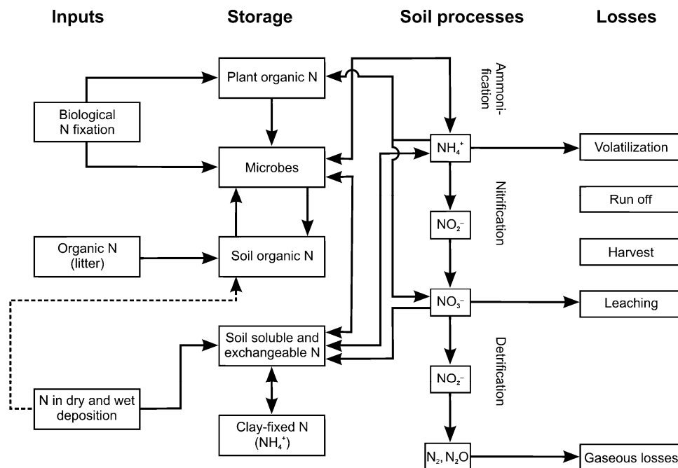
Figure 1: Interactions of N processes in soils (adapted from Rosswall, 1976).
