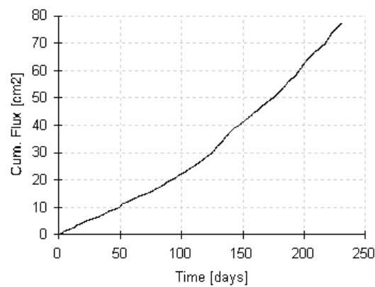
Figure 26: Simulated a) cumulative water fluxes at the atmospheric boundary, b) potential evapotranspiration and c) actual evapotranspiration of the Fynbos treatment.
