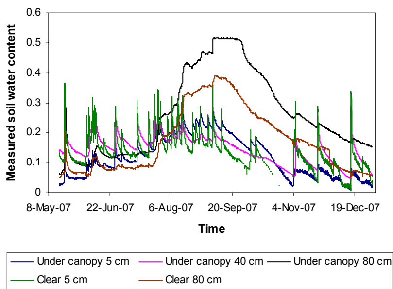
Figure 12: Volumetric soil water contents measured with Echo-sensors at different soil depths and positions in the Fynbos treatment at Riverlands.
