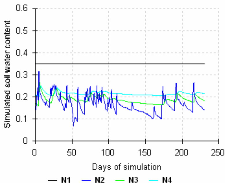
Figure 22: Simulated volumetric soil water contents in the Cleared treatment during 2007. The observation nodes are: N1 – 150 cm; N2 – 5 cm; N3 – 40 cm; N4 – 80 cm.
