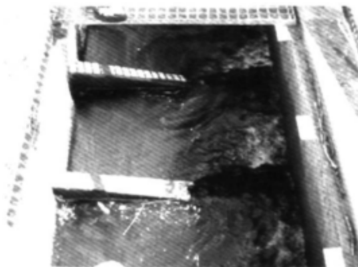
Plate 7.4: Grating removed to show pools and baffles inside Nhlabane Fishway.
