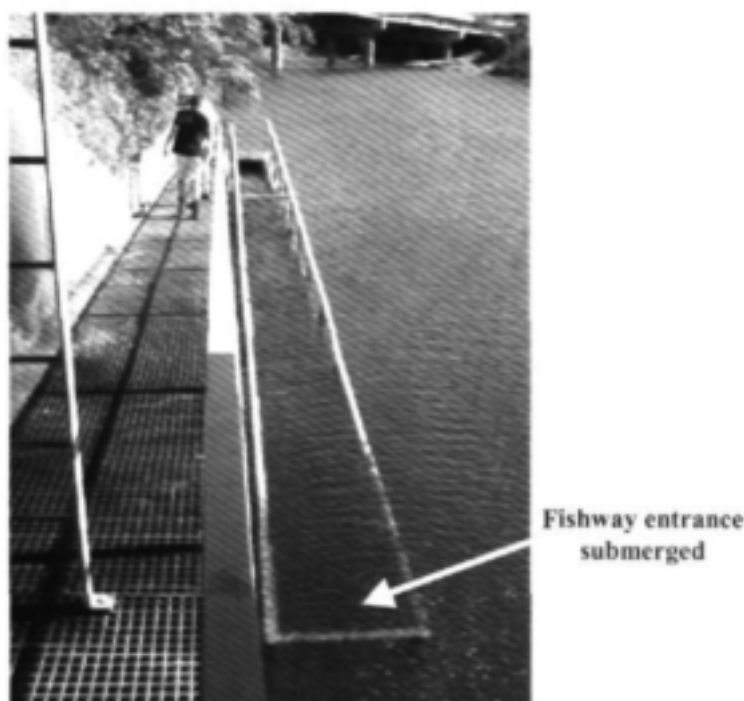
Plate 7.2: Fishway entrance as seen from the weir.
