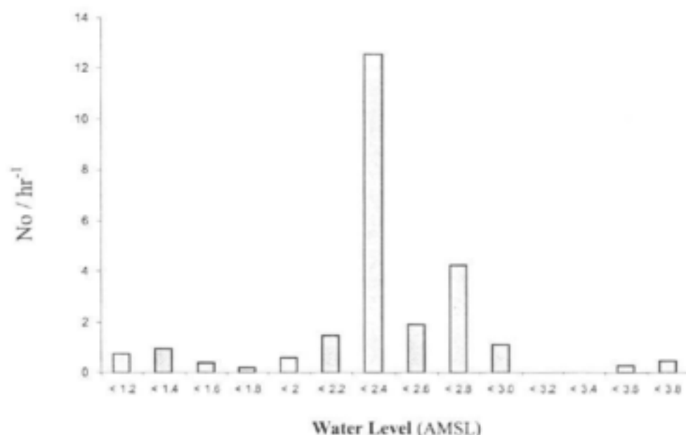
Figure 7.4: Number of fish recorded migrating upstream per hour through the Nhlabane fishway at estuary water levels of 1.0 - 1.2 ( n = 80 h), 1.21 - 1.4 ( n = 27 h), 1.41 - 1.6 ( n = 38 h), 1.61 - 1.8 ( n = 14 h), 1.81 - 2.0 ( n = 12 h), 2.01 - 2.2 ( n = 103 h), 2.21 - 2.4 ( n = 57 h), 2.41 - 2.6 ( n = 123 h), 2.61 - 2.8 ( n = 108 h), 2.81 - 3.0 ( n = 216 h), 3.01 - 3.2 ( n = 3 h), 3.21 - 3.4 ( n = 0 h), 3.41 - 3.6 ( n = 100 h) and 3.61 - 3.8 ( n = 48 h) m AMSL during the sampling period from January –December 2001 and October 2002 - September 2003.
