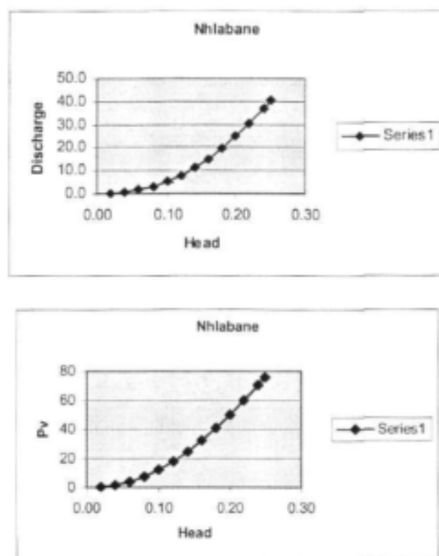
Figure 2: Nhlabane fishway: Discharge and Power as function of Head
