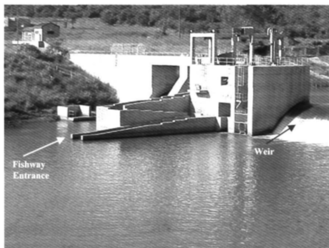
Plate 8.1: A view of the three sections of the Xikundu fishway
