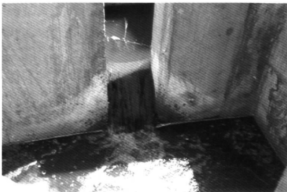
Plate 3.5: Close-up of “Pool and Slot” baffle at Riverside Weir fishway in the KNP under low flow conditions.
