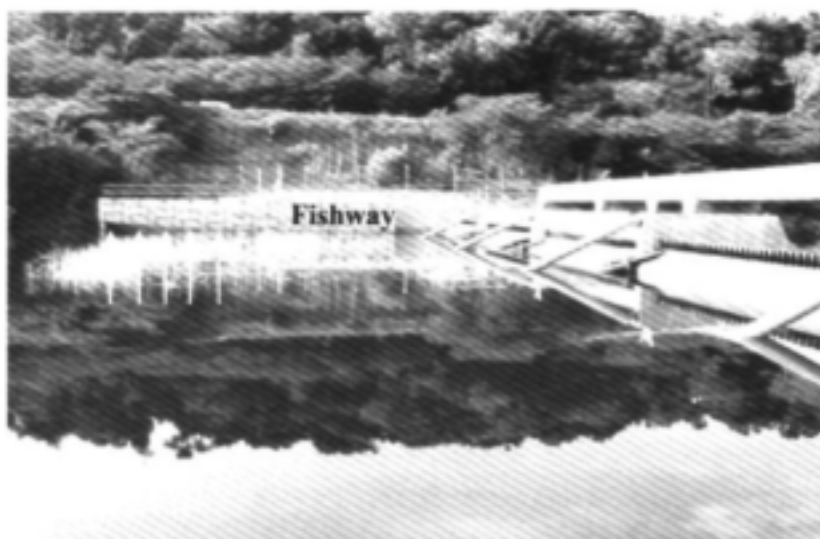
Plate 7.3: Upstream view of Nhlabane weir and fishway exit during low lake level. Arrows indicate positions of exposed exit ports/inlet sluices.
