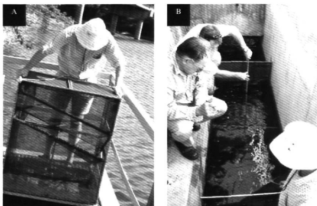
Plate 7.5: Funnel trap (A) and block nets (B) in pool 82 in fishway showing position of block nets and use of scoop net to clear trap.
