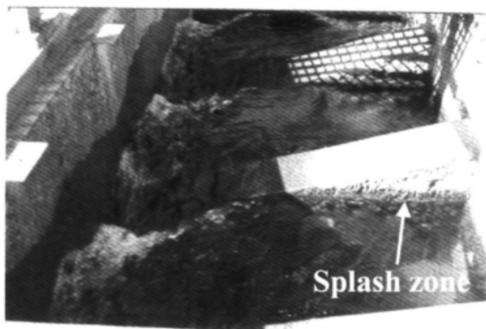
Plate 3.3: Water flow over the weir of the Nhlabane Pool and Weir fishway, showing the sloping weir with variable passage depth and wetted “splash-zone” for eels and macroinvertebrates.
