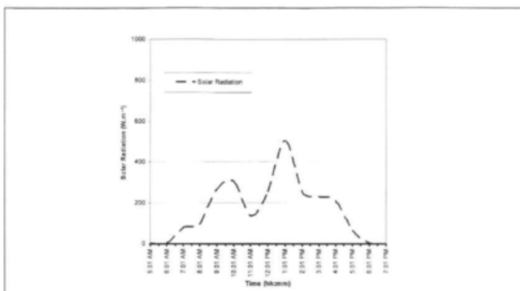
Figure 4.9: Hourly solar-radiation data ( \text{W/m}^2 ) from the 22 nd March 2005 at OSCA.
