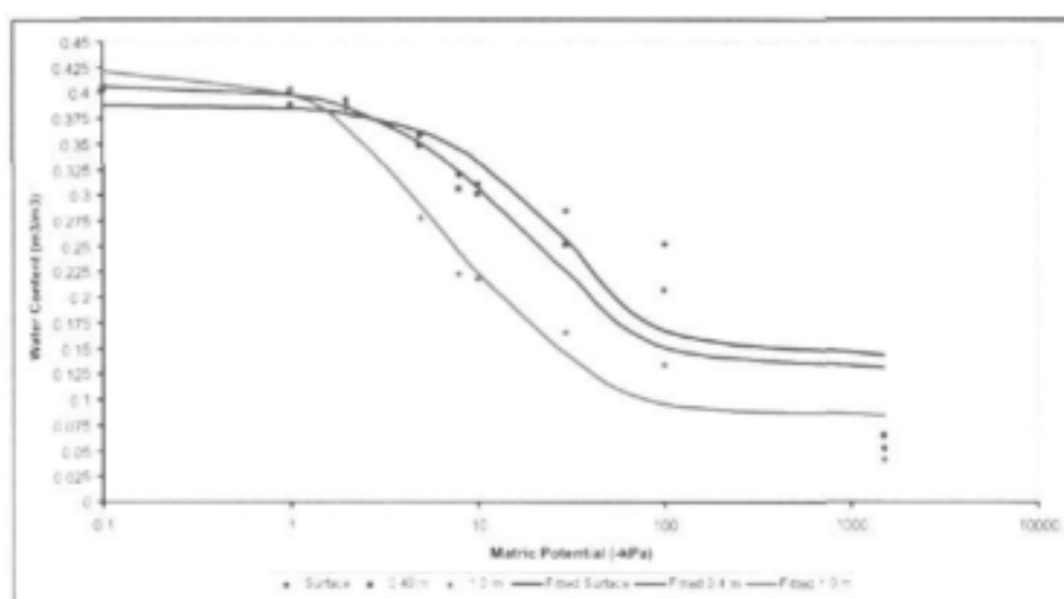
Figure 4.18: Water-retention curve for the soils at the OSCA site
