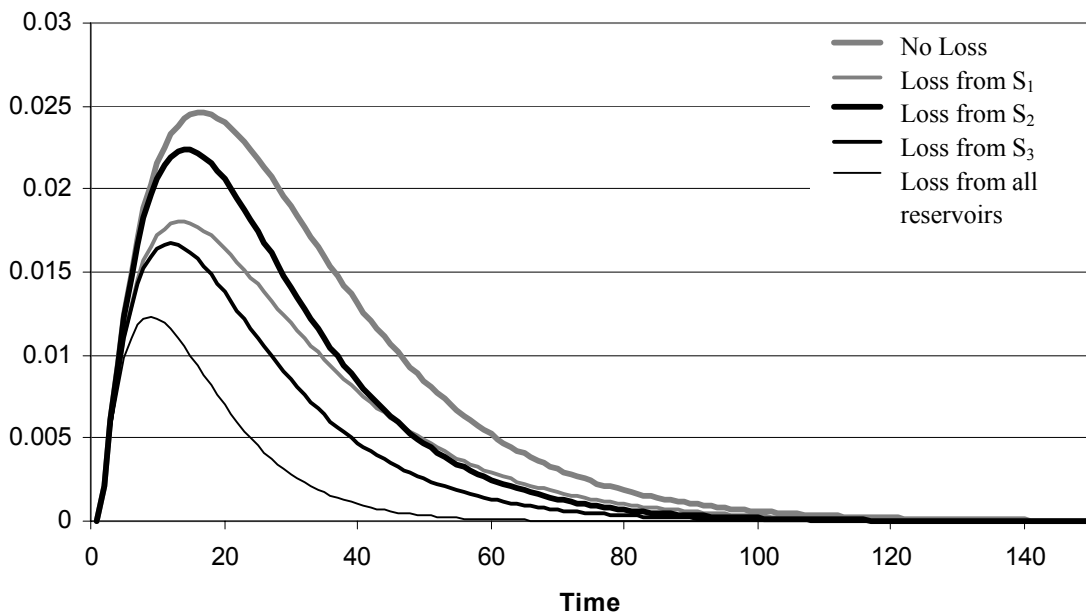
Figure A.5: Comparison of some pulse response functions for the 3 reservoir model
