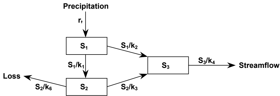
Figure 3.9: Schematic of a 3 linear reservoir feed forward linear catchment model
