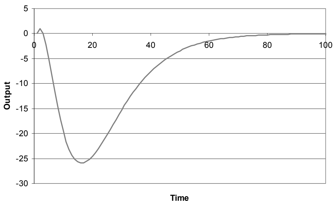
Figure A.3: A negative response from a three reservoir arrangement
