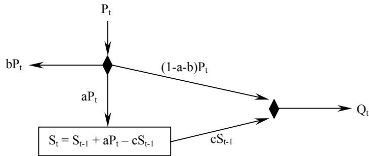
Figure 1.2 : Schematic of the abc model
