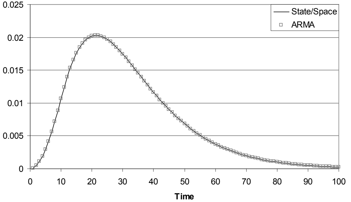
Figure A.2: Comparisons of a pulse response function for the State-Space and pseudo-ARMA representations of the 3 linear reservoir model
