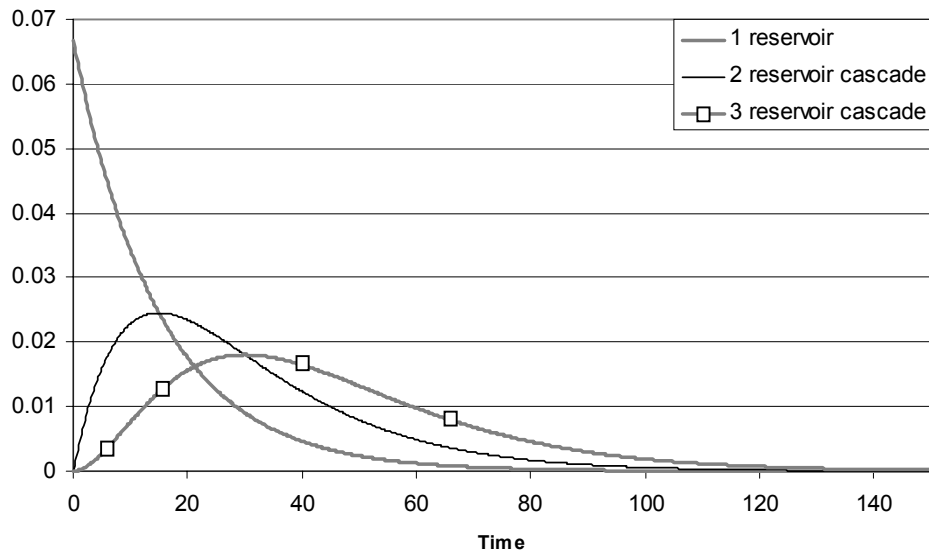
Figure 2.3: Impulse response functions for a single reservoir and cascades of equal reservoirs (with k = 15 time periods).
