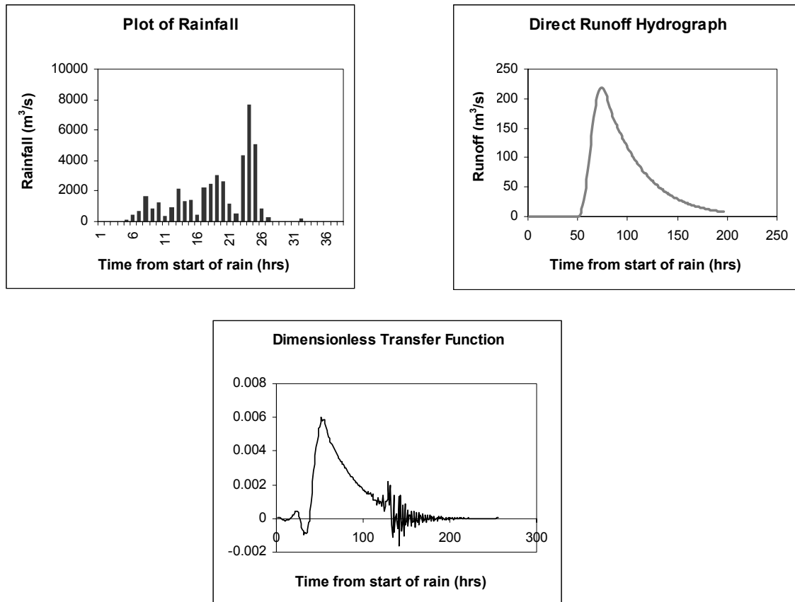
Figure 2.2: Transfer Function found making use of Fast Fourier Transforms
