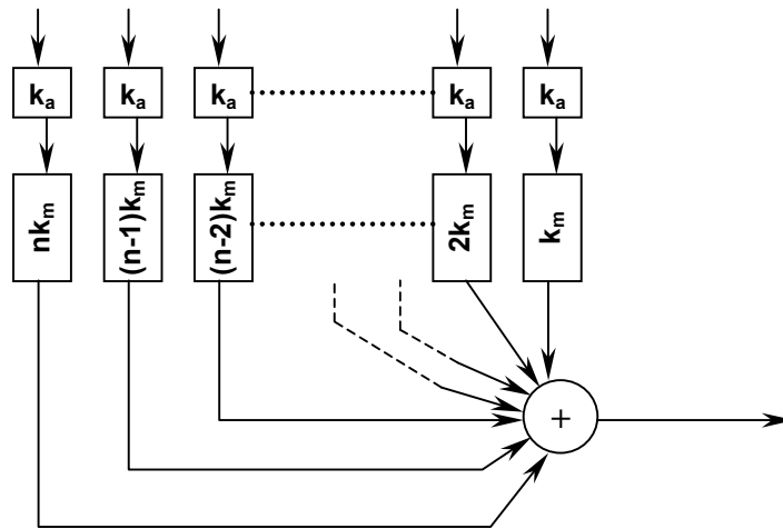
Figure 2.6: The Manifold cell model (Pegram & Diskin, 1987a)
