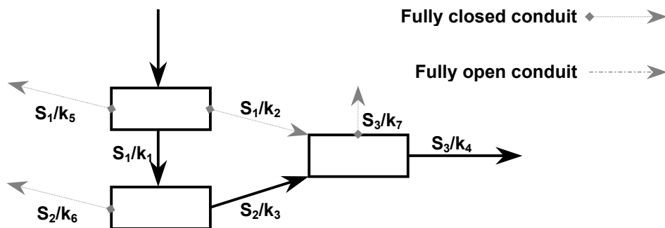
Figure 4.6: A “three reservoir cascade” configuration of the model
