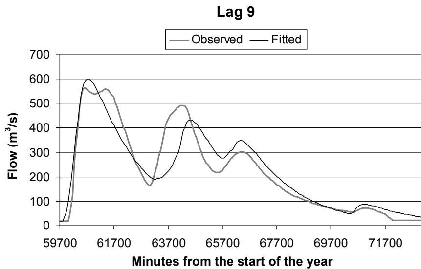
Figure 4.21: Observed and fitted streamflow for February 1996 (single cell, single parameter set for the entire event)
