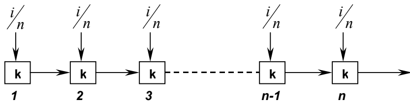
Figure 2.5: The Distributed input cascade (Dooge, 1959)
