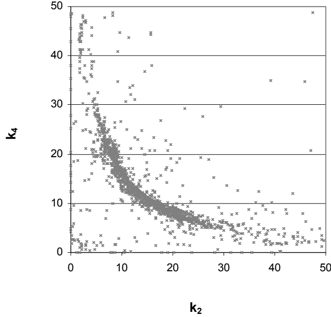
Figure 4.12: Example scatter plot showing a clustering of points near the optimum
