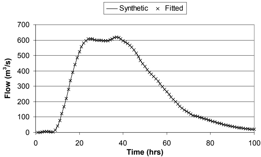
Figure 4.11: Streamflow responses for the full 3 reservoir model
