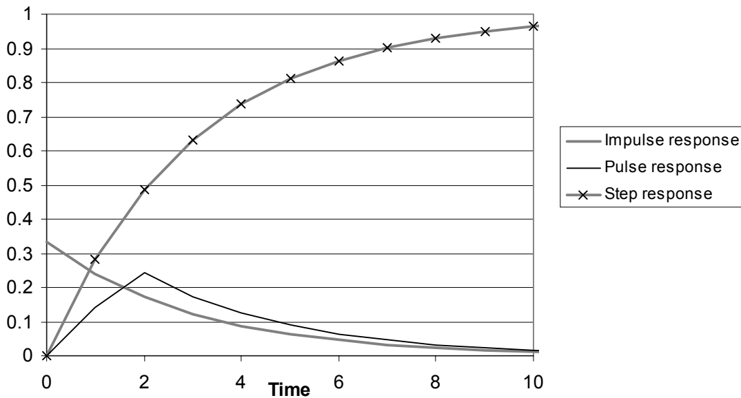
Figure 2.1 : Response functions for a linear reservoir (after Chow et al., 1988)
