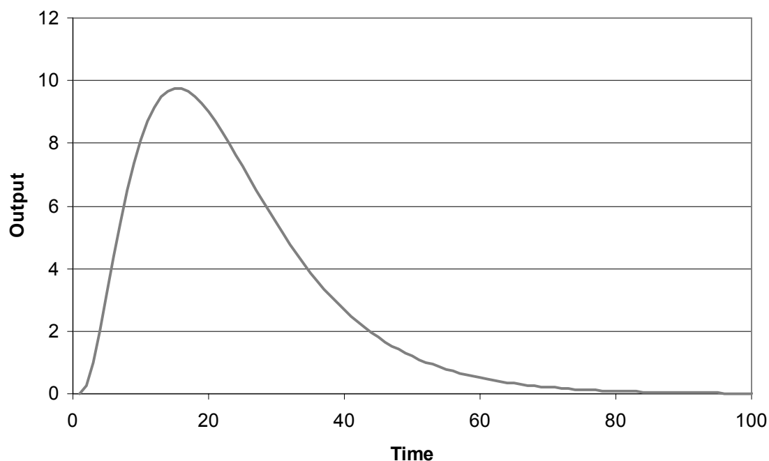
Figure A.4: A non-negative response from a three reservoir arrangement
