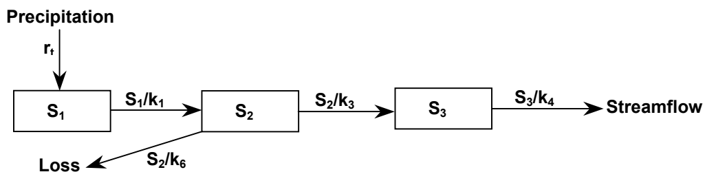
Figure 4.34: A 3 reservoir cascade with loss from the second reservoir.
