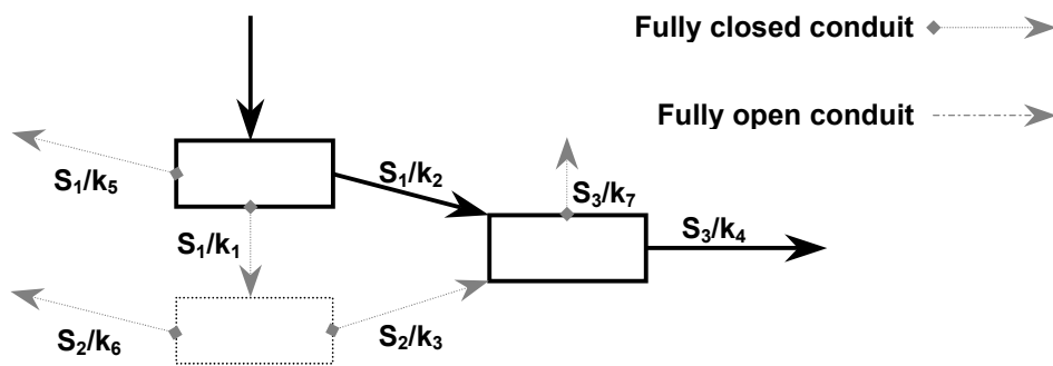
Figure 4.5: A “two reservoir cascade” configuration of the model
