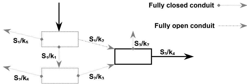
Figure 4.1: Schematic of “single reservoir” model configuration
