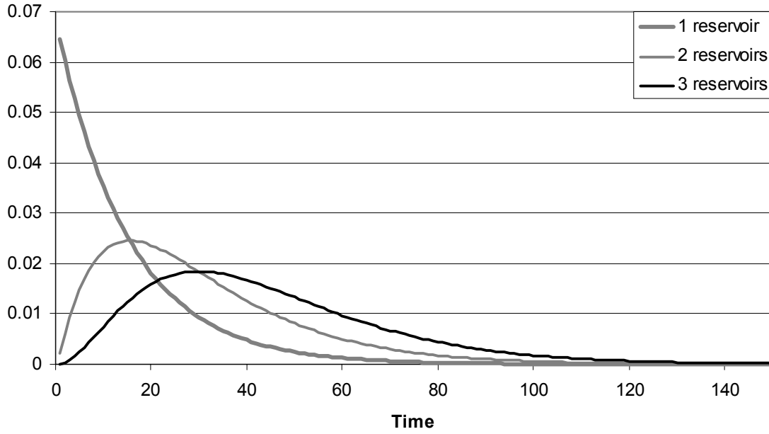
Figure A.8: Impulse response functions for the 3 linear reservoir model reduced to 1, 2 & 3 reservoir cascades
