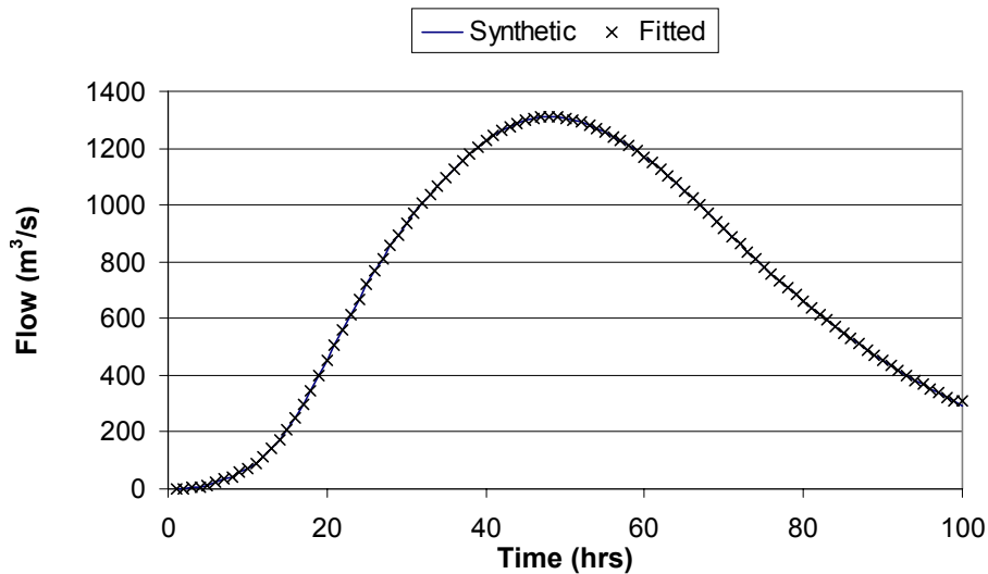
Figure 4.8: Streamflow responses for a “3 reservoir cascade”
