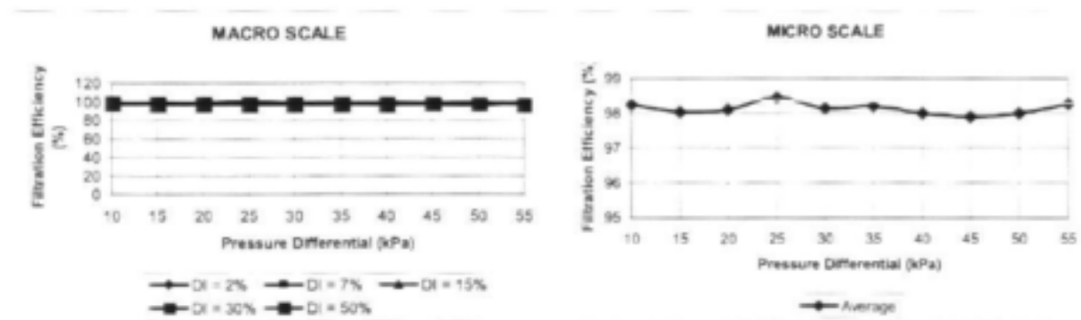
Fig. 4.13: Filtration efficiency of sand filters AS and DS
