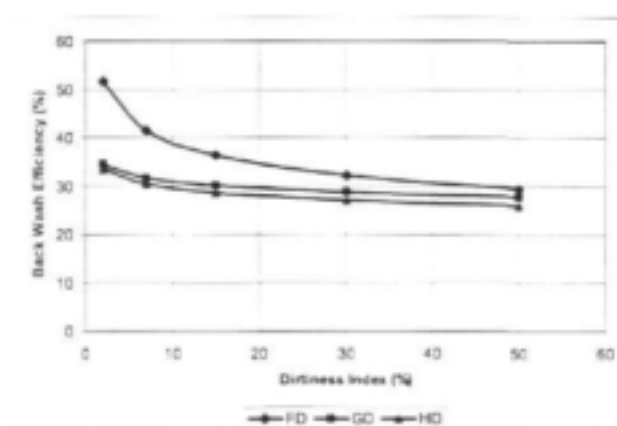
Fig. 4.9: The backwash efficiencies of the three different filter discs
