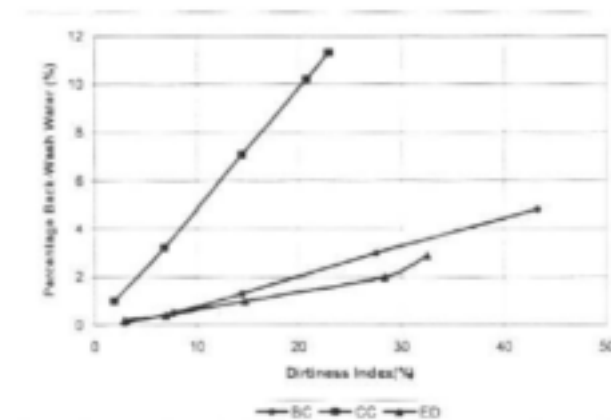
Fig. 4.16: Backwash water percentages test results for the automatic filters
