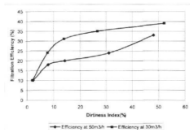
Fig. 4.17: The effect of flow-rate on filtration efficiency
