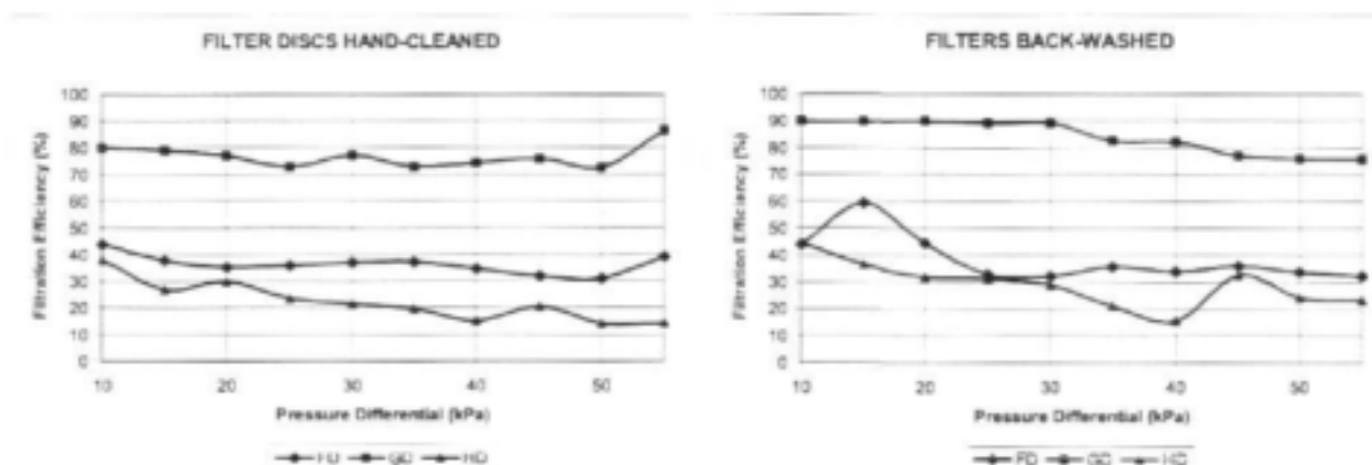
Fig. 4.8: The filtration efficiencies of the three different filter discs
