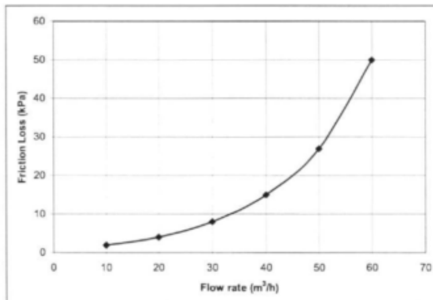
Fig. 6.3: Friction loss graph of the Silicon II sand filter
