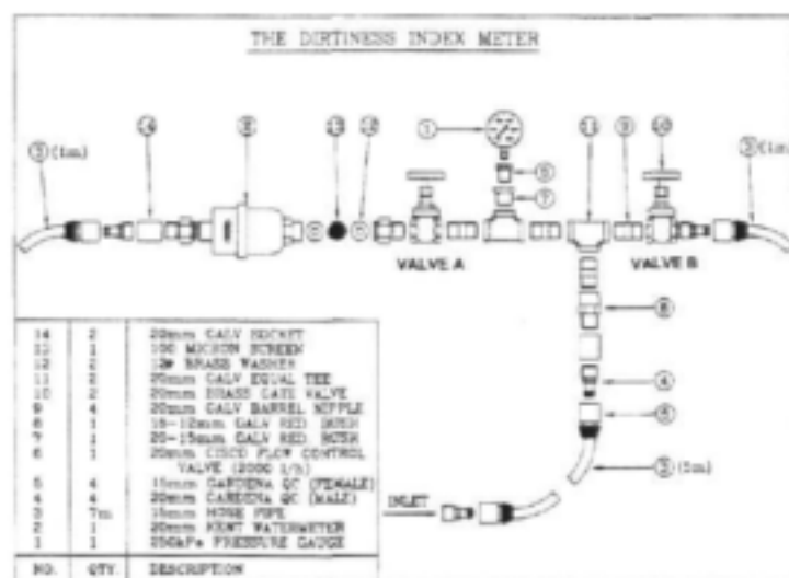
Diag. 3.1: Components of the Dirtiness Index Meter
