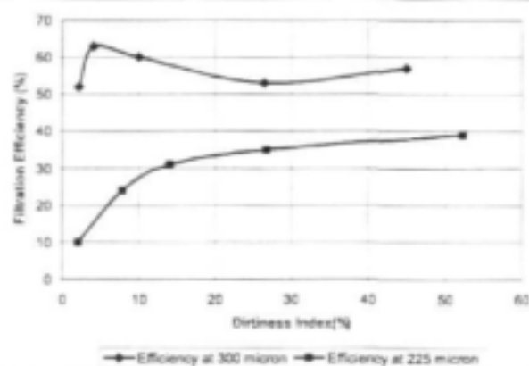
Fig. 4.18: Effect of different ratings of the fineness of a filter's element on its filtration efficiency
