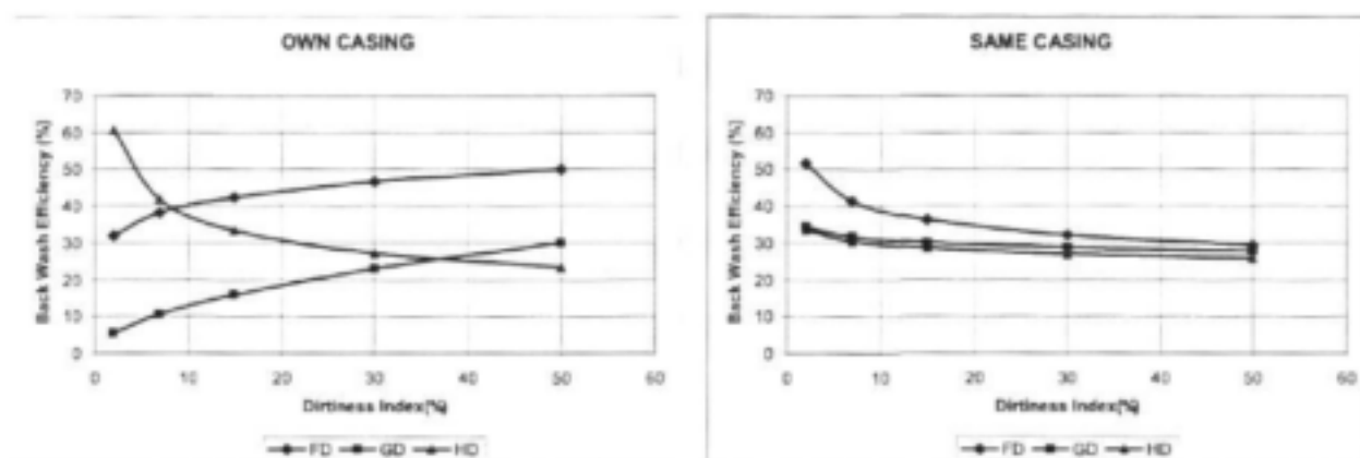
Fig. 4.12: Backwash efficiencies for three different filter discs in their own and same casing
