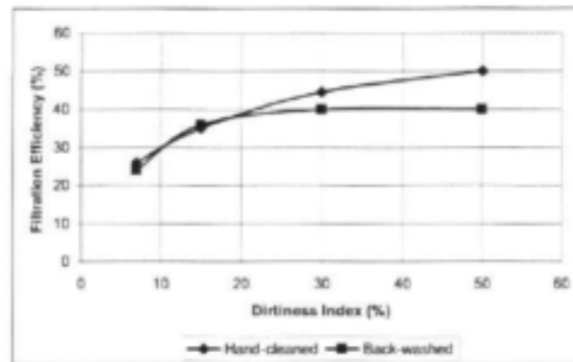
Fig. 4.6: Filtration efficiency as a function of the dirtiness of the water
