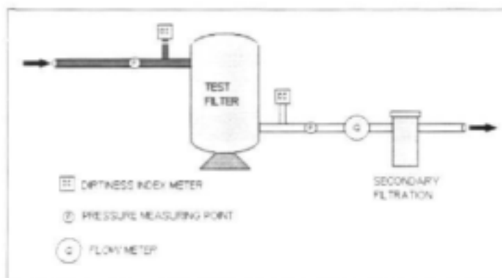
Diag. 3.2: Schematic set-up of filter test
