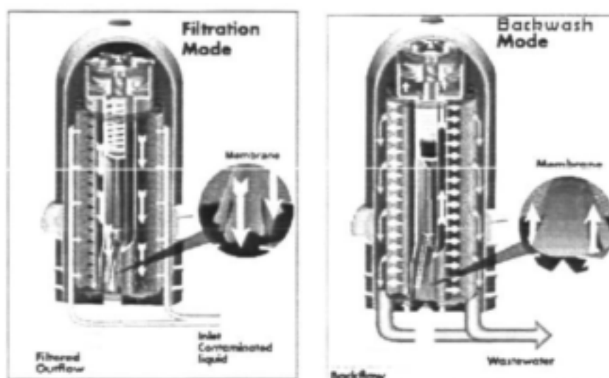
Fig. 2.2: Operating principles of automatic disc filters during the filtration and backwashing mode (Arkal, 2002)
