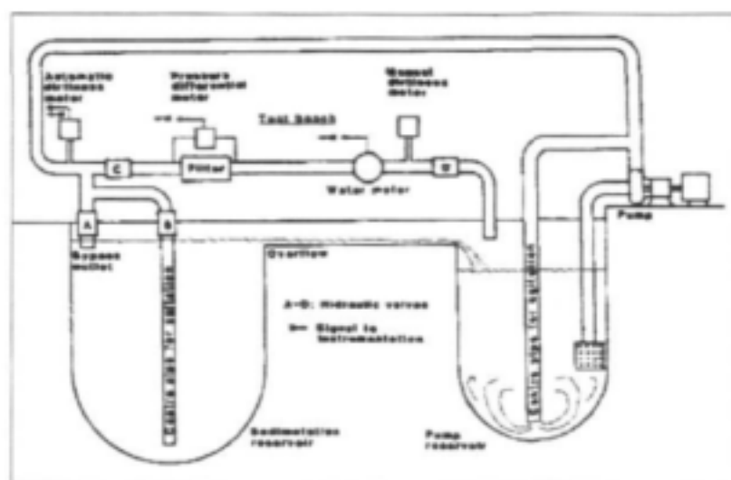
Diag. 3.3: The irrigation filter test bench of the ILI Hydrolabs (Van Niekerk, 1983)
