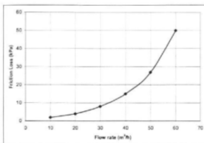
Fig. 3.2: A typical friction loss curve of a filter
