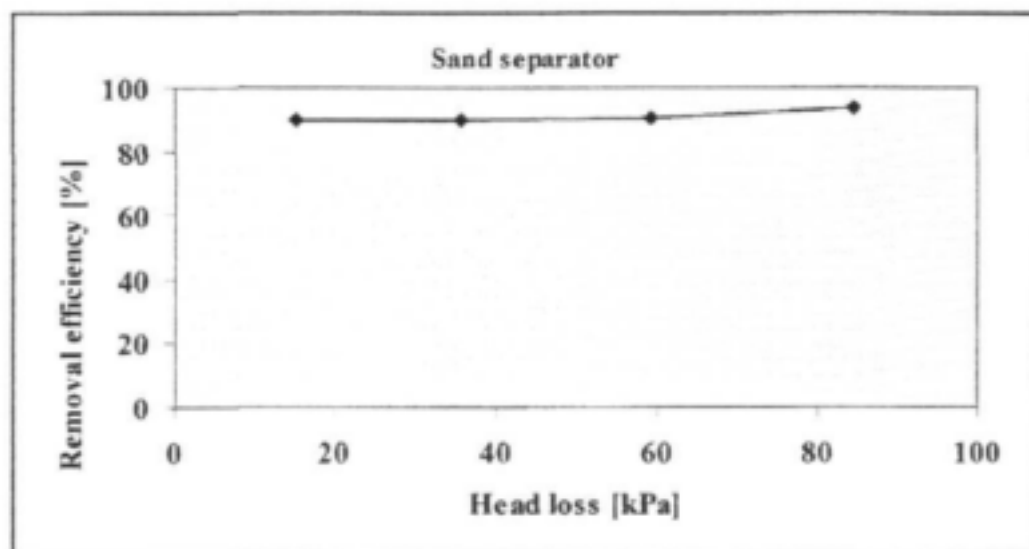
Fig. 2.7: Removal efficiency of a sand separator (after Norum, 1999)
