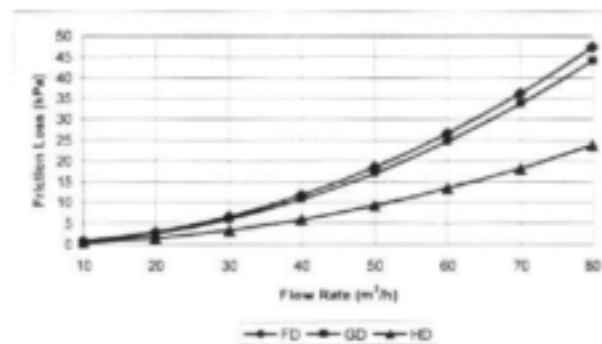
Fig. 4.7: Friction loss curves for the three different filter discs in the same casing
