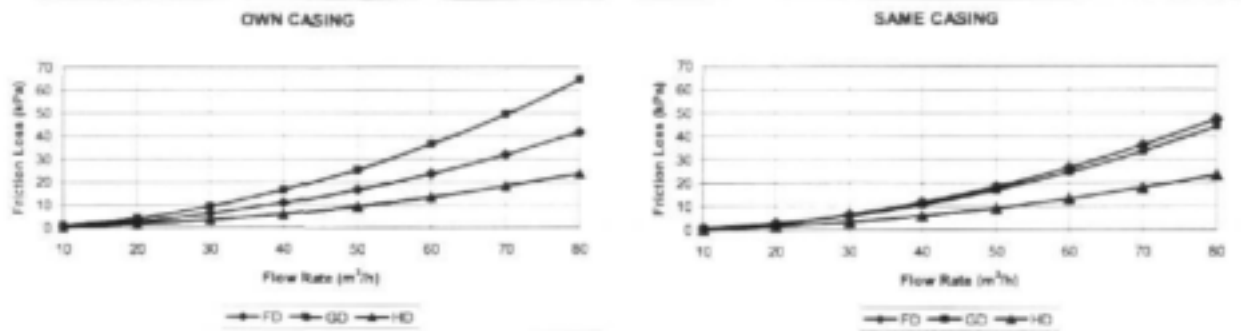
Fig. 4.10: Friction loss curves for the three different filter discs in their own and same casing
