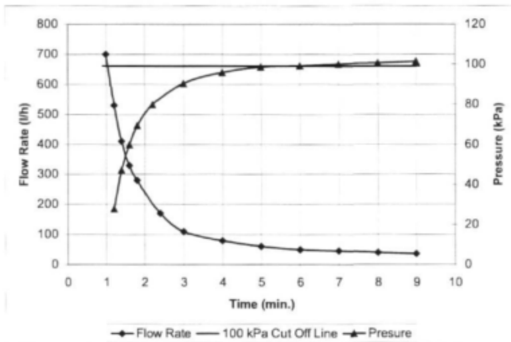
Fig. 2: Flow-rate and pressure build up characteristics of the Dirtiness Index Meter
