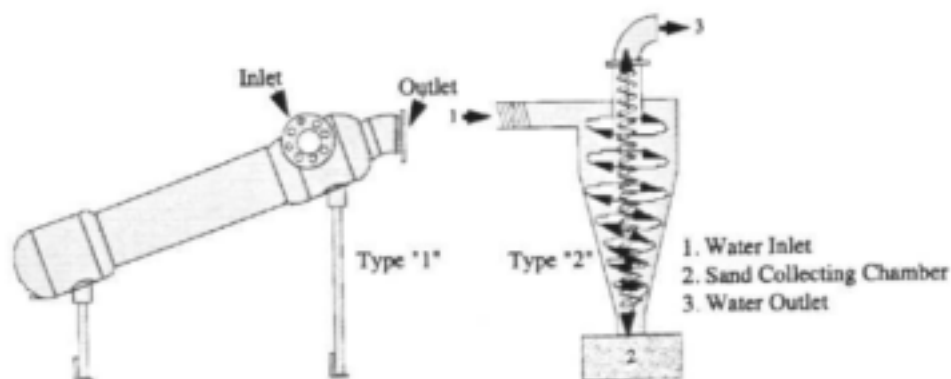
Diag. 2.4: Two types of sand separators (Burt and Styles, 1994)
