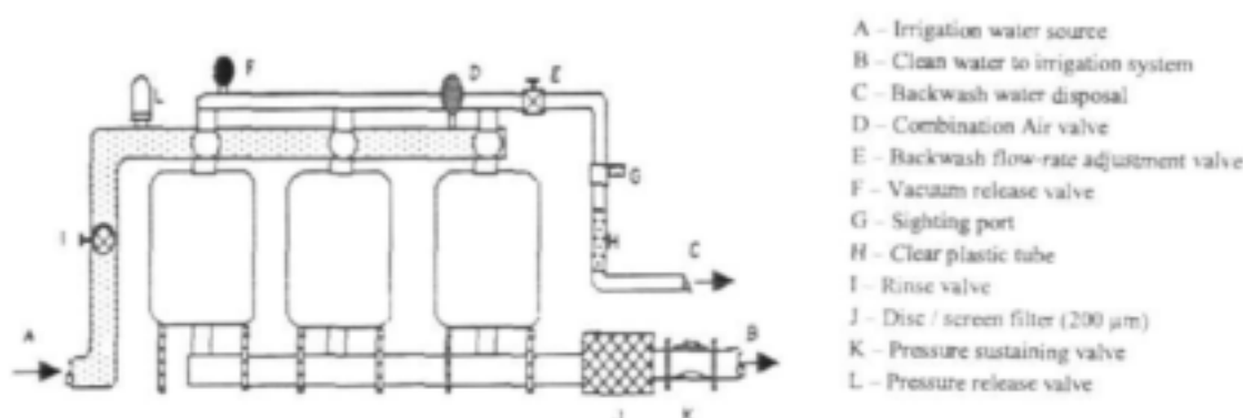
Fig. 6.1: Typical layout of three sand filters with accessories (adopted ed. From Burt & Styles, 1994)
