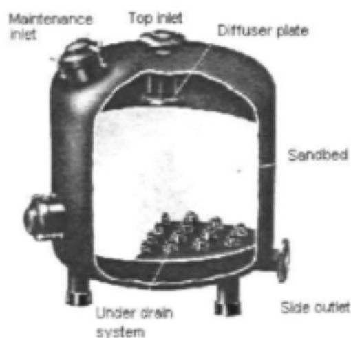
Fig. 2.1: Components of a sand filter (Amiad, 2002)
