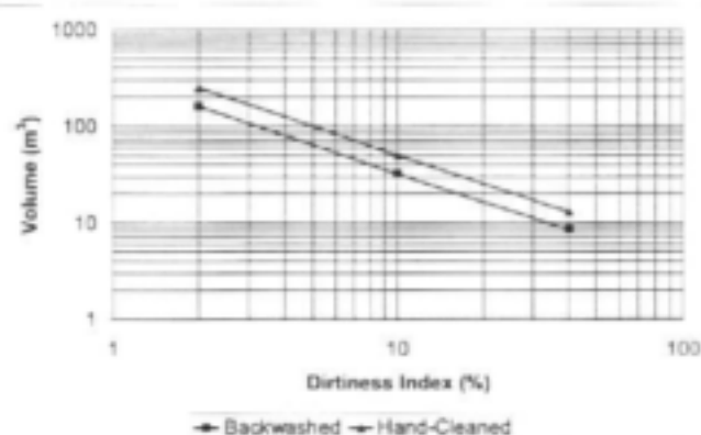
Fig. 3.3: A typical filtration capacity curve of a filter
