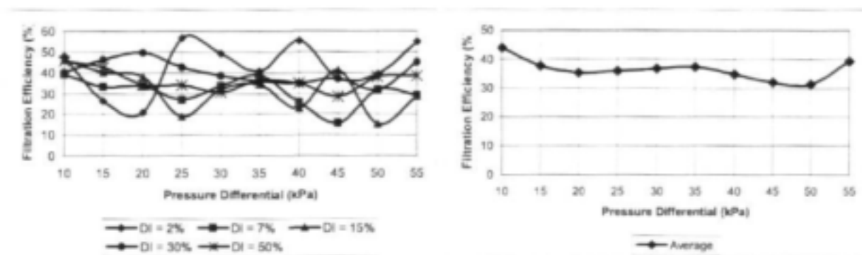
Fig. 4.5: Filtration efficiency during the clogging of a disc filter
