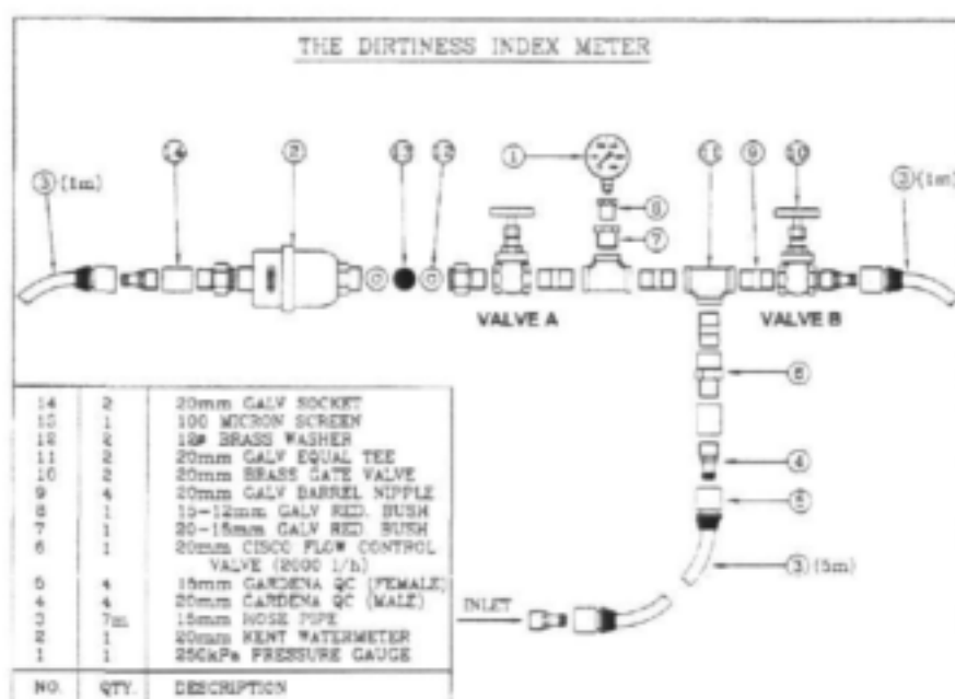
Fig. 1: Construction of the Dirtiness Index Meter
