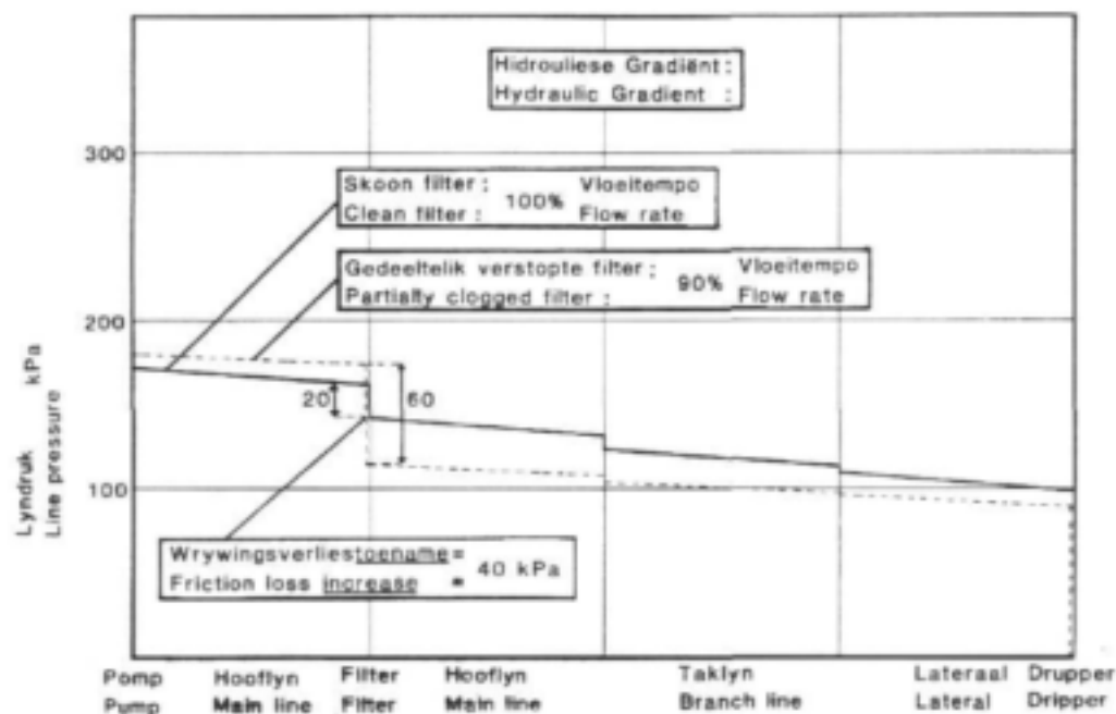
Diag. 2.3: Permissible friction loss increase over a filter if it is accepted that the discharge of the furthest dripper should not decrease by more than 10% as a result of the clogging of the filter (Van Niekerk, 1989)
