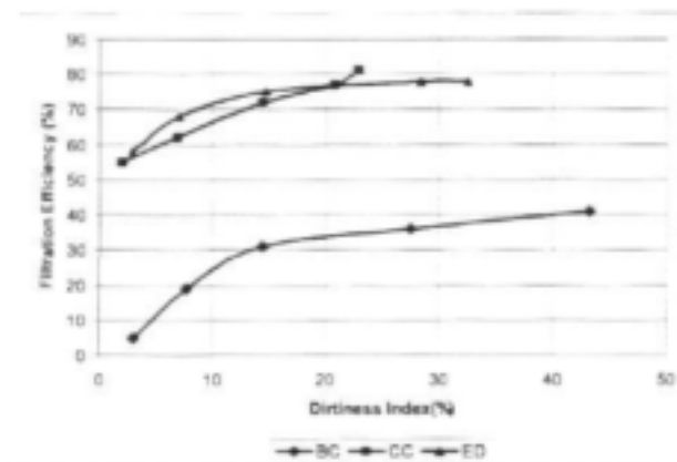
Fig. 4.15: Filtration efficiency test results on the automatic filters
