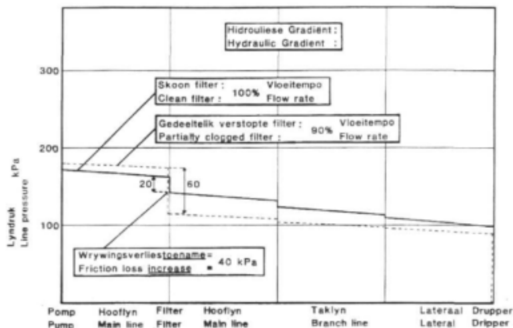
Diagram 6.1: Permissible friction loss increase over a filter
