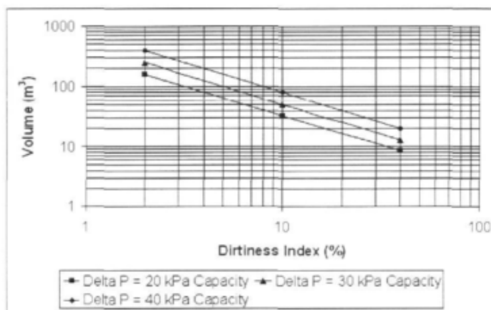
Fig. 6.4: Dirty water capacity graph for the Silicon II sand filter
