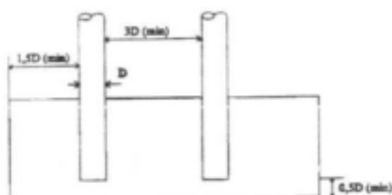
Fig. 6.2: Minimum distances between suction pipes and sides, and bottom of pump hole
