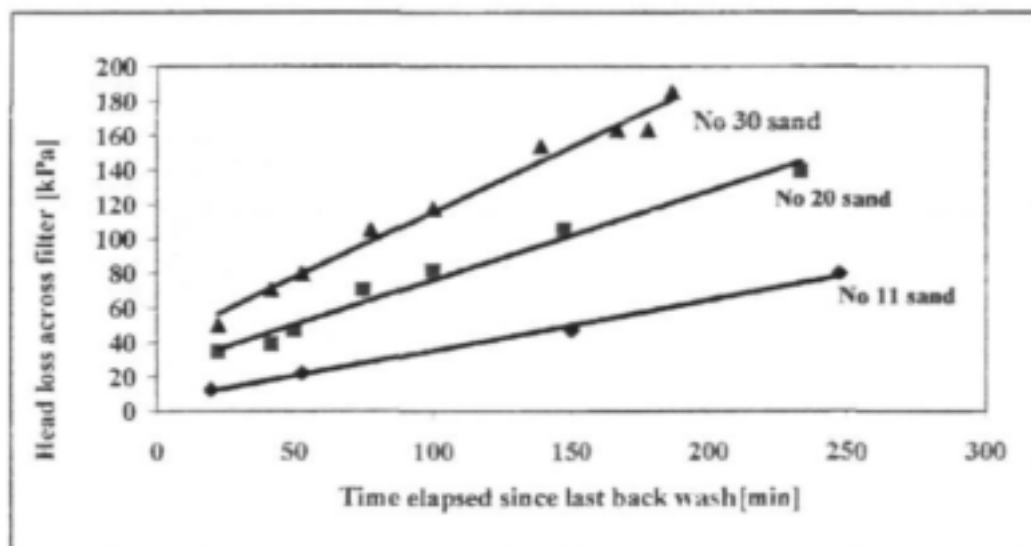
Fig. 2.9: Head losses versus elapsed time since last backwashing (after Haman et al. 1994)
