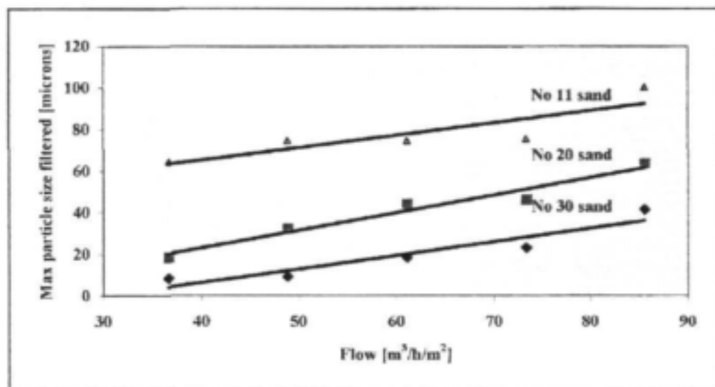
Fig. 2.8: Maximum particle size filtered versus flow per area (after Haman et al. 1994)
