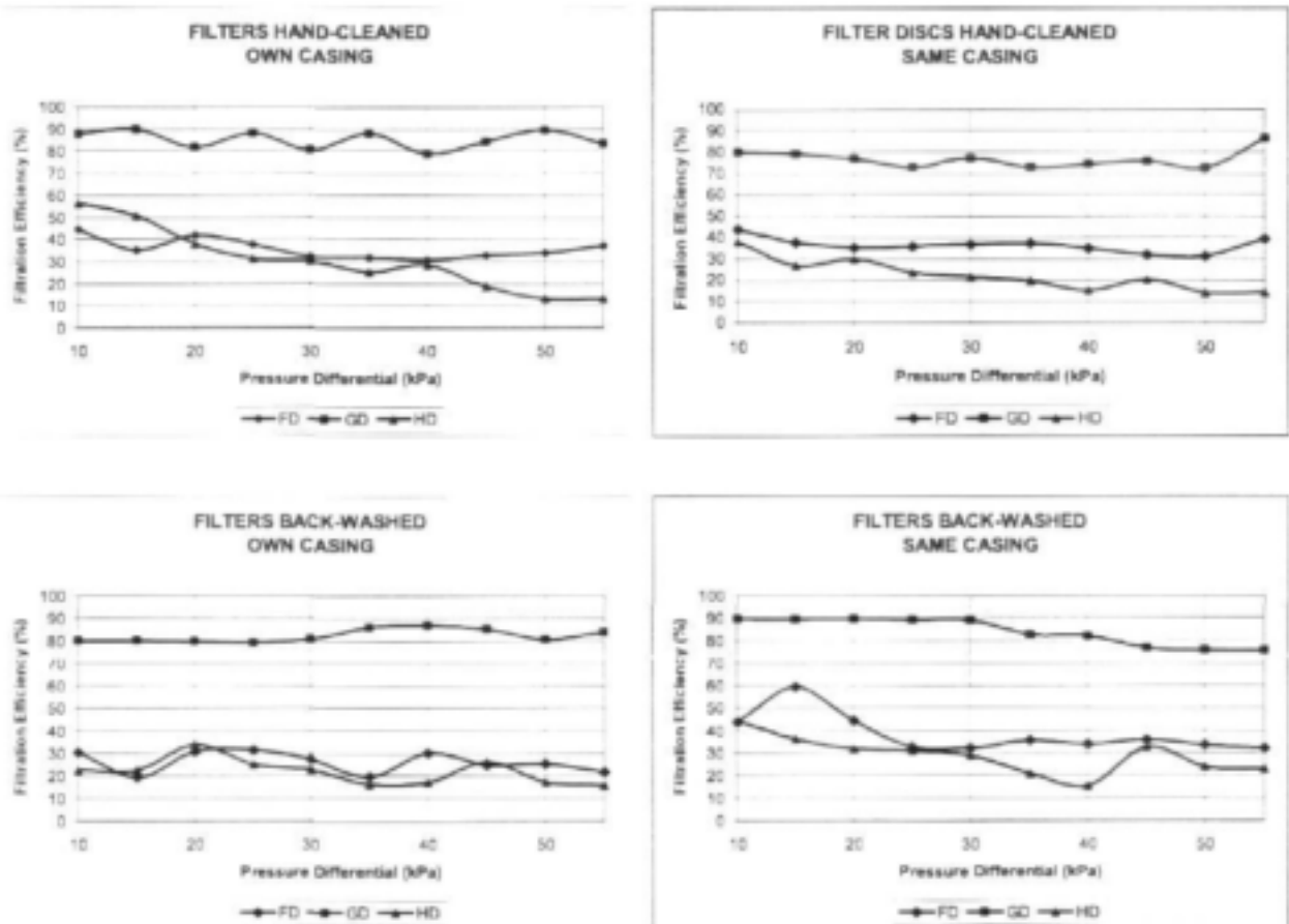
Fig. 4.11: Filtration efficiencies for three different filter discs in their own and same casing
