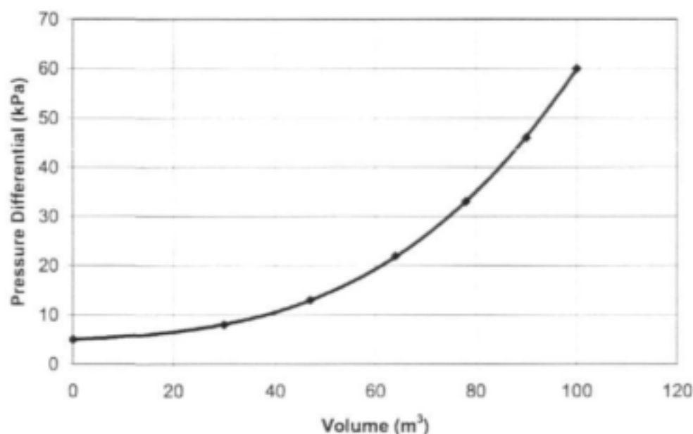
Fig. 2.5: Typical clogging graph of a filter (Van Niekerk, 1983)
