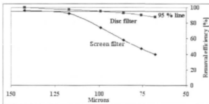
Fig. 2.6: Removal efficiency of a screen and a disc filter (after Norum, 1999)
