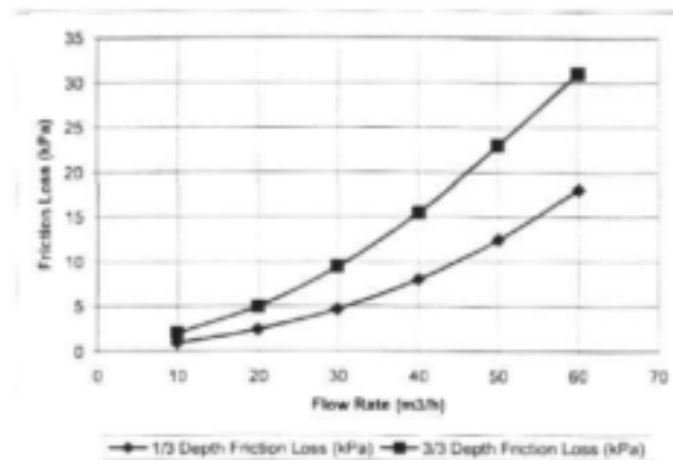
Fig. 4.14: The effect of the sand depth in a sand filter on its friction loss
