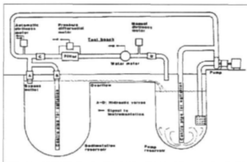
Illustration 1: The irrigation filter test bench
