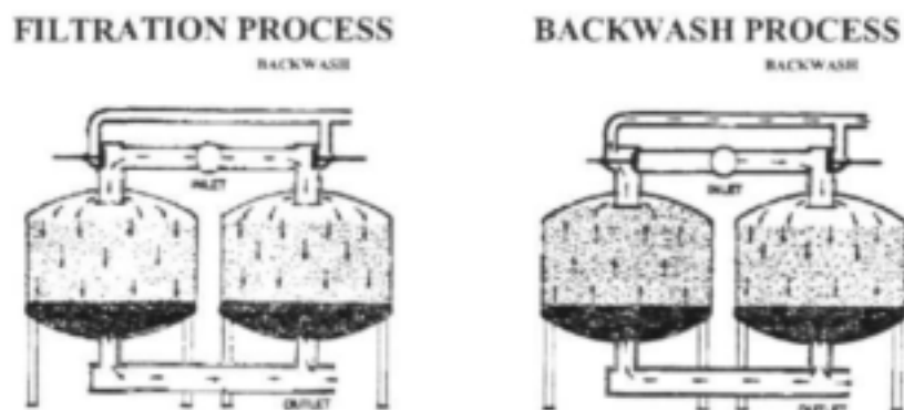
Diag. 2.1: Filtering and backwashing with sand filters (Burt and Styles, 1994)
