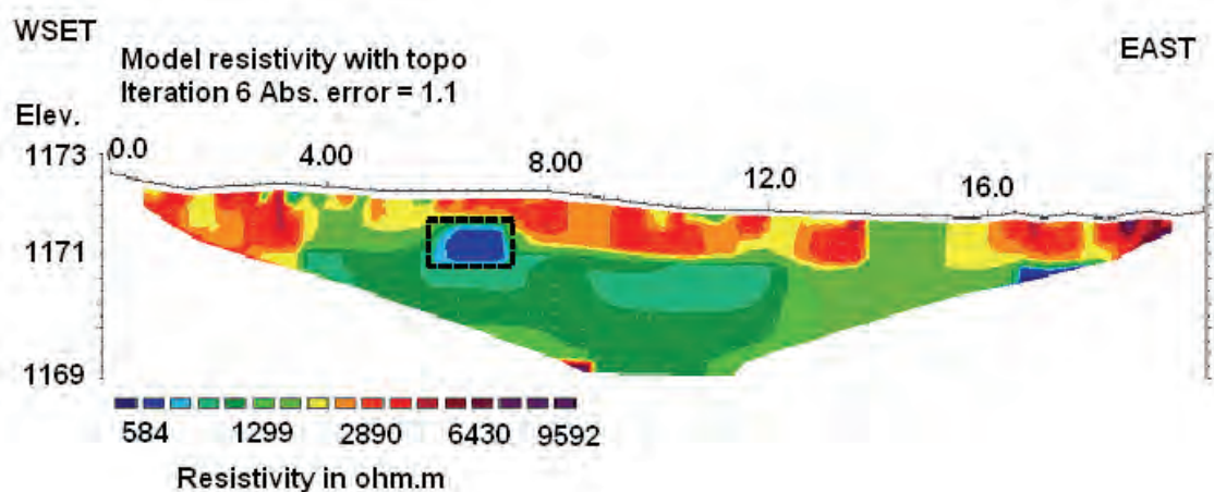
Figure 6.12 Resistivity for transect of T4 plot (12-18 July 2011)
