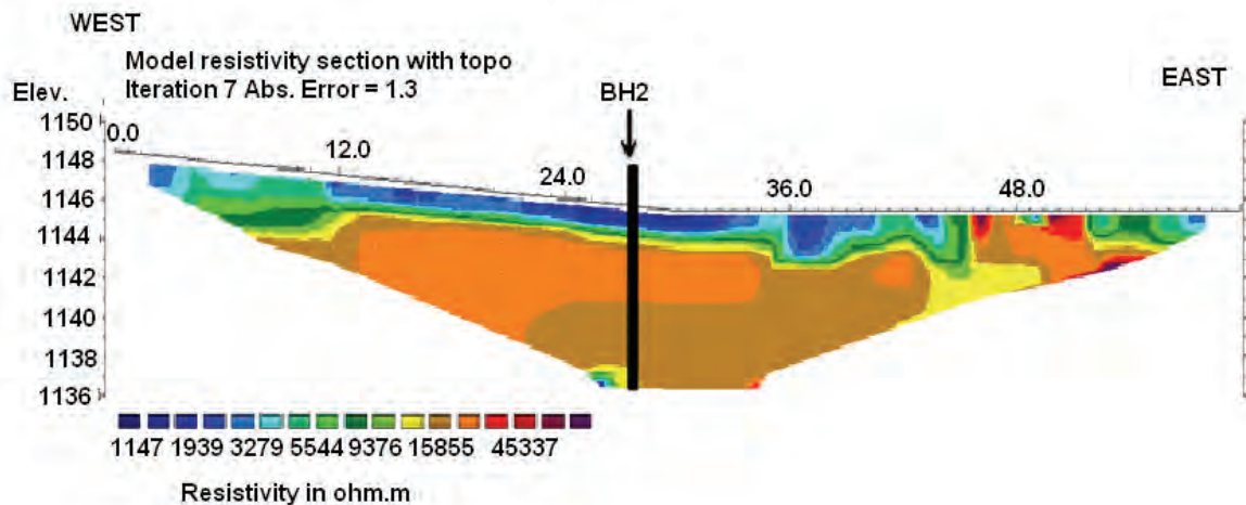
Figure 6.7 Resistivity for transect near Borehole BH2 (12-18 July 2011)
