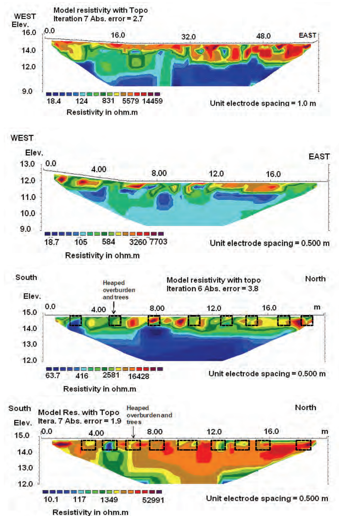
Figure 5.34 ERT inverse model resistivity section Umlazi 1-4 from top to bottom (July, 2011)
