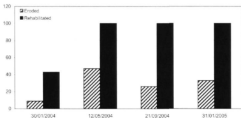
Figure 3. Basal cover (%) at the Jakalasi site (Ingubhela).
