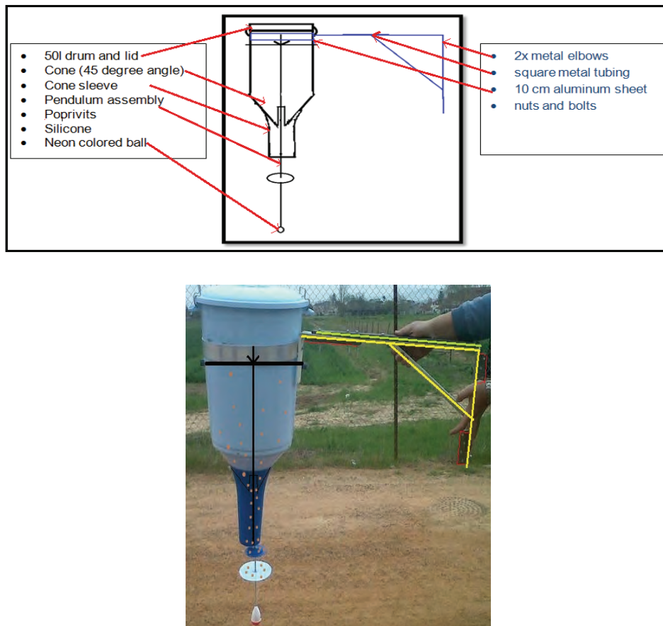
Figure 3.7. Illustration and picture of the demand feeder built by the research team.
