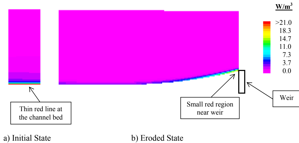
Figure 9-2: Typical unit stream power contours associated with scour upstream of a weir (McGahey, 2001)
