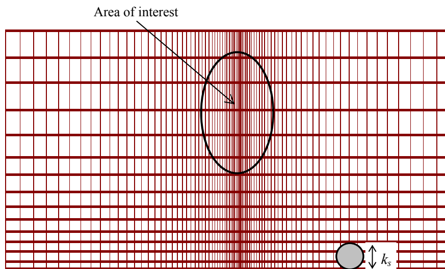
Figure 8-1: Typical example of mesh refinement (McGahey, 2001)
