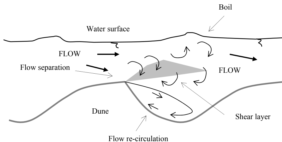
Figure 2-13: Schematic of a shear layer and boil combination over a dune (After Bennett & Best, 1996)
