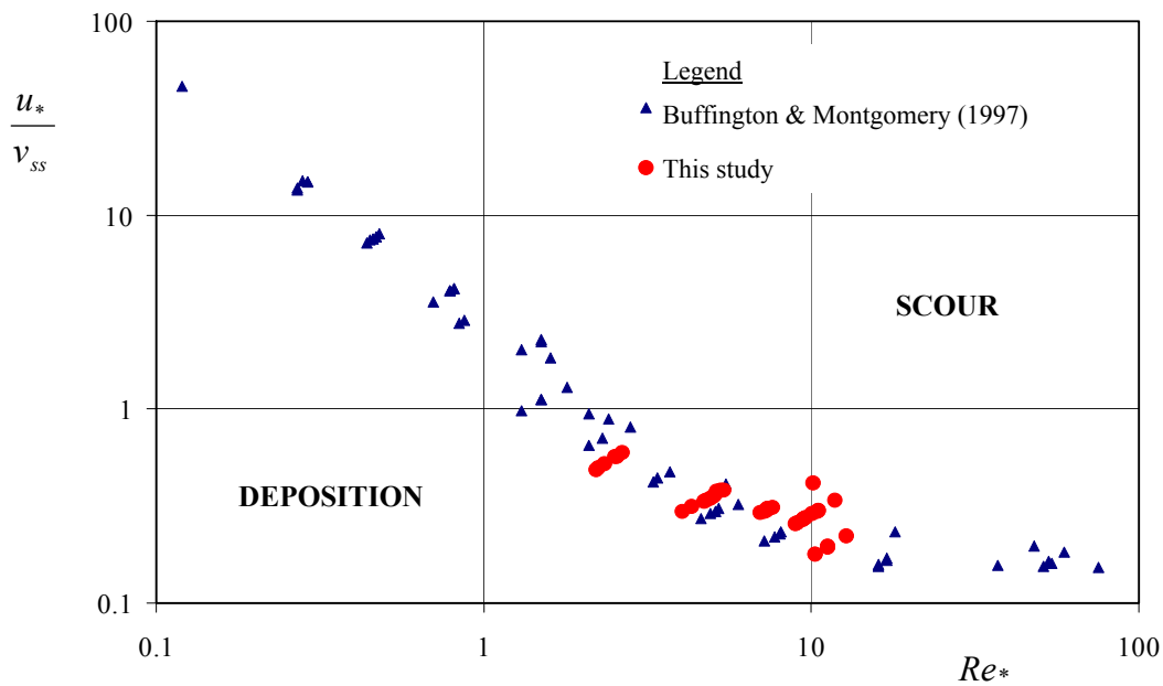
Figure 7-9: Plot of Movability Number versus particle Reynolds Number for the laminar and transitional data
