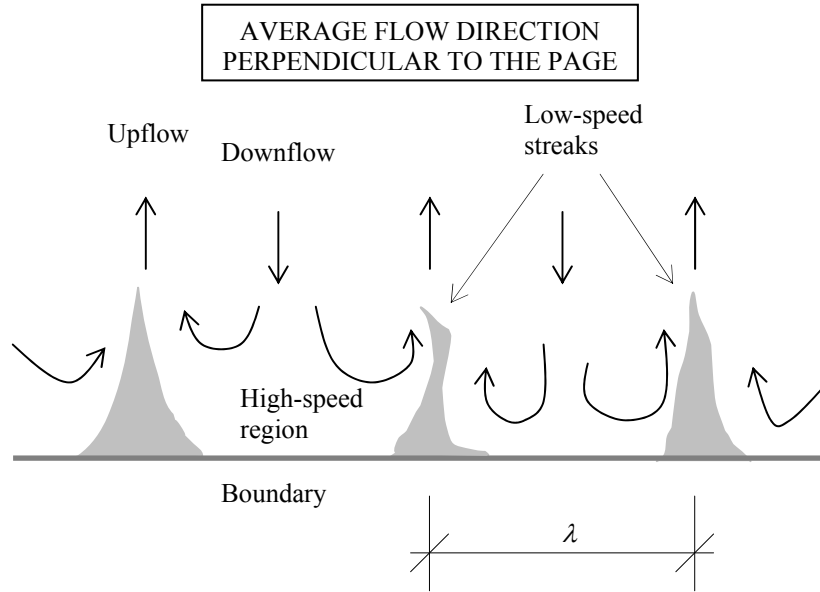
Figure 2-11: Schematic cross-section through the instantaneous velocity field (After Smith, 1996)
