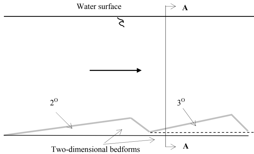
Figure 8-2: The Cellino & Graf (2000) 2D bedforms (McGahey, 2001)
