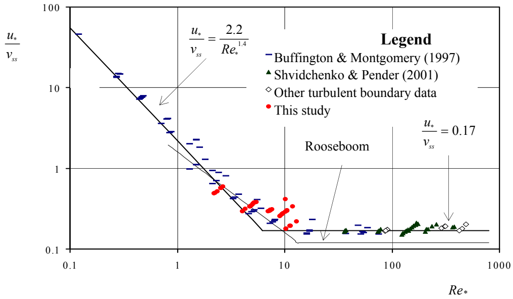
Figure 7-10: Plot of Movability Number versus particle Reynolds Number for all the data describing “weak” motion
