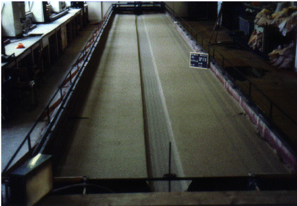
Figure 9-11: A typical self-formed (regime) channel (Babaeyan-Koopaei, 1996)
