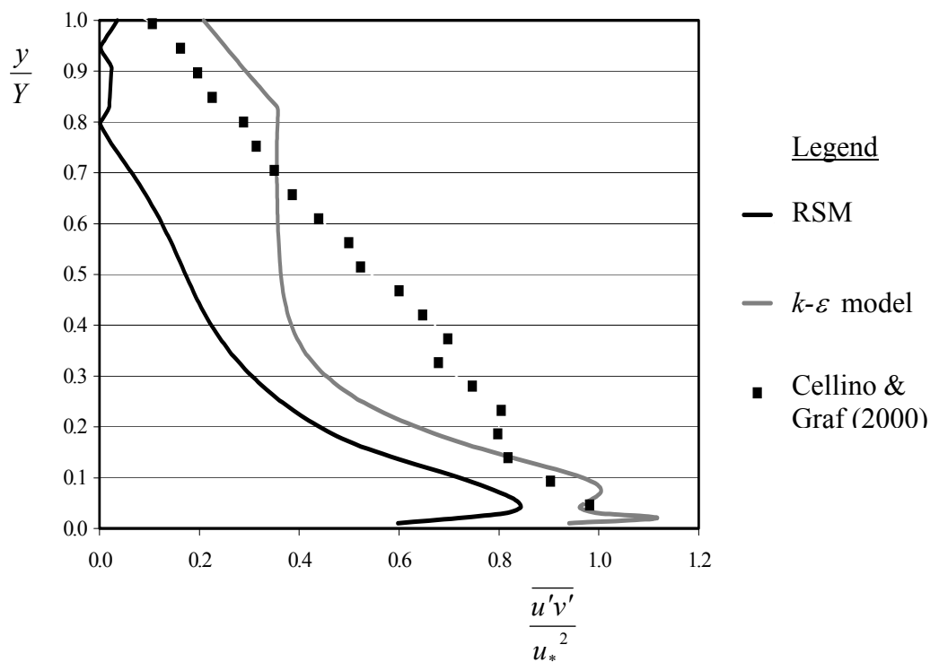
Figure 8-4: Cellino & Graf (2000) - Relative shear stress versus relative depth (McGahey, 2001)
