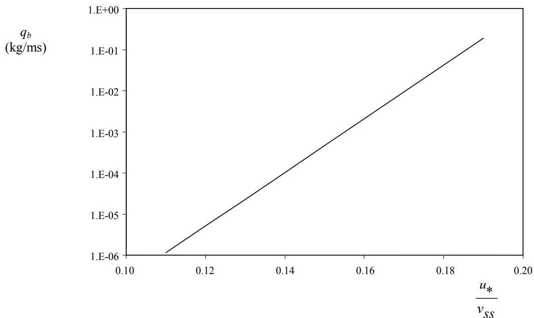
Figure 7-6: Plot of unit bedload transportation rate versus Movability Number for 1 mm diameter quartzitic sand
