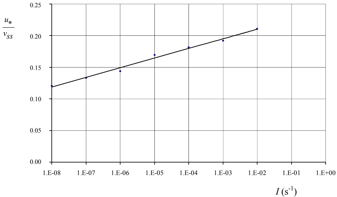
Figure 7-3: Variation of Movability Number with intensity of motion for a flat turbulent bed and zero relative roughness (Semi-logarithmic plot)
