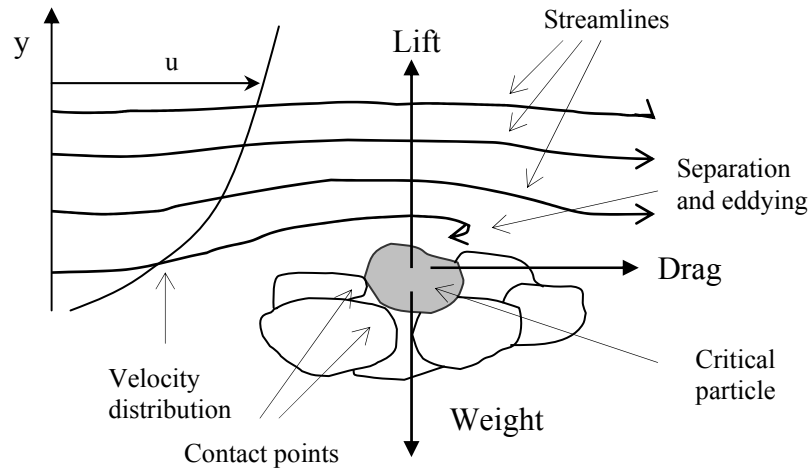
Figure 3-1: Forces on a sediment particle (horizontal bed)
