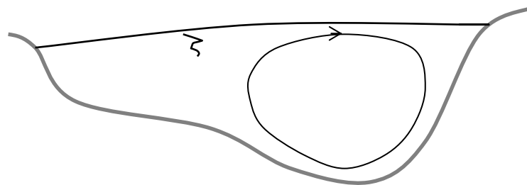
Figure 2-9: Typical secondary flow cell on a bend
