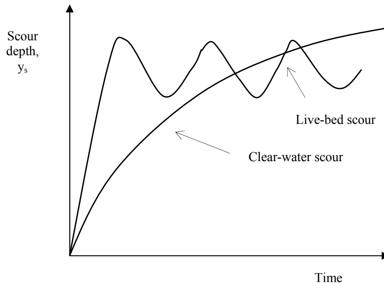
Figure 5-1: Scour depth as a function of time
