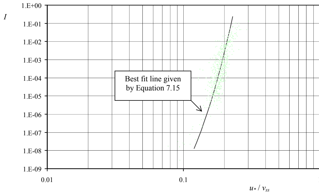
Figure 7-4: Comparison of new intensity of motion equation for turbulent boundaries with adjusted data set
