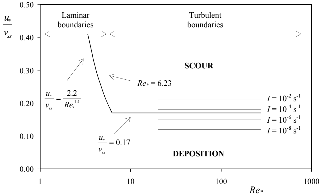
Figure 7-11: New criteria for the prediction of scour
