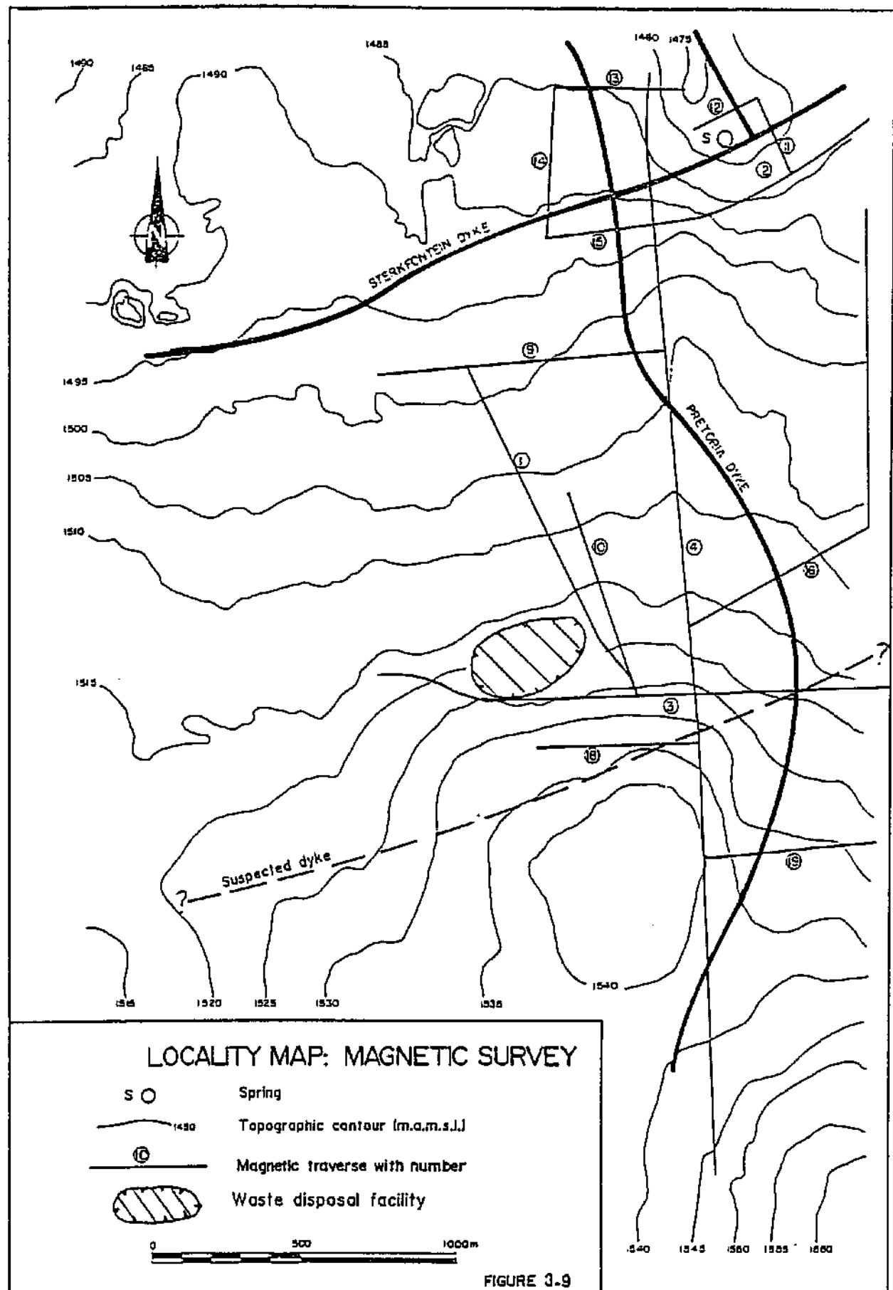
Figure 3.9 Locality map: magnetic survey
