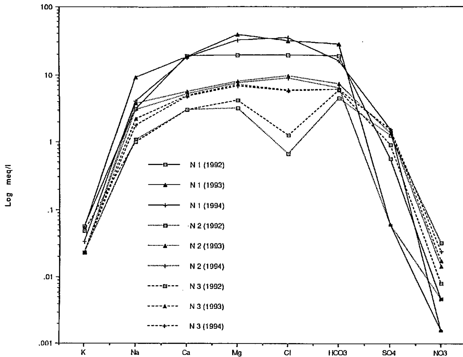
Figure 12.2 Modified Schoeller diagram for Bloemfontein North boreholes
