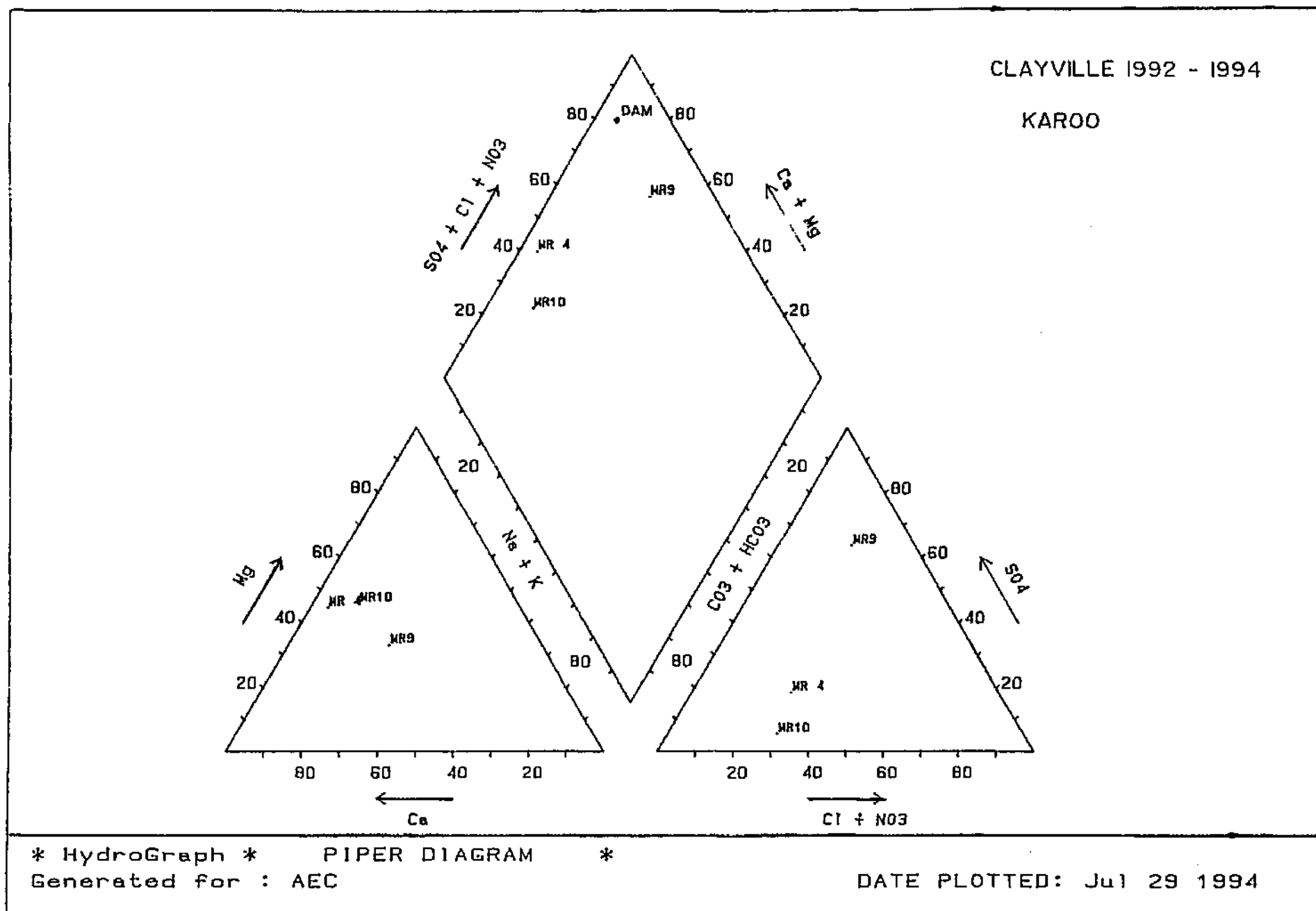
Figure 7.9 Piper diagram - Clayville 1992 - 1994 - Karoo
