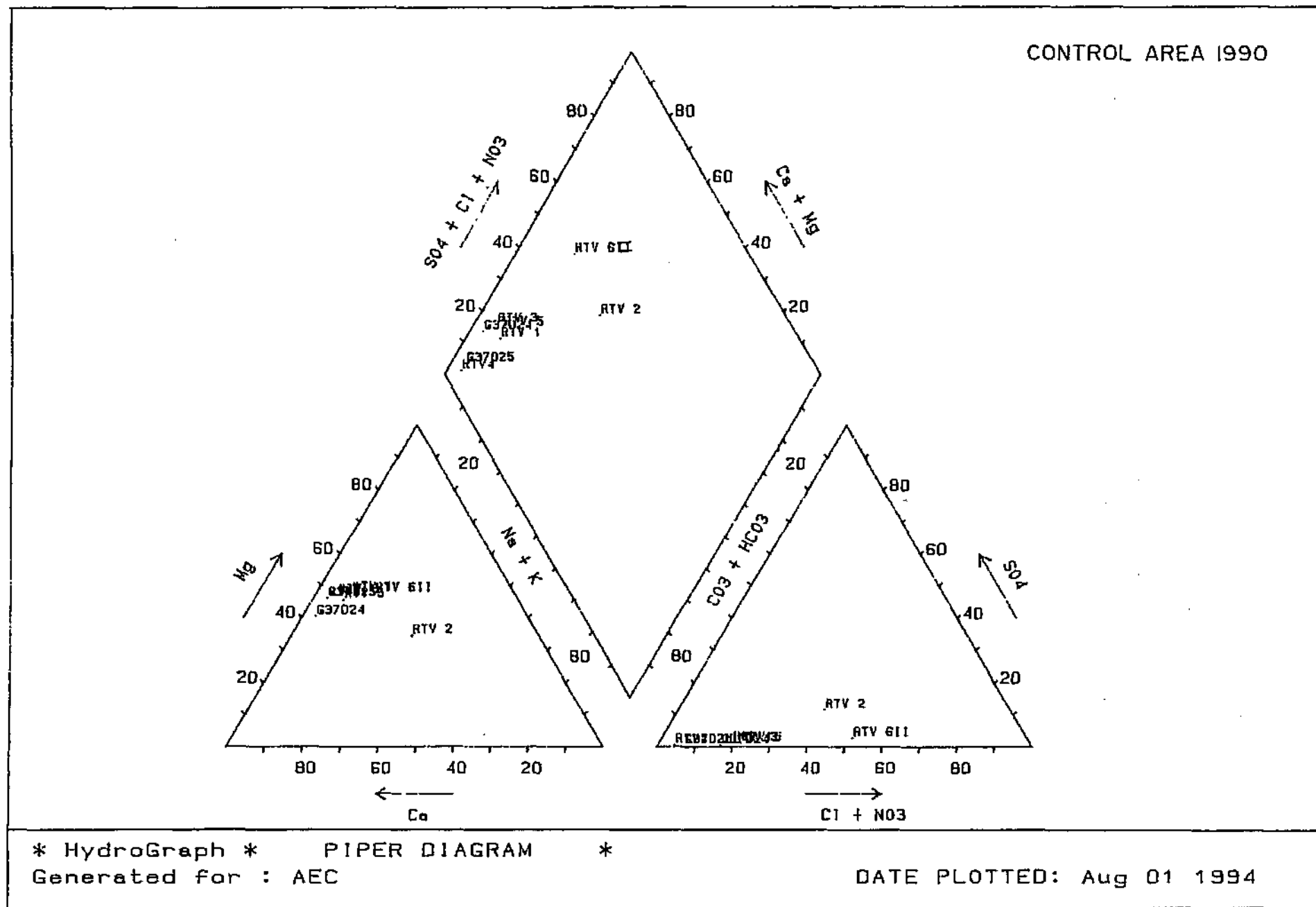
Figure 7.1 Piper diagram - Control area 1990
