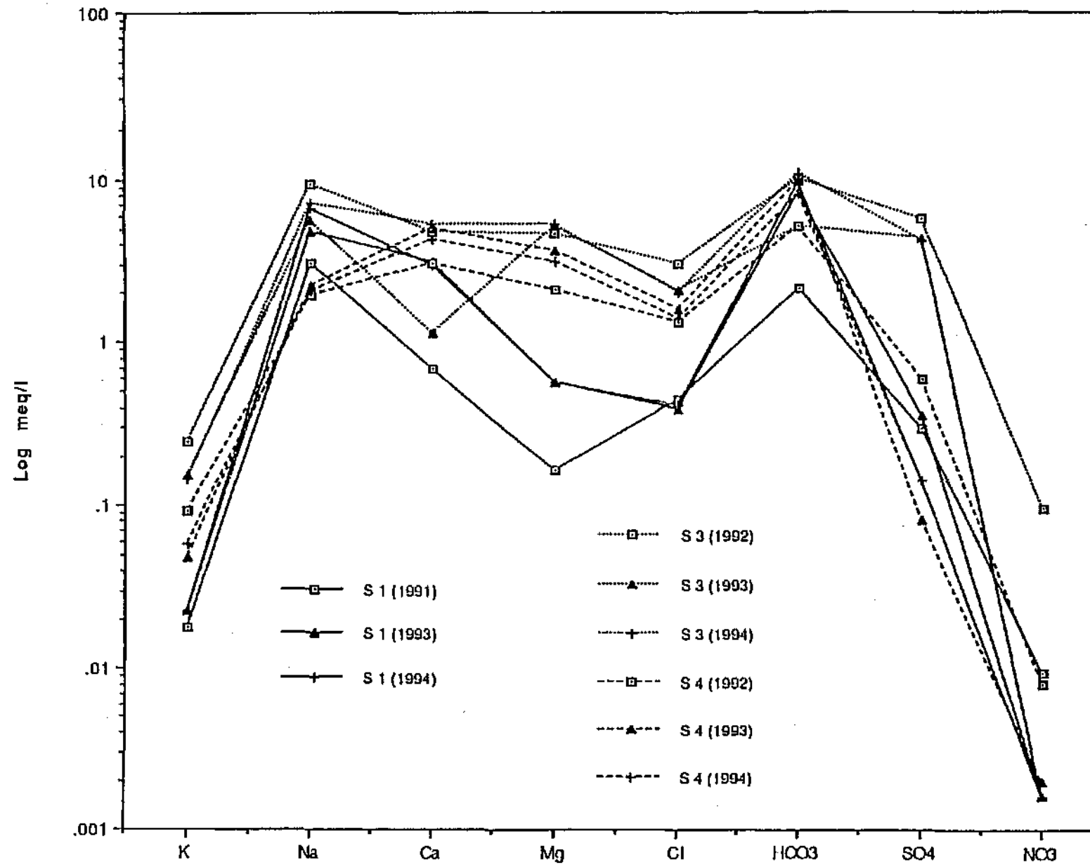
Figure 13.3 Modified Schoeller diagram for "upstream" boreholes at Bloemfontein South
