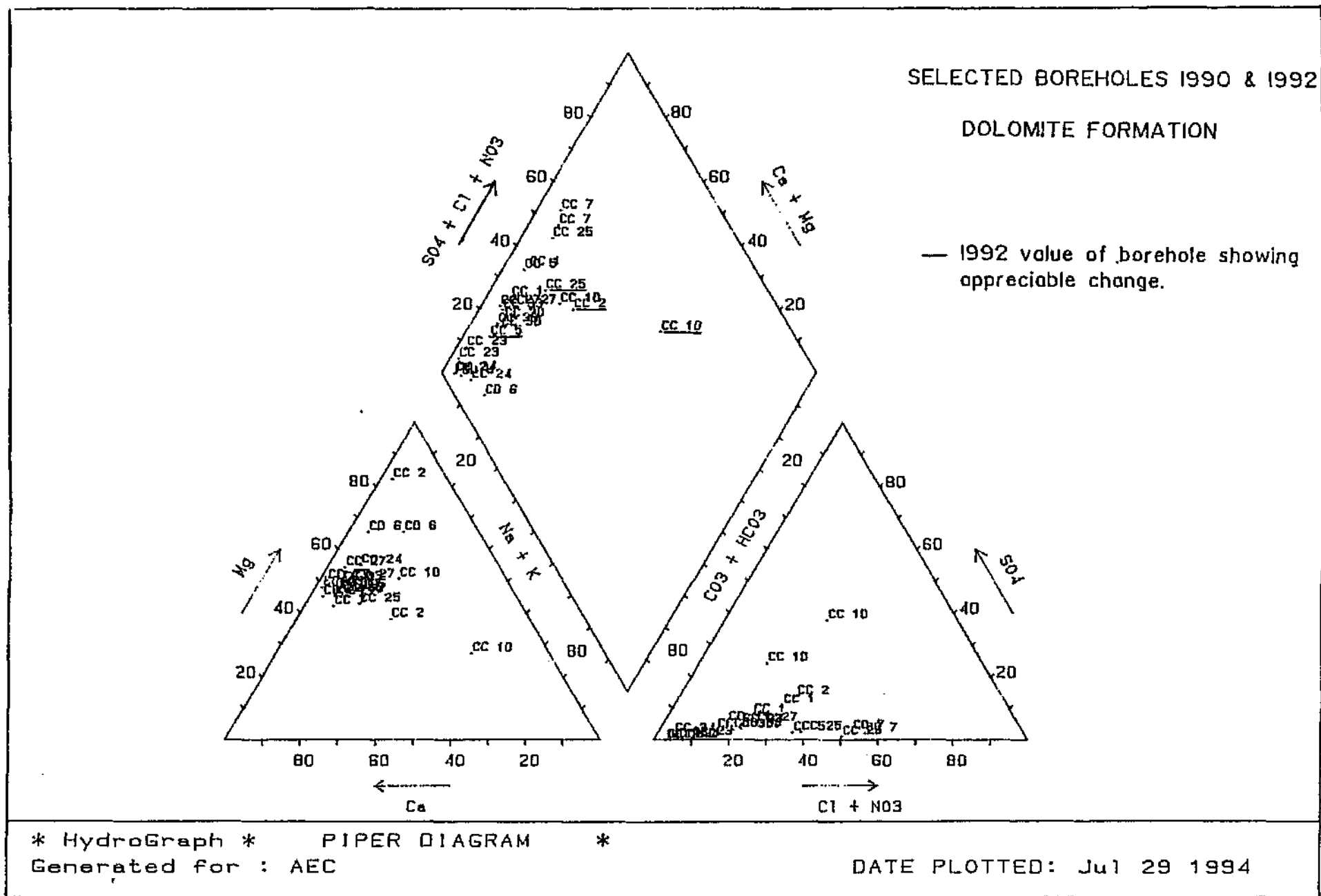
Figure 7.10 Piper diagram - selected boreholes 1990 - 1992 - Dolomite
