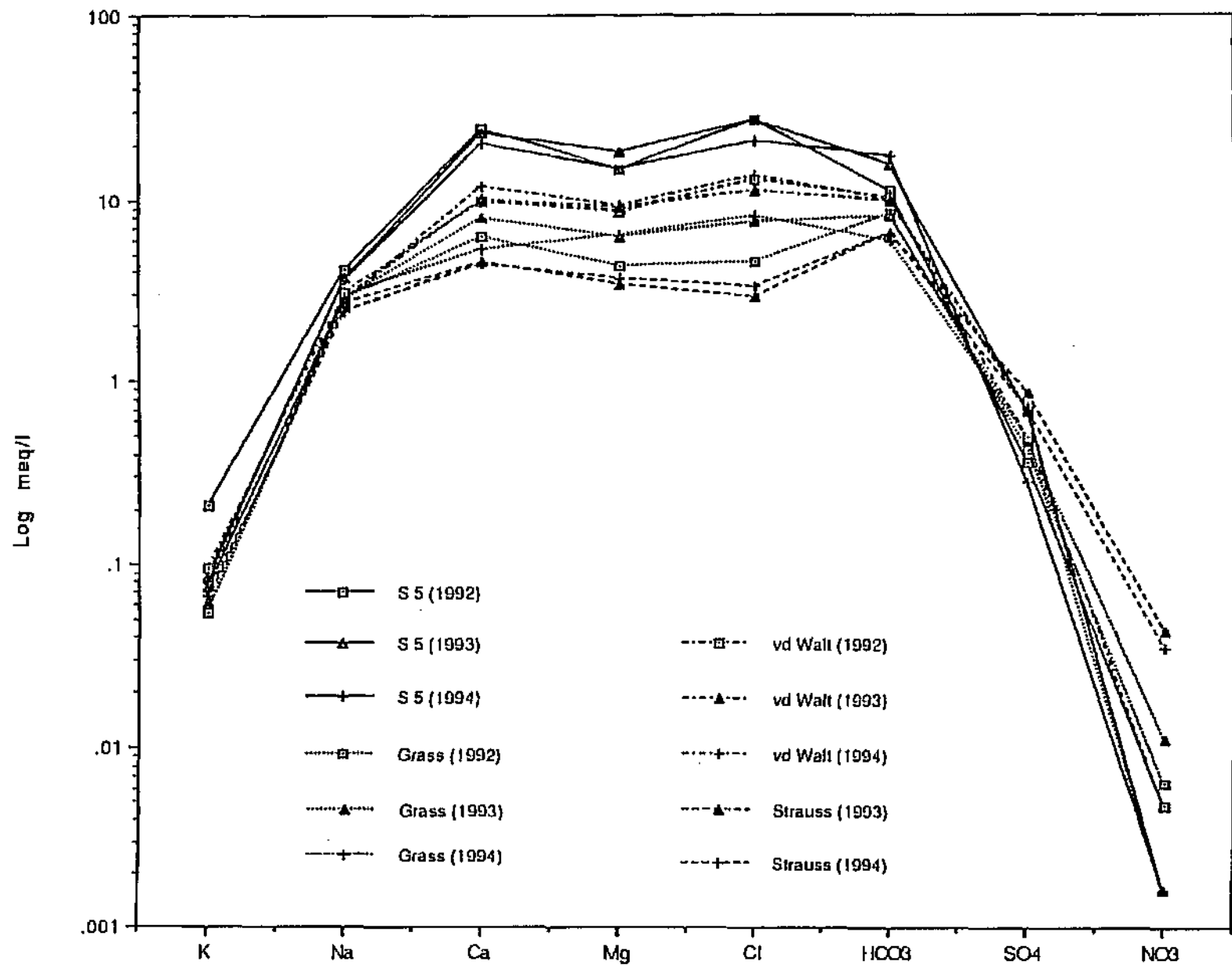
Figure 13.2 Modified Schoeller diagram for "downstream" boreholes at Bloemfontein South
