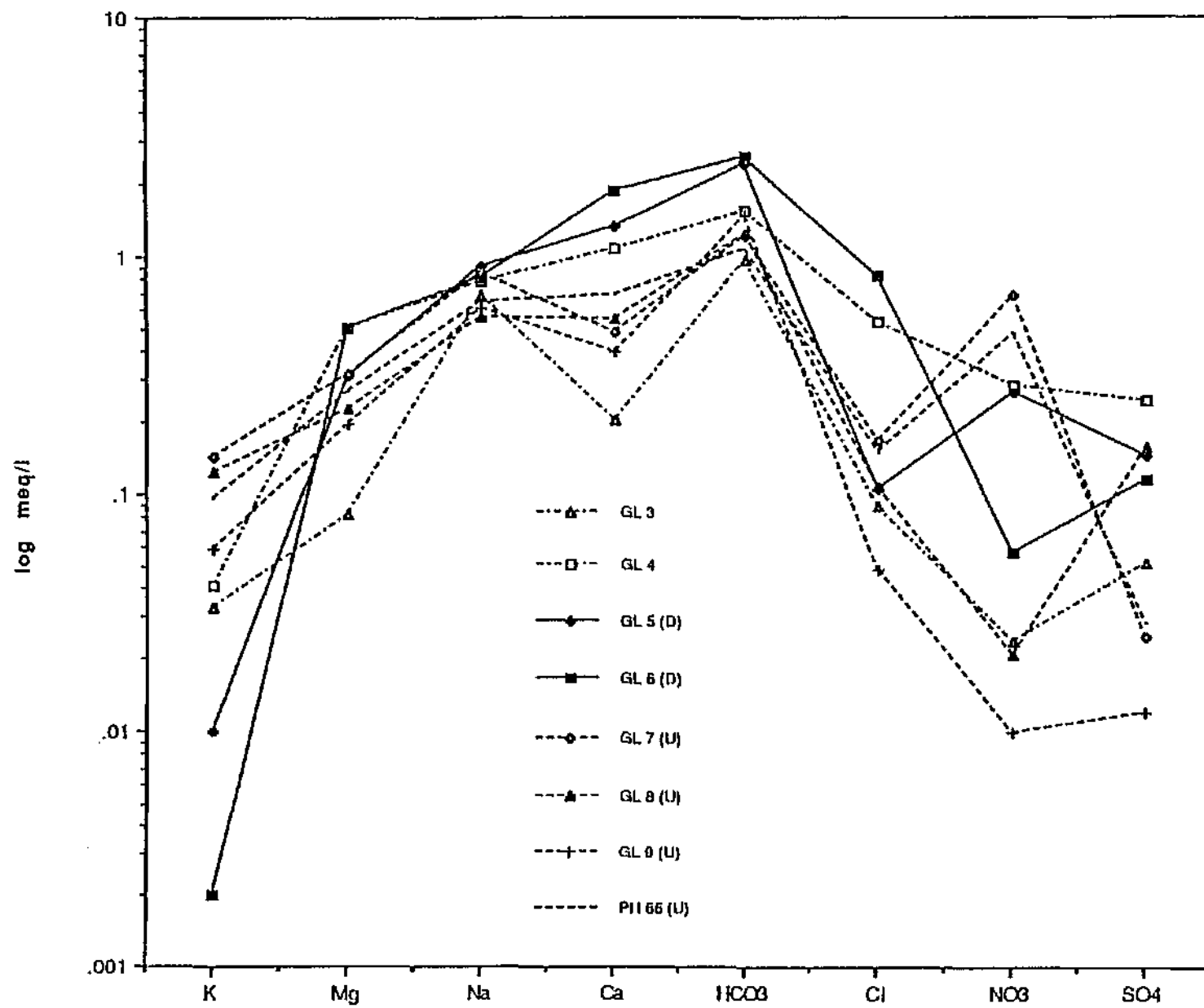
Figure 10.4a Modified Schoeller diagram for Linbro Park boreholes : June 1992
