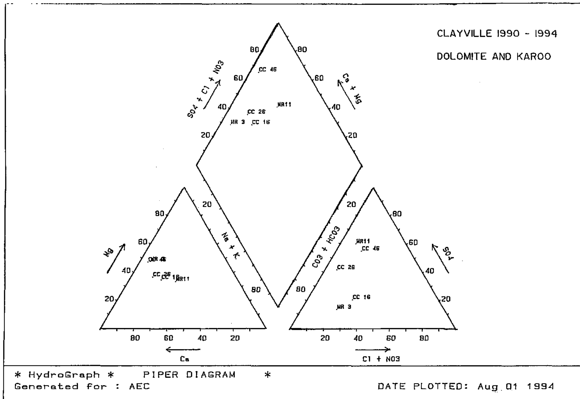
Figure 7.8 Piper diagram Clayville 1990 - 1994 - Dolomite and Karoo
