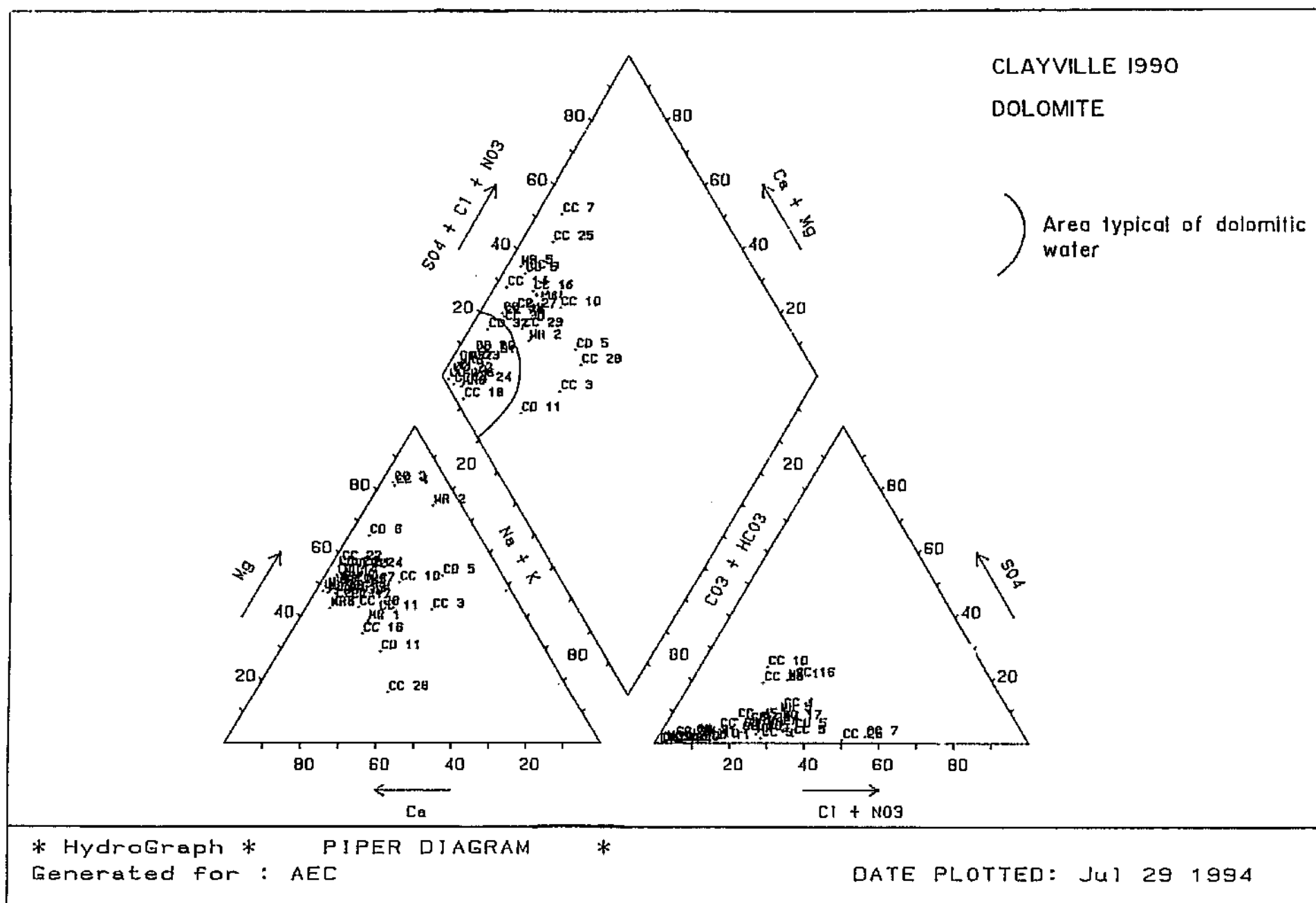
Figure 7.7 Piper diagram - Clayville 1990 - Dolomite
