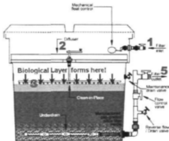
Figure B1.1: Cross-section through BioSand filter
