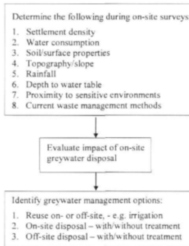
Figure 4.5.1: Greywater management flowchart
