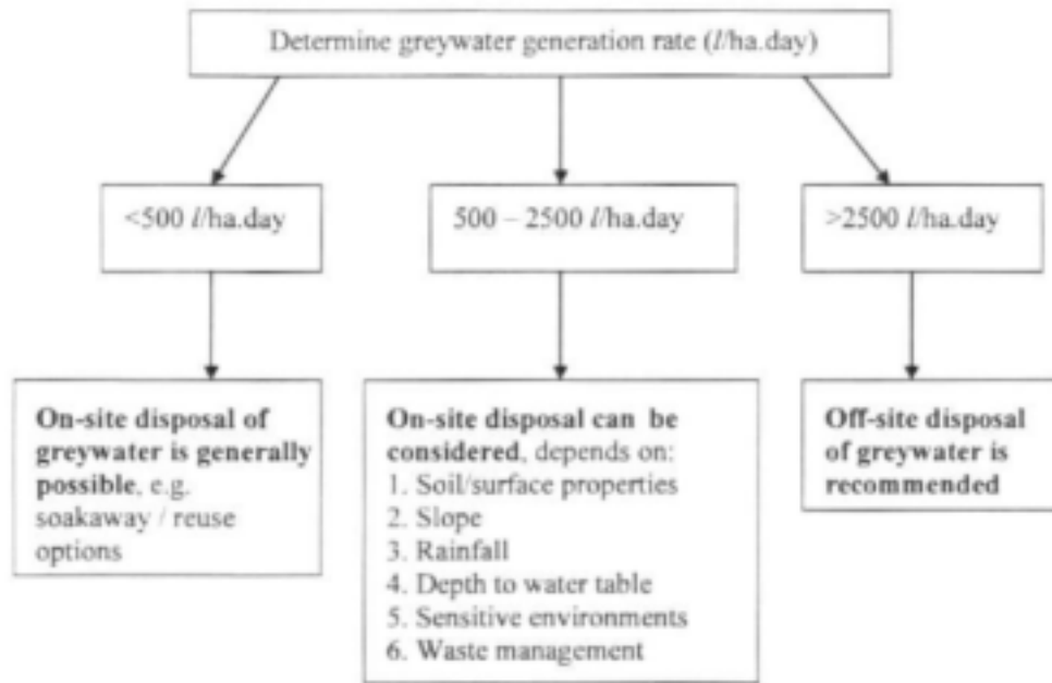
Figure 4.5.2: Decision tree for determining appropriate greywater management options
