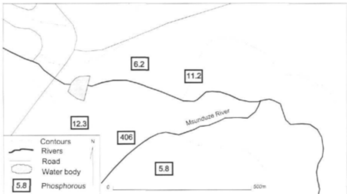
Figure 4.1.3: Total Phosphorous as P (mg/l) in samples collected from KwaShange
