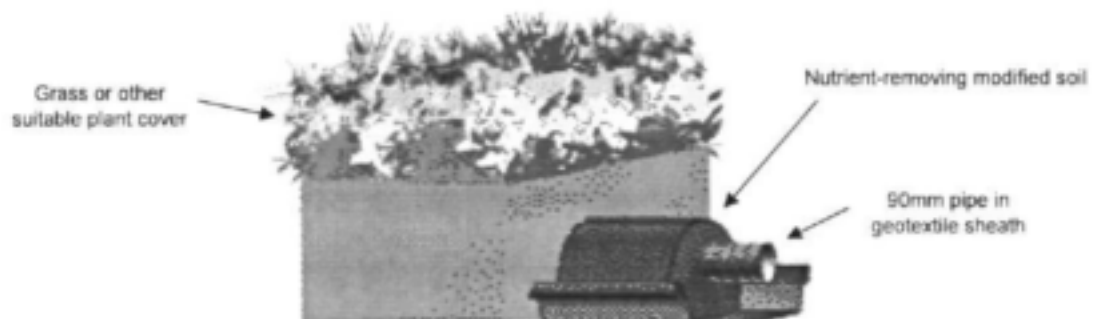
Figure B6.1: Oblique section through Ecomax system
