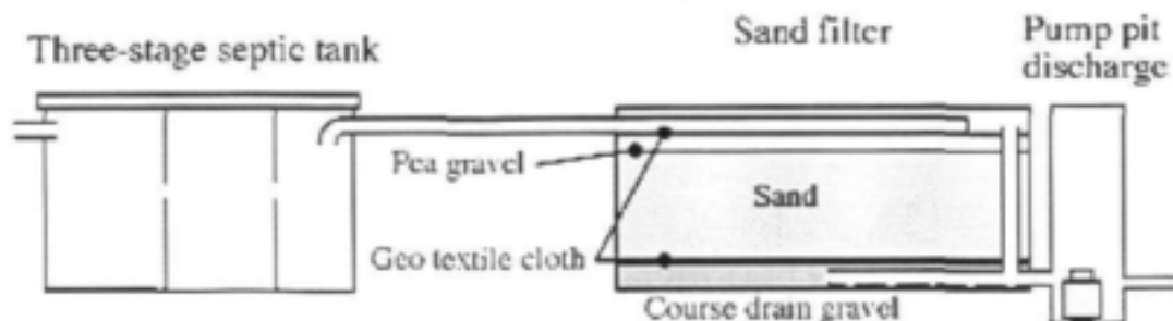
Figure B10.5: Anaerobic to aerobic pre-treatment system
