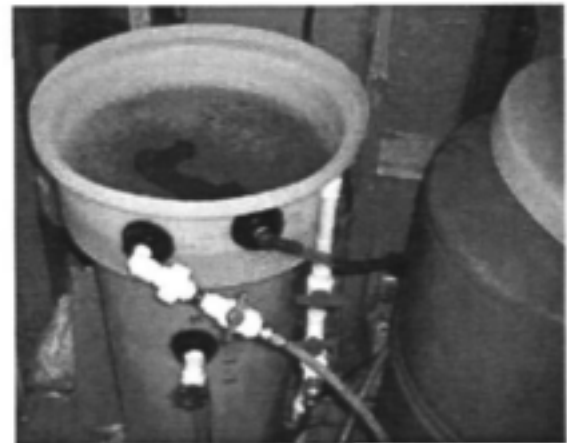
Figure B1.2: Example of BioSand filter installation
