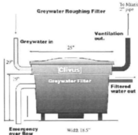
Figure B10.4: Aerobic pre-treatment with Clivus fabric filter
