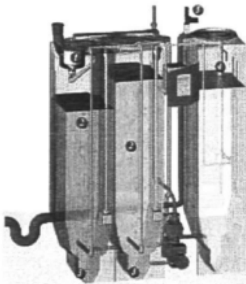
Figure B4.1: AquaCycle 900
