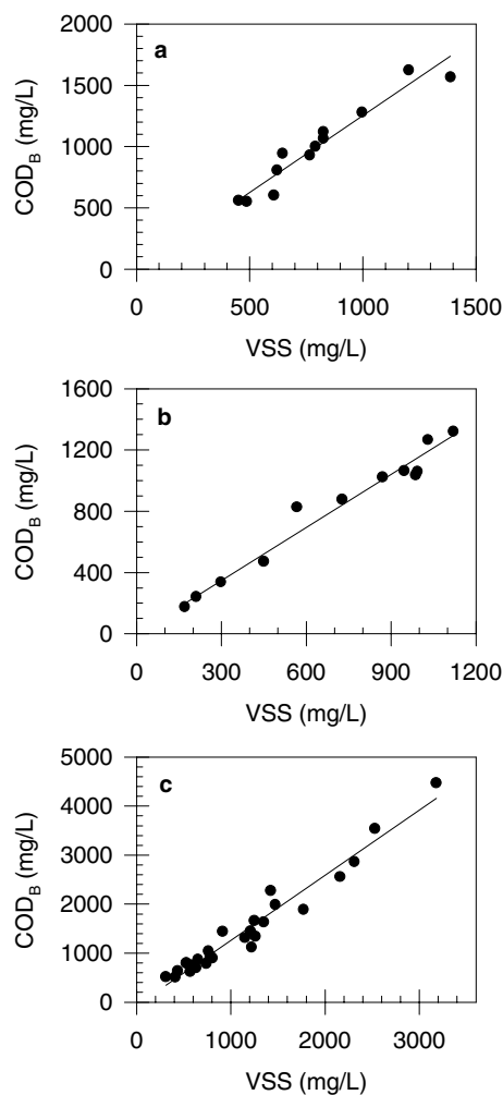
Figure 2 Linear relationship between COD_B (proposed technique) and VSS to determine f_{CV} values for (a) S. natans ( r^2 = 0.9278 , n = 12 ), (b) strain E932 ( r^2 = 0.9657 , n = 12 ) and (c) activated sludge ( r^2 = 0.9541 , n = 27 ).
