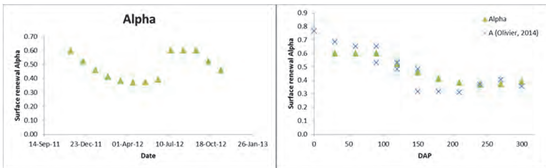
Figure 7. Alpha values used to estimate sensible heat flux using the surface renewal method. Left: Actual alpha values used, against dates and right: Alphas (used and by Olivier, 2014) plotted against days after planting (DAP).
