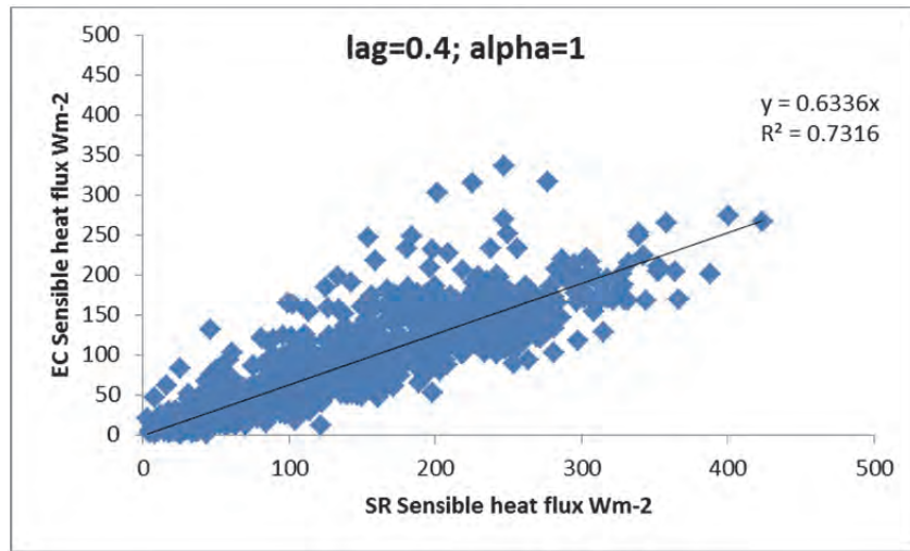
Figure 6. For SR system calibration, the sensible heat flux densities was compared to that from an eddy covariance system
