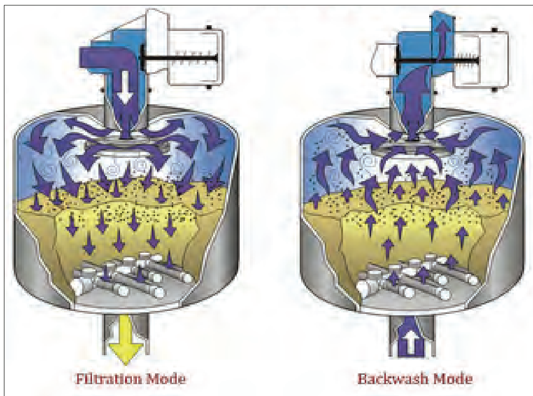
Figure 19: Operation of sand filters
