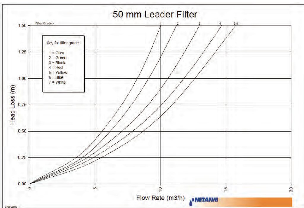
Figure 20: Example of pressure loss graphs (Source: Netafim)
