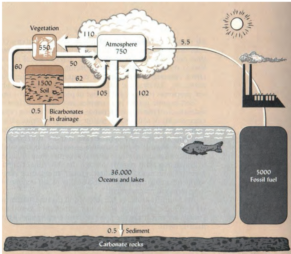
Figure 2.1 The global C cycle indicating the annual C flux in Pg (Brady & Weil, 2002). 1 Pg = 10^{15}
