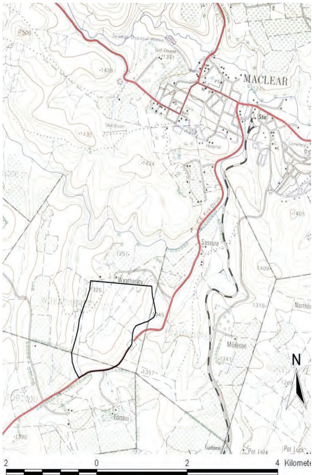
Figure 3.1 Location of the Weatherley catchment, 4 km south of Maclear on the road to Ugie (Chief Director of Surveys and Mapping, 1993)
