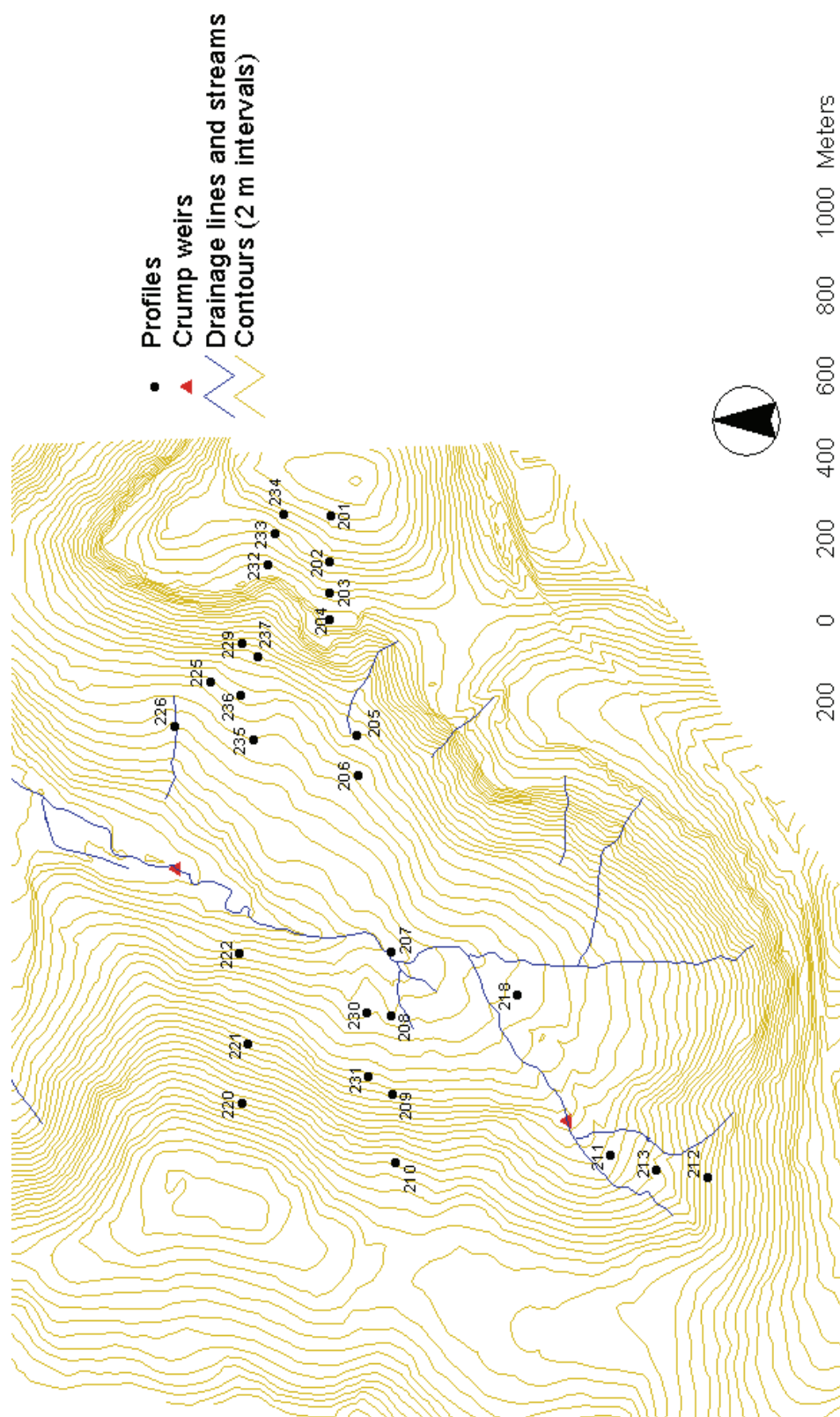
Figure 3.2 Geography of the Weatherley catchment, including the location of the sampling sites (Van Huyssteen et al. , 2005)
