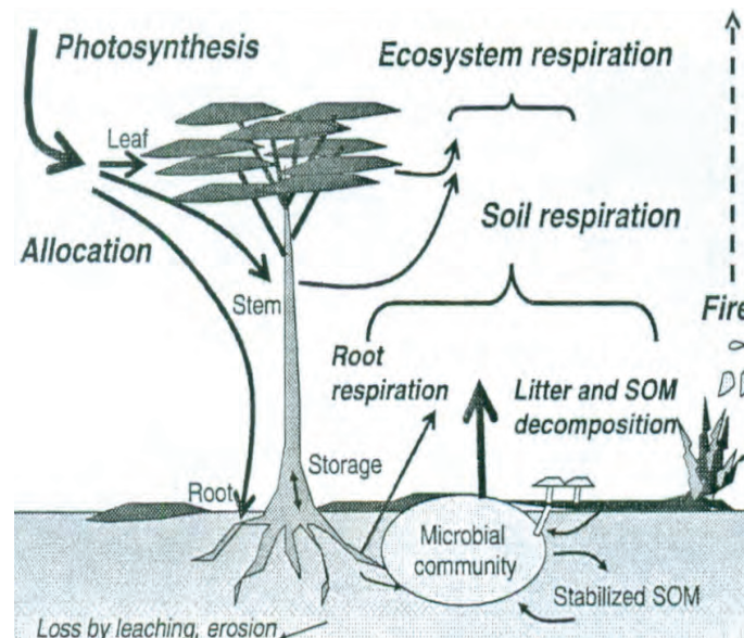
Figure 2.2 Pathways of carbon flow through ecosystems (Trumbore, 2006)
