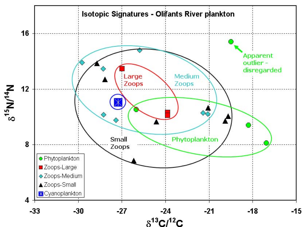
Figure 4. Expanded plots of C^{13} and N^{15} signatures among planktonic components in the Olifants River system.
