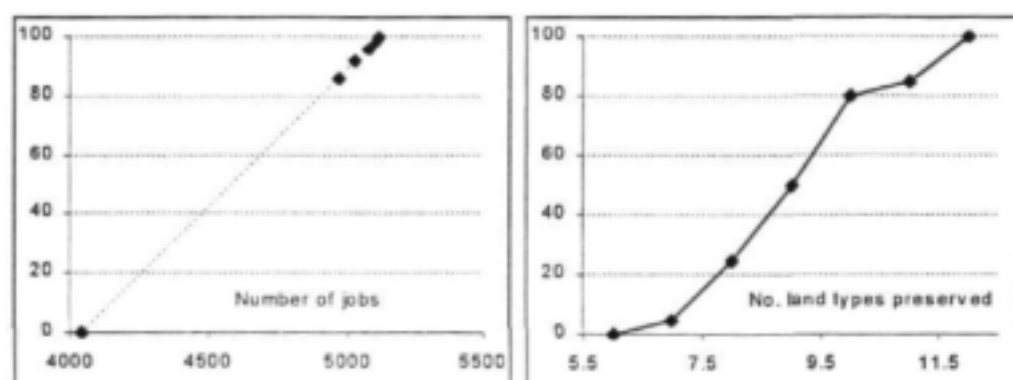
Figure 8.3 (a) The linear value function, and (b) non-linear value function.
