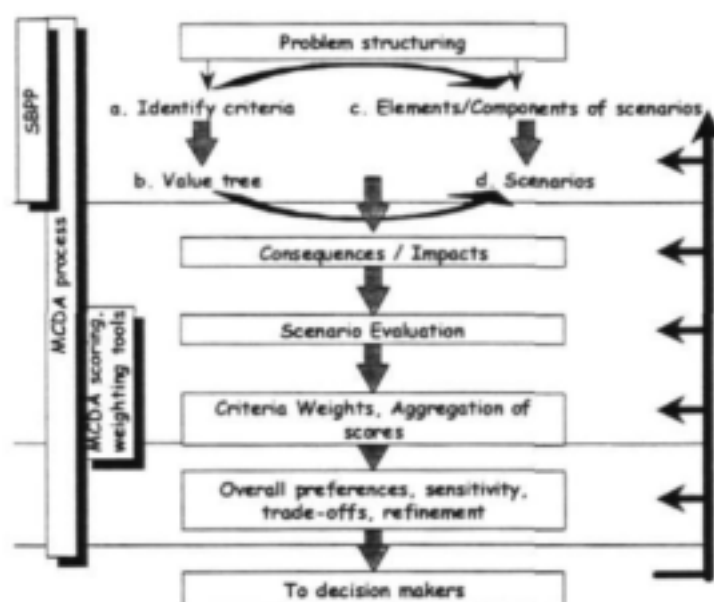
Figure 3.1. Outline of the SBPP/MCDA process. The process is likely to be iterative and non-linear.
