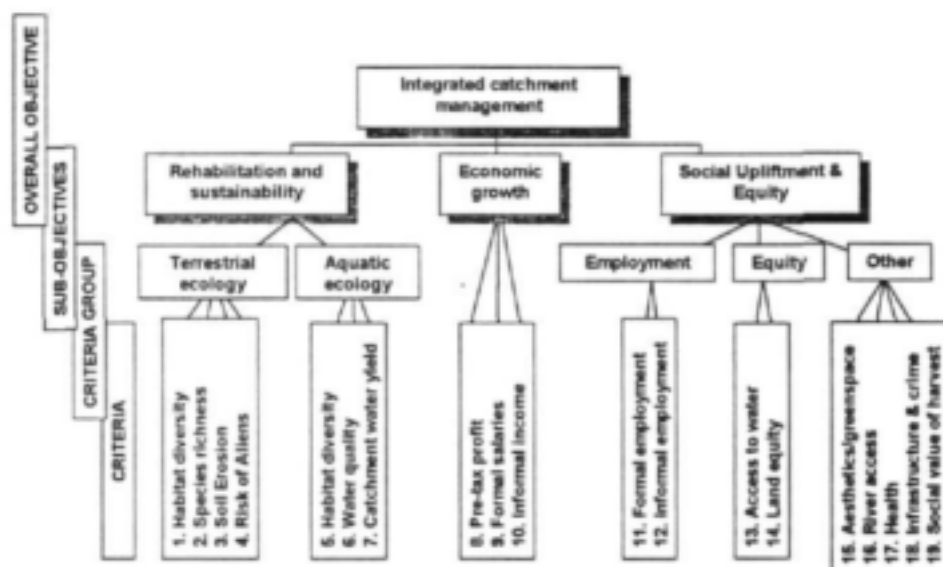
Figure 3.3. An example of a value tree.
