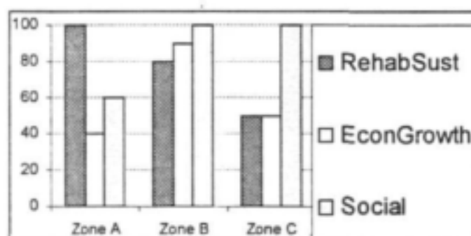
Figure 7.4. "Consensus" weights applied to the different zones for the three main criteria groups.
