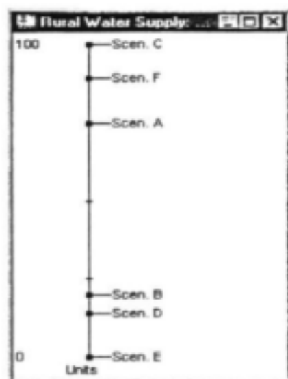
Figure 2.2. Illustration of a "thermometer" scale
