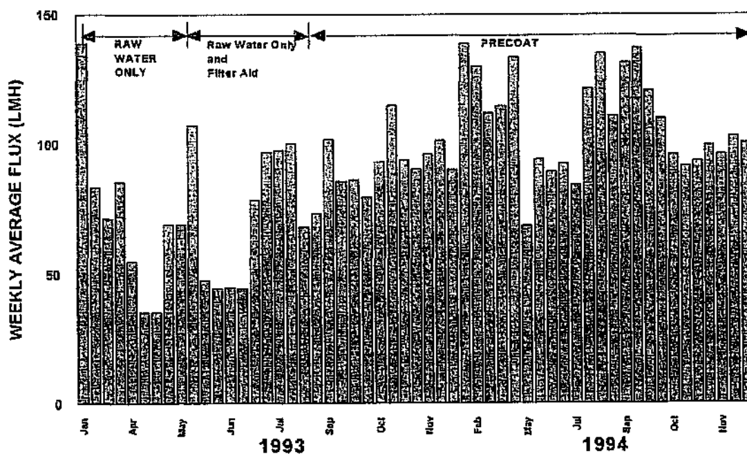
Figure 10 : Weekly Average Fluxes over Project Period
