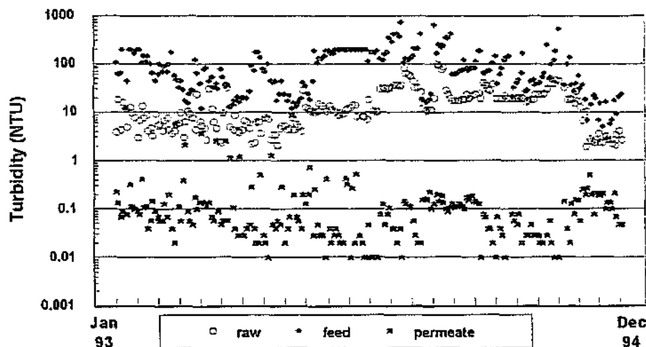
Figure 6 : Turbidity Removal History
