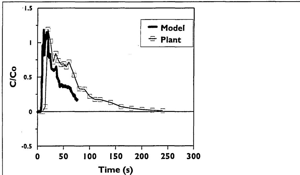
Figure 5.3 : Comparison of the RTD for the Plant and the Model
