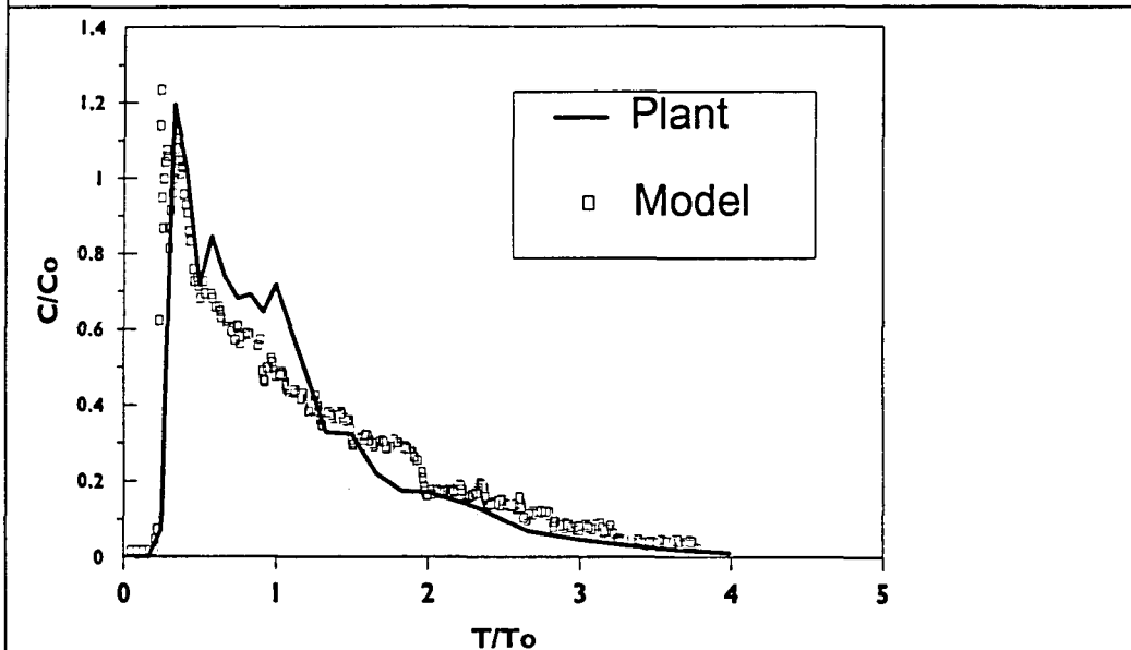
Figure 5.4 : Corrected Comparison of the RTD for the Plant and the Model
