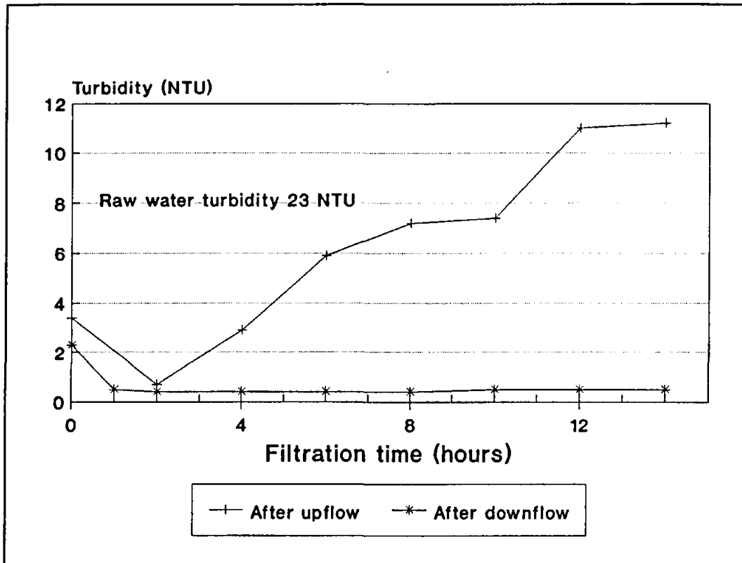
Figure 3.3 Turbidity removal at Hectorspruit plant for RUN HF 18.1: Filtration rate 18 m/h up; 9 m/h down and 14 mg/l \text{FeCl}_3
