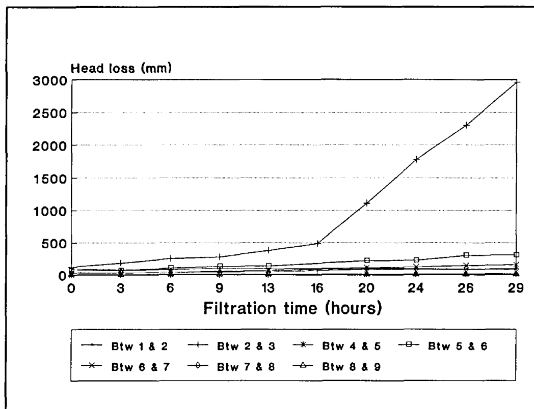
Figure C8 Head loss development in the filter for RUN V5.2: Filtration rate 5 m/h and 40 mg/l alum
