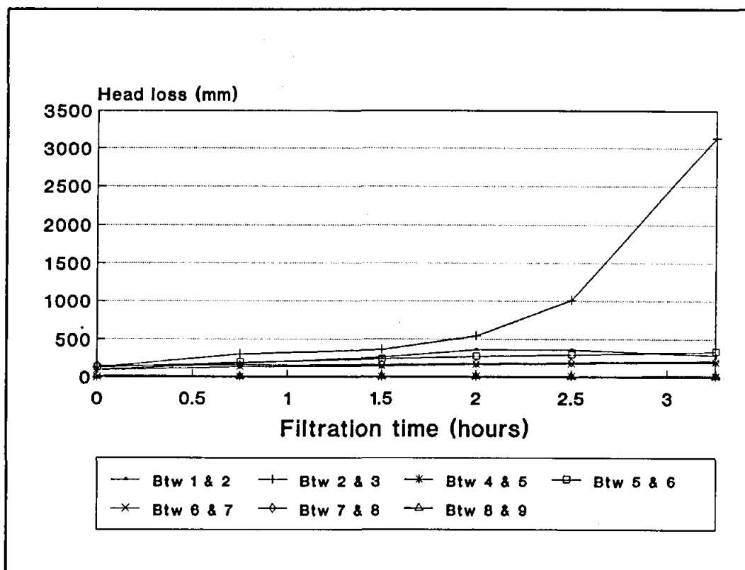
Figure C12 Head loss development in the filter for RUN V20.2: Filtration rate 20 m/h and 45 mg/ℓ alum
