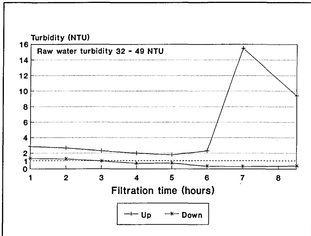
Figure C3 Turbidity removal at Vaalkop for RUN V10.1 Filtration rate 10 m/h, 7,5 mg/l \text{FeCl}_3 and 15 mg/l lime
