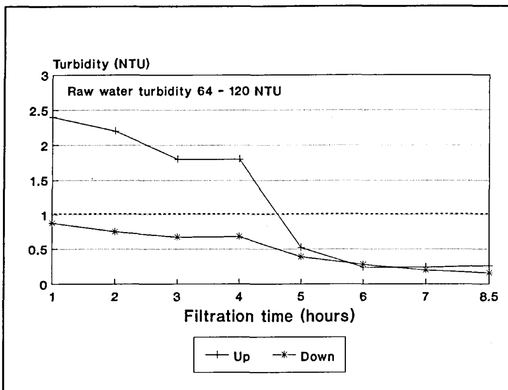
Figure C17 Turbidity removal at Vaalkop for RUN V10.4: Filtration rate 10 m/h, 7,8 mg/l \text{FeCl}_3 and 0,5 mg/l LT 22
