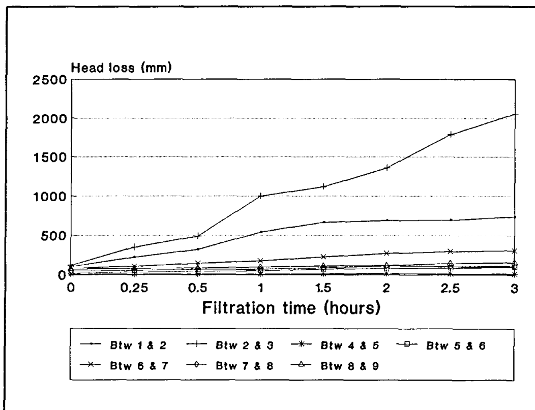
Figure D9 Head loss development in the filter for RUN R20.1: Filtration rate 20 m/h and 30 mg/ℓ alum
