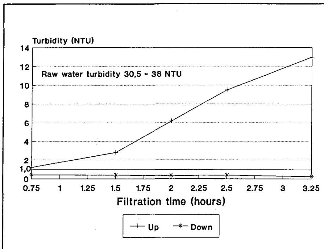
Figure C11 Turbidity removal at Vaalkop for RUN V20.2: Filtration rate 20 m/h and 45 mg/ℓ alum
