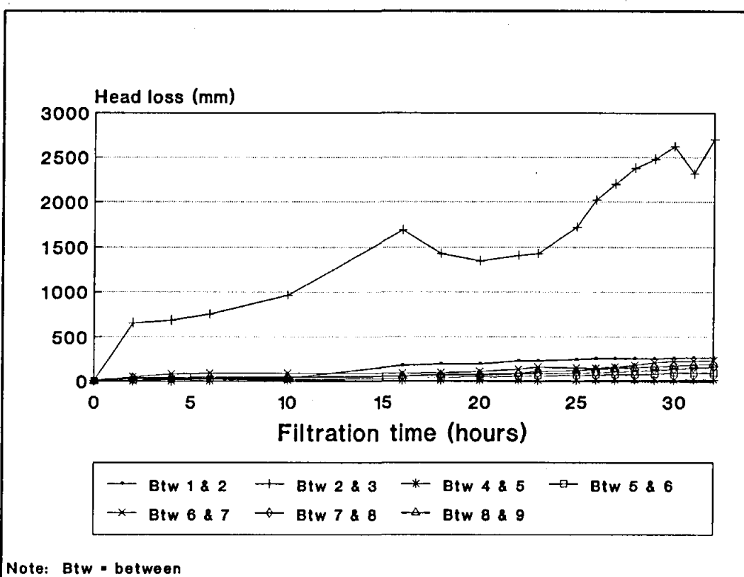
Figure B12 Head loss development in the filter for RUN H30.2: Filtration rate 30 m/h and 1 mg/l LT 22
