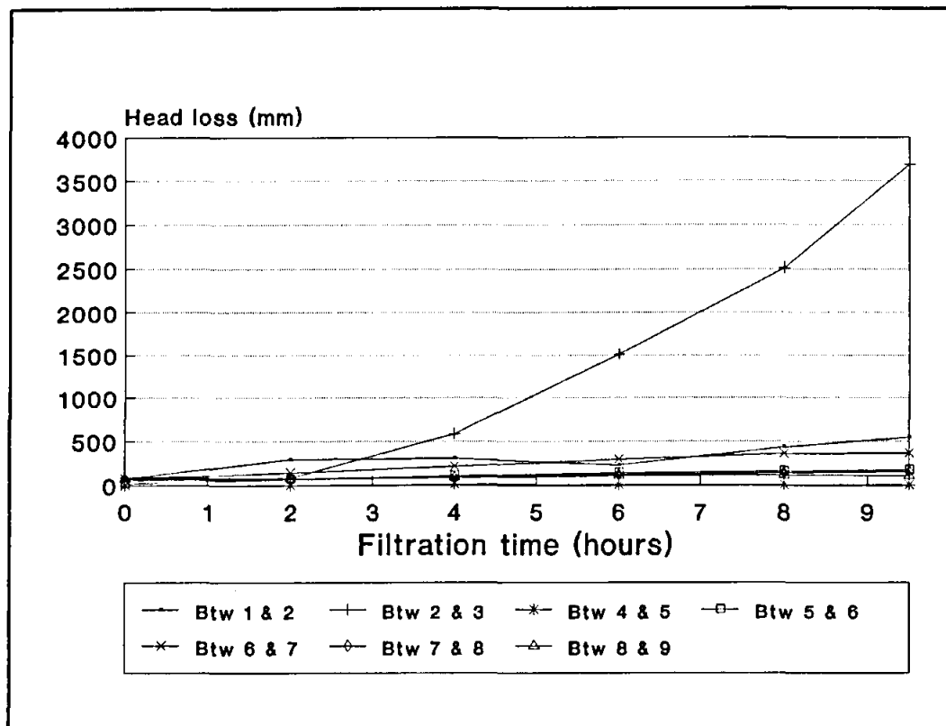
Figure D30 Head loss development in the filter for RUN 10.4: Filtration rate 10 m/h, 60 mg/ℓ alum and 0,5 mg/ℓ LT 22
