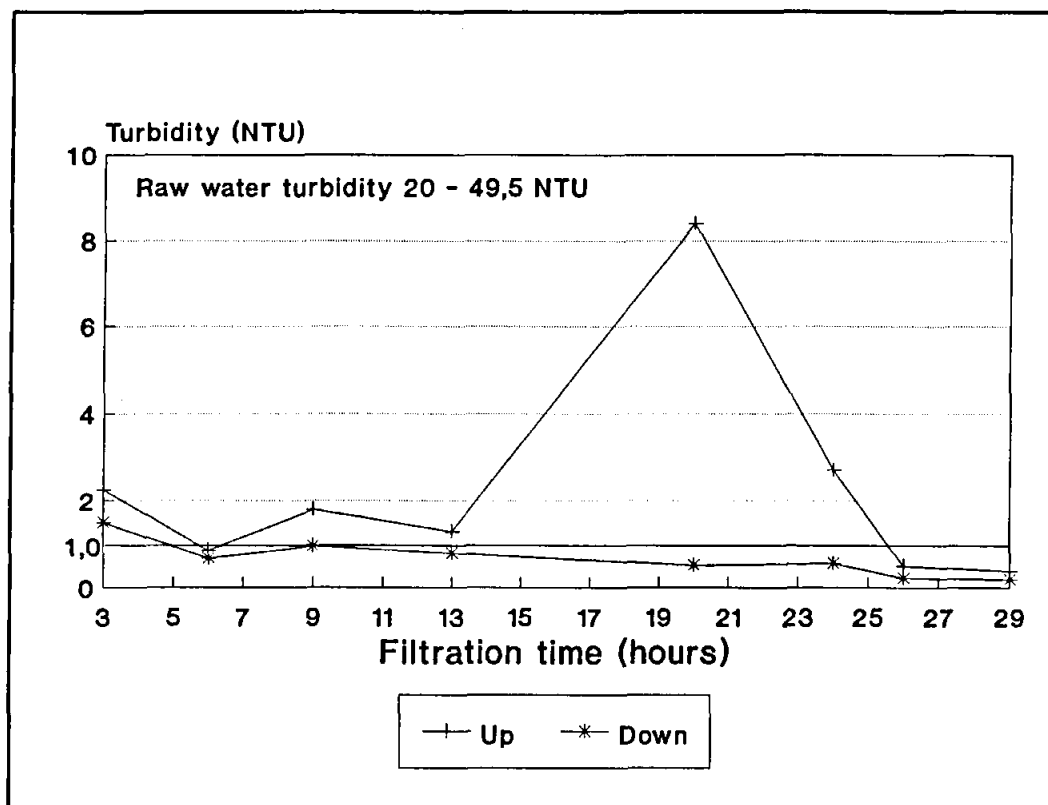
Figure C7 Turbidity removal at Vaalkop for RUN V5.2: Filtration rate 5 m/h and 40 mg/l alum
