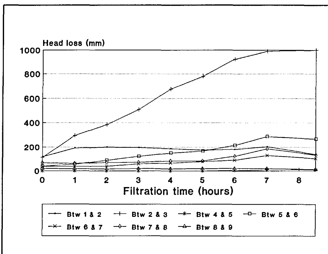
Figure C18 Head loss development in the filter for RUN V10.4: Filtration rate 10 m/h, 7,8 mg/l \text{FeCl}_3 and 0,5 mg/l LT 22
