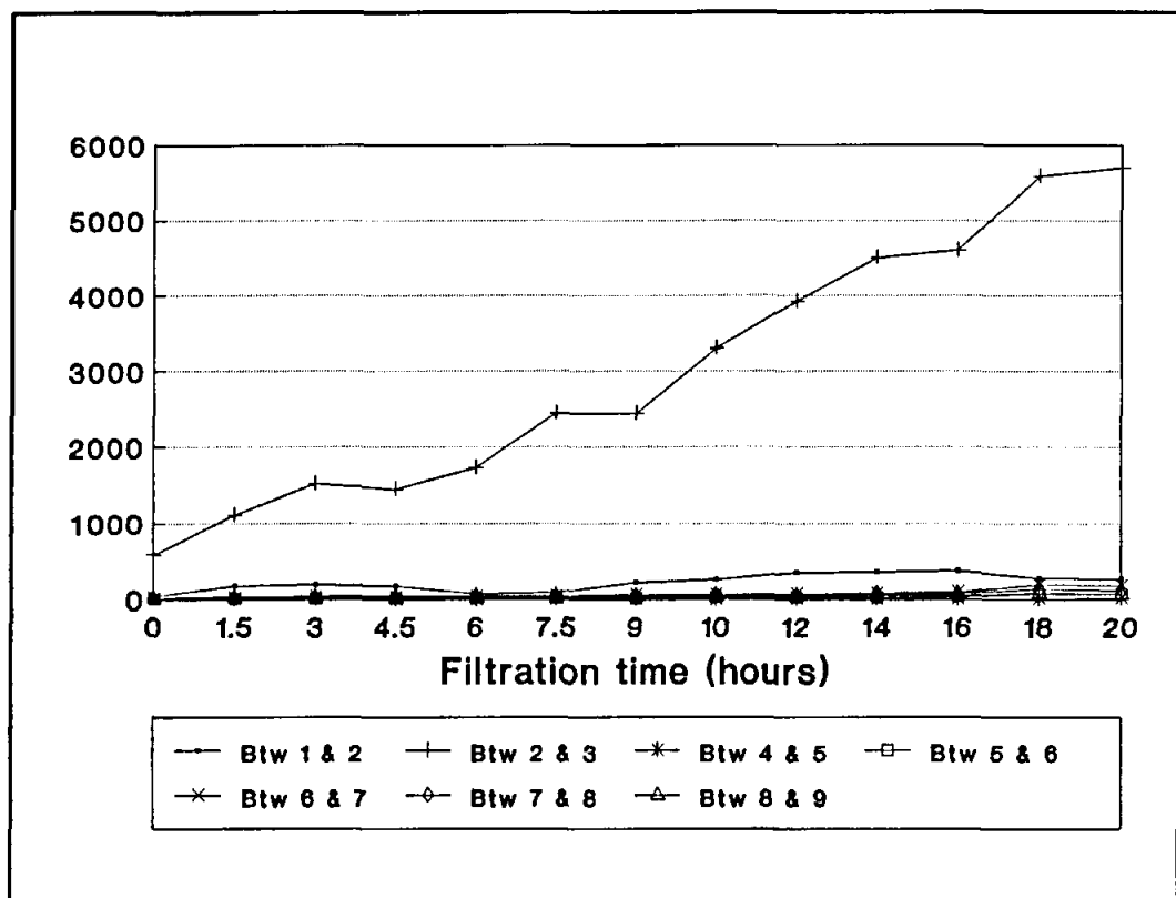
Figure D3 Head loss development in the filter for RUN 5.1: Filtration rate 5 m/h and 35 mg/ℓ alum
