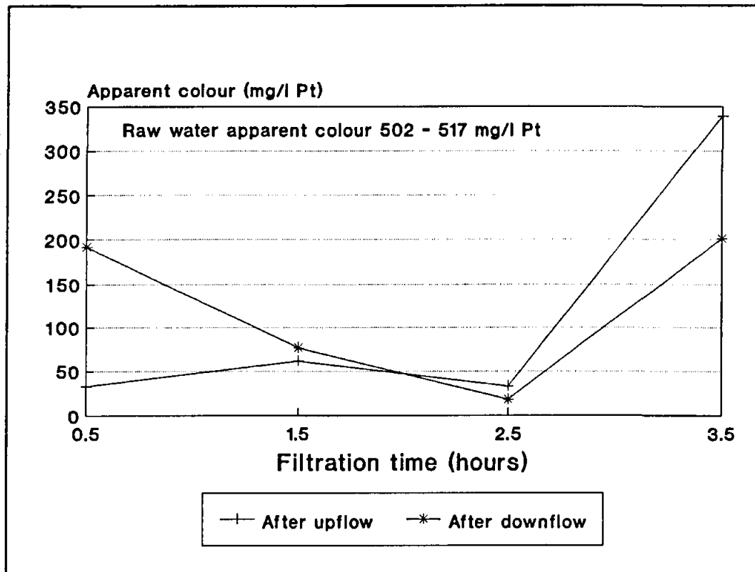
Figure E5 Apparent colour removal at Mossel Bay for RUN M20.1: Filtration rate 20 m/h and 100 mg/l alum
