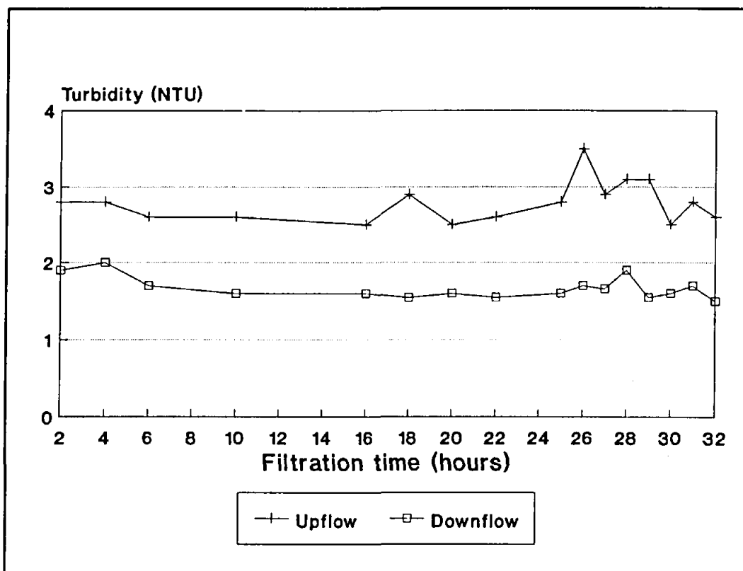
Figure B11 Turbidity removal at Hectorspruit for RUN H30.2: Filtration rate 30 m/h and 1 mg/l LT 22
