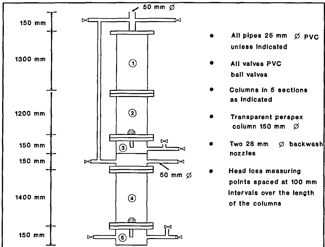
Figure 4.2 Lay-out and dimensions of the direct series filtration pilot plant
