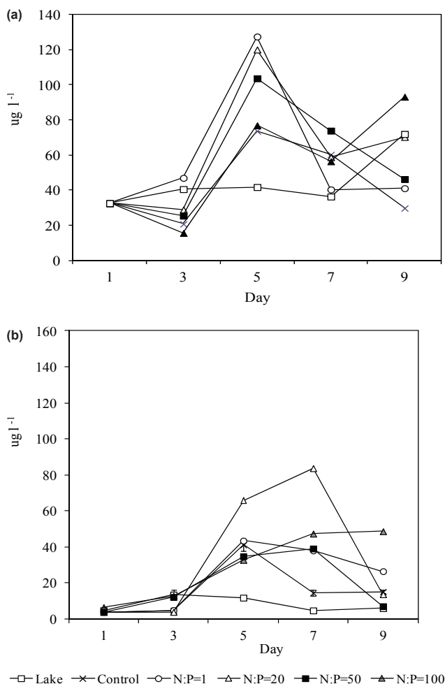
Figure 2 Chlorophyll a concentrations ( \mu\text{g}\cdot\text{l}^{-1} ) in different treatments during the experimental periods (a = Experiment 1, b = Experiment 2)
