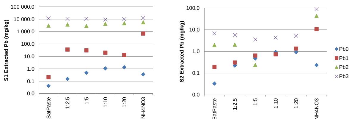
Figure 11: Pb concentrations extracted from S1 and S2 with different extracts
