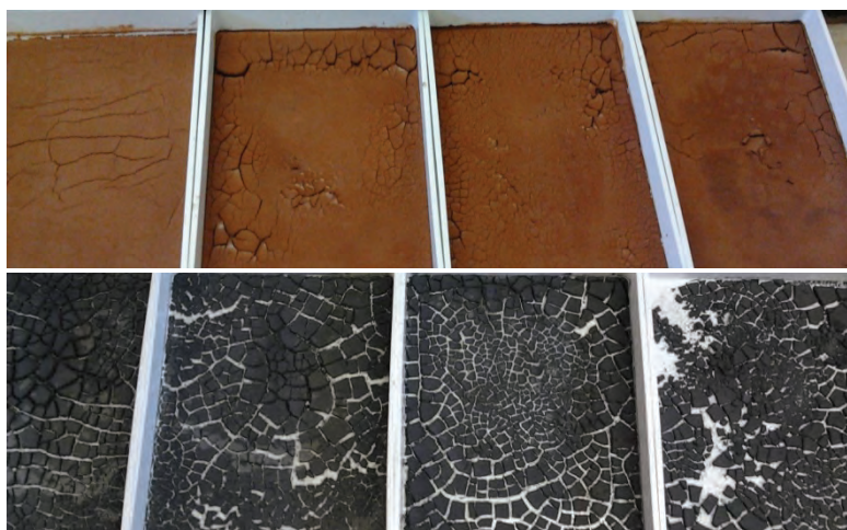
Figure 9: Drying of soils in trays
