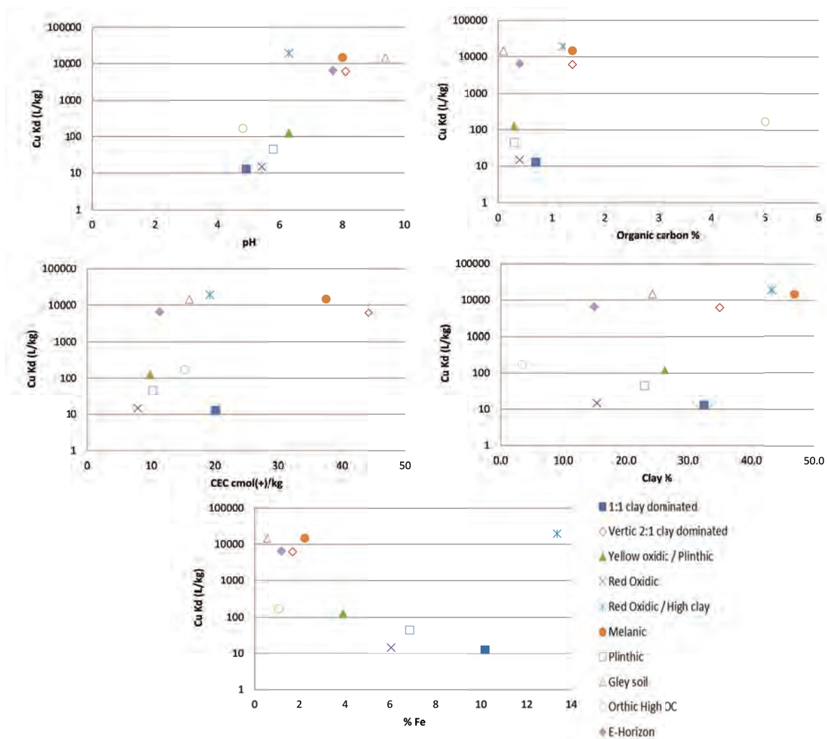
Figure 15: Correlation between Cu K_d and soil properties
