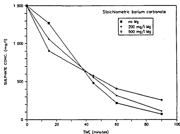
FIGURE 2 : The Effect of Magnesium Chloride on Sulphate Removal from a Calcium Sulphate Solution
