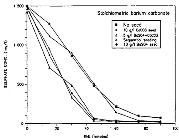
FIGURE 1 : Sulphate Removal from a Calcium Sulphate Solution Using Barium Carbonate : The Effect of Seeding
