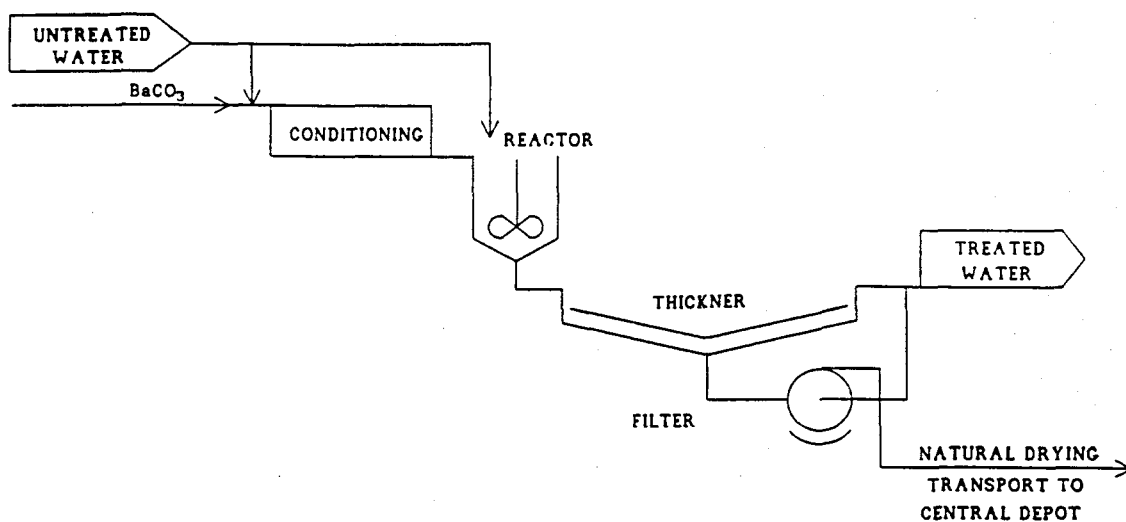
FIGURE 1 : Process Flow Diagram for the Treatment of Sulphate Rich Water with Barium Carbonate
