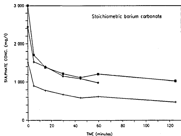
FIGURE 4 : Sulphate Removal from Different Concentrations of a Sodium Sulphate Solution Using Barium Carbonate
