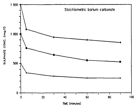
FIGURE 3 : Sulphate Removal from Different Concentrations of a Magnesium Sulphate Solution Using Barium Carbonate
