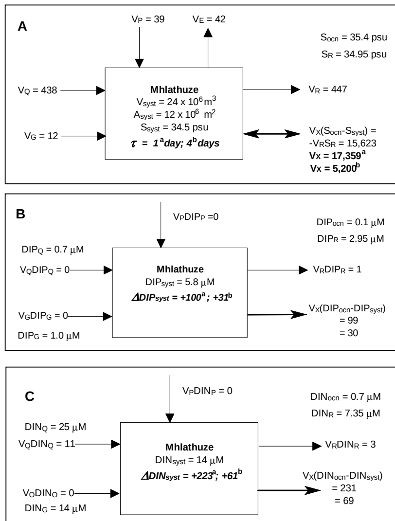
Figure 14. Water and salt budgets (A), dissolved inorganic phosphorous budget (B) and dissolved inorganic nitrogen budget (C) for the Mhlathuze Estuary. Water flux is presented in 10^6 \text{ m}^3 \text{ d}^{-1} and salt flux in 10^6 \text{ psu} \cdot \text{m}^3 \text{ d}^{-1} , whereas nutrient fluxes are in 10^3 \text{ mol m}^3 \text{ d}^{-1} .
