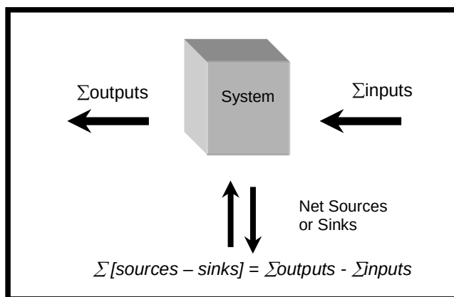
Figure 11. Generalised diagram indicating the components of the LOICZ budget procedure. (Adapted from Gordon et al. 1996).
