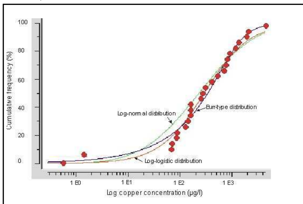
Figure 19. Cumulative distribution functions for the copper datasets (filled circles) based on log-normal, log-logistic and Burr-type distribution fitting using the Australian EPA software, BurrliOz. Data are for seawater acute toxicity 50% effect concentration ( LC_{50} ) endpoints for copper, n=25 , extracted from the aquatic toxicity information retrieval (ECOTOX) database.
