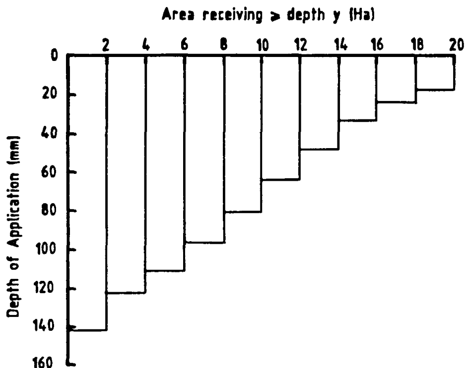
Figure 3.3 Example of an application depth vs area irrigated histogram for a 20Ha plot.
