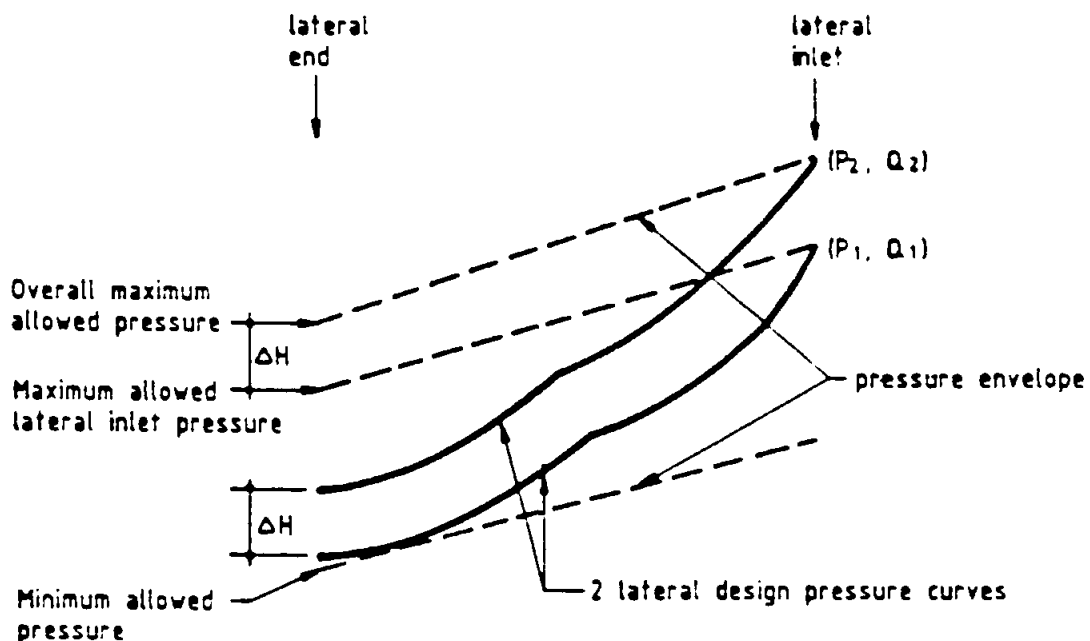
Figure 4.8: Calculation of the lateral pressure/discharge relationship
