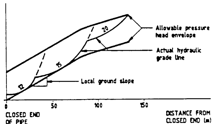
Figure 4.3(b) : Poly-plot design for pipe with SDR = 30 \text{ l/h/m}
