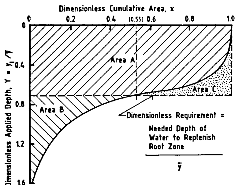
Figure 3.6 Analysis of the cumulative frequency distribution curve.
