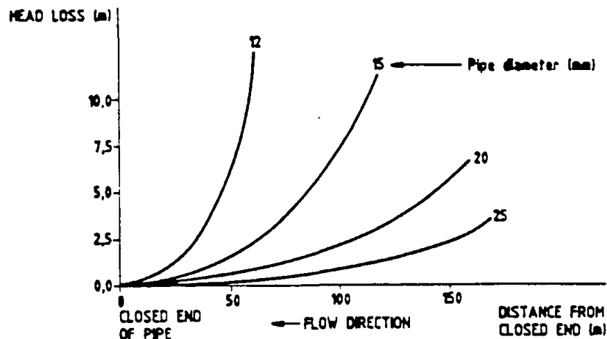
Figure 4.3(a) : Head loss curves for SDR = 30 \text{ l/h/m}
