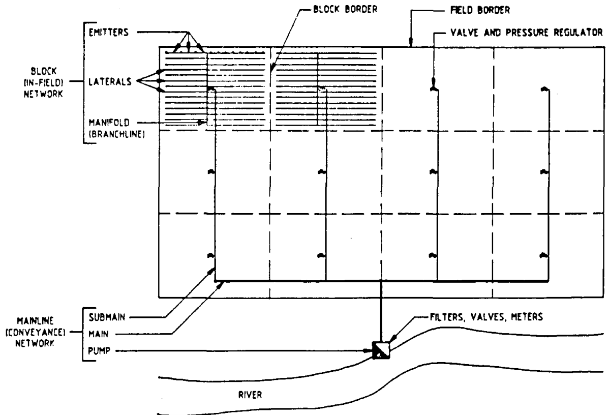
Figure 1.1 Diagrammatic representation of a typical irrigation system
