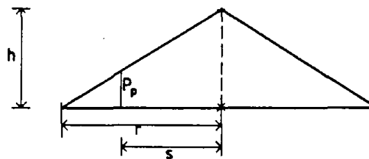
(b) section showing assumed triangular distribution
