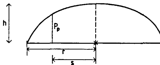
(c) section showing assumed elliptical distribution
