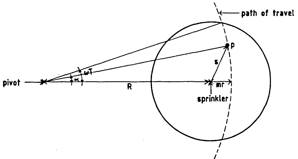
Figure 3.2(b) Analysis of distribution pattern for a moving sprinkler: center-pivot.
