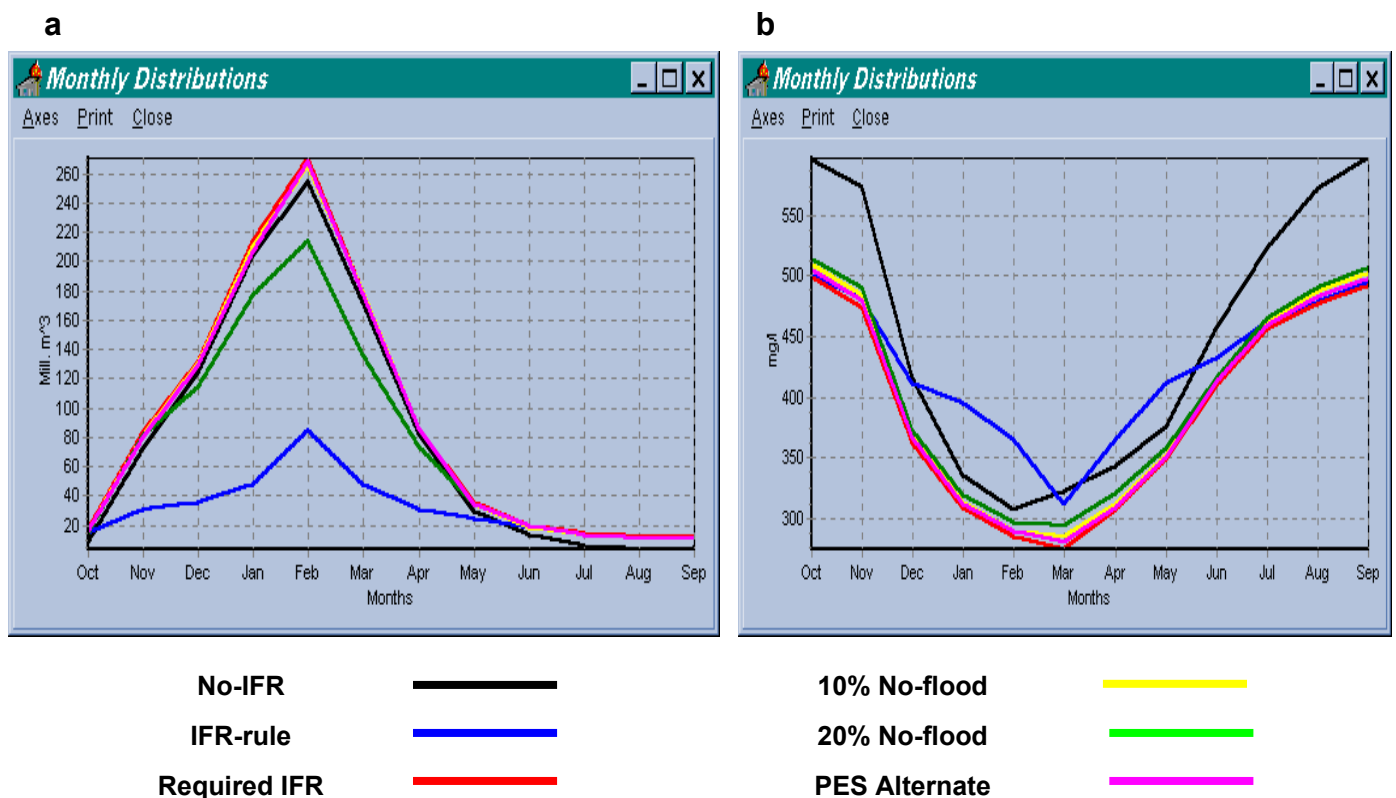
Figure 2.2 Mean monthly discharge in million cubic meters (a) and mean monthly salinity in mg/L (b) for IFR 13 as predicted under the different flow scenarios using TSOFT. Values calculated using the entire flow time-series (1920-1987). Flow scenarios given below the figures.
