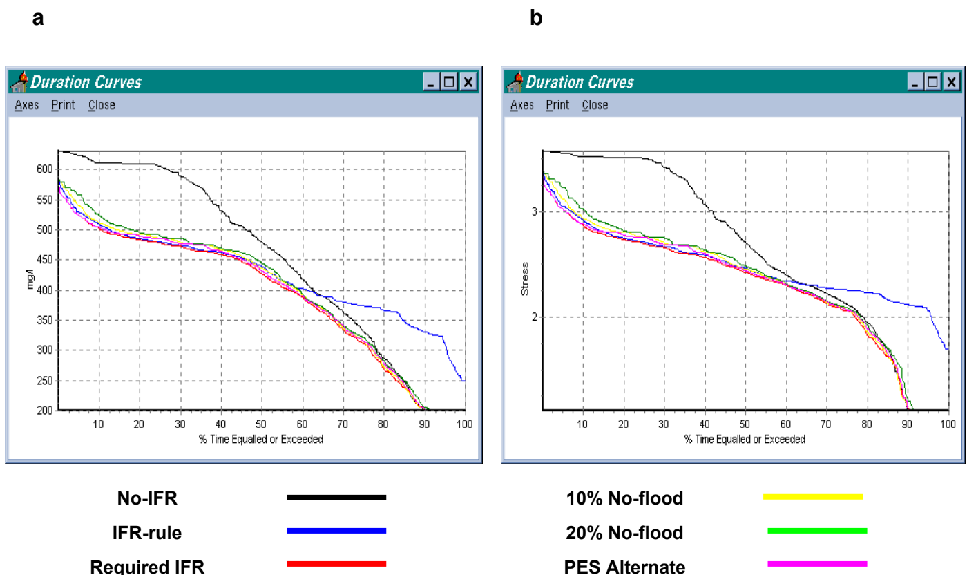
Figure 2.3 Salinity in mg/L (a) and stress (b) duration curves for IFR 13 as predicted under the different flow scenarios. Stress derived using a scale of 0-10 as described in the text.
