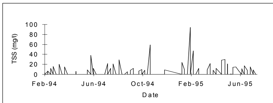
Figure A11 TSS at X2H016Q01.
