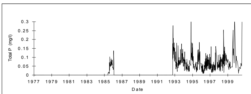
Figure A8 Total phosphorus at X2H016Q01.
