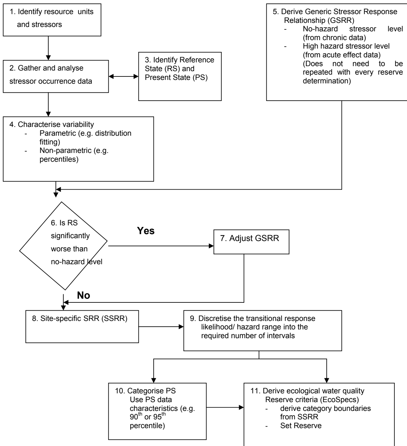
Figure 3.2 A procedure for applying site-specific stressor response relationships in setting the reserve.
