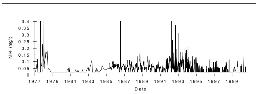
Figure A7 \text{NH}_4 at X2H016Q01.
