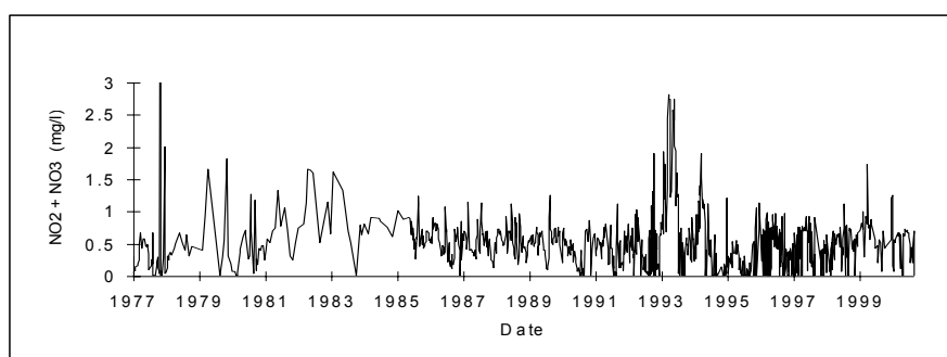
Figure A6 NO 2 and NO 3 at X2H016Q01.
