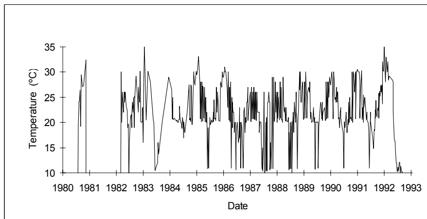
Figure A3 Historical water temperature at X2H016Q01.
