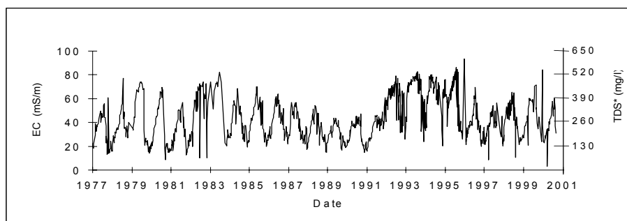
Figure A10 EC (TDS) at X2H016Q01. (*TDS = EC x 6.5).
