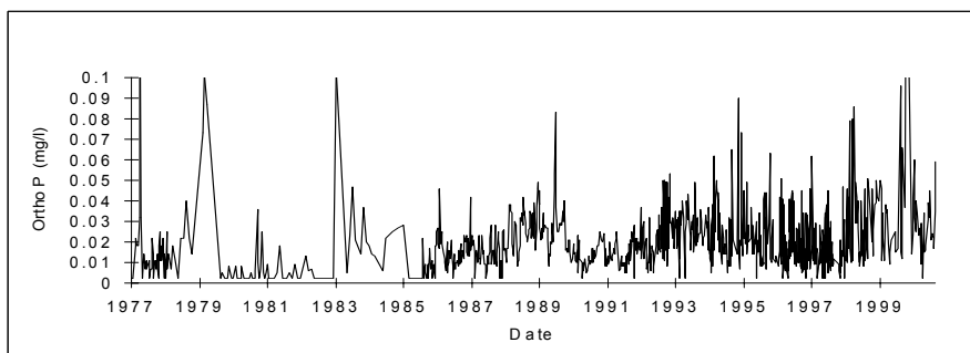
Figure A9 \text{PO}_4 at X2H016Q01.
