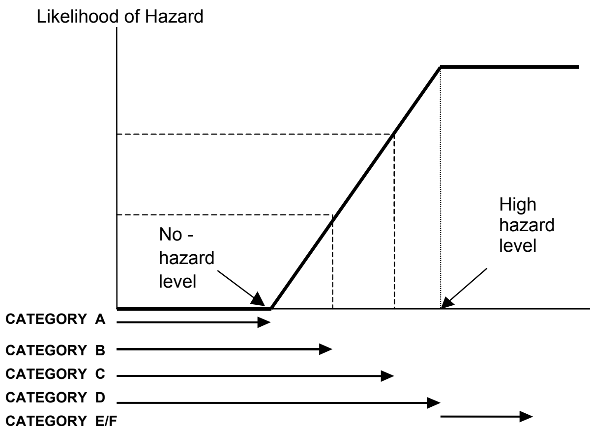
Figure 3.1 A typical stressor response relationship.
