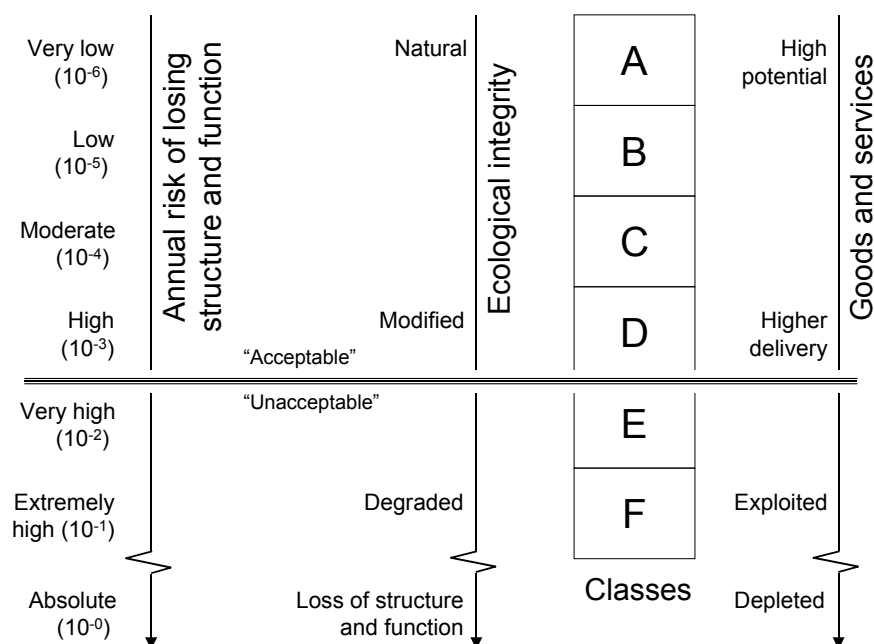
Figure A1 Relation between risk and water resource classification (Claassen, in prep).
