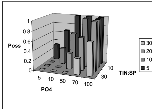
Figure 3.3 Possibility of response as a function of nutrient parameters.
