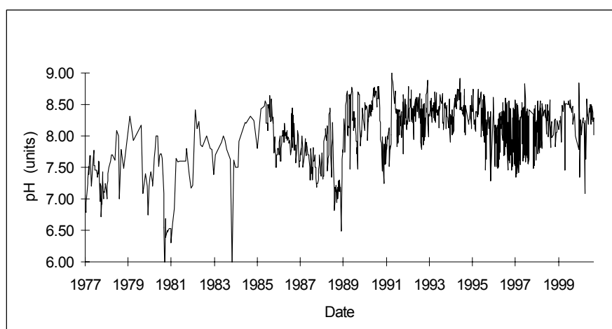
Figure A5 pH at X2H016Q01.
