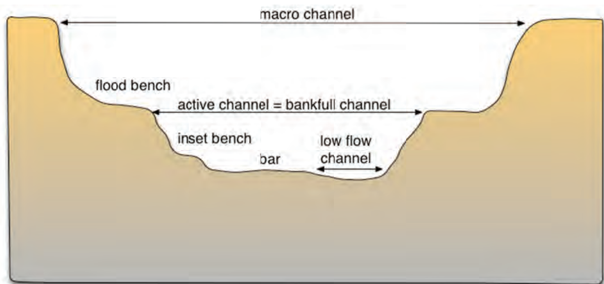
Figure 4.2 Channel features
