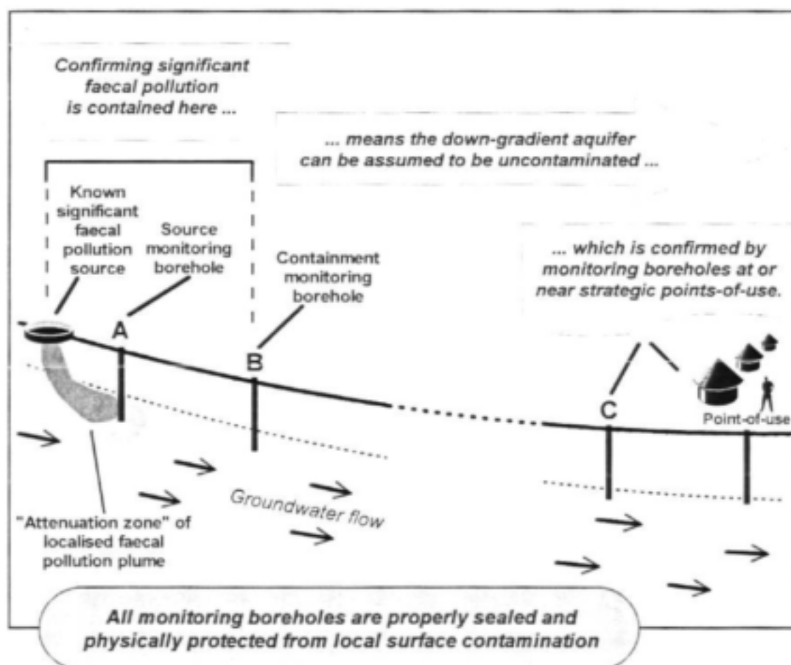
Figure 4.2. Illustration of the three types of monitoring boreholes and the philosophy behind each.
