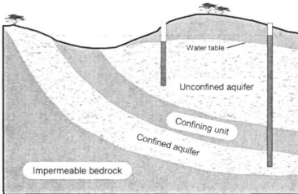
Figure 2.2. Schematic illustration of a confined and an unconfined aquifer (adapted from Purdue University, 1998).
