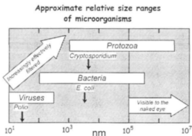
Figure 2.9. Approximate relative sizes (nm) of microorganisms.
