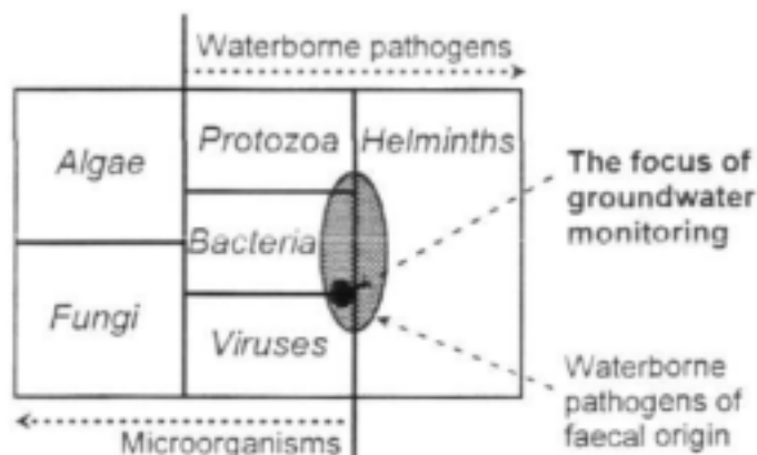
Figure 2.4. The specialised microbiological focus of groundwater monitoring.
