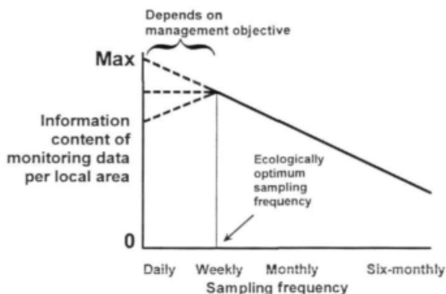
Figure 4.1. Schematic illustration of the relationship between information content and sampling frequency.
