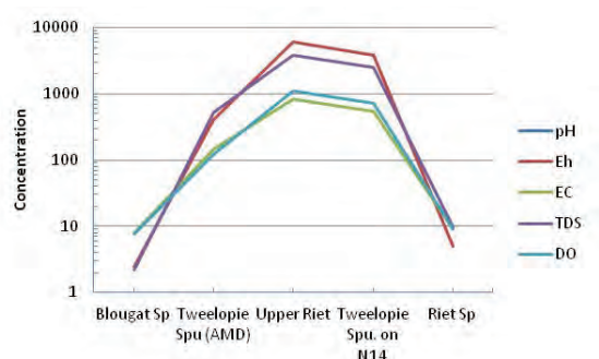
Figure 7: Variation of field measured parameters (Table 3) along a Rietspuit.
