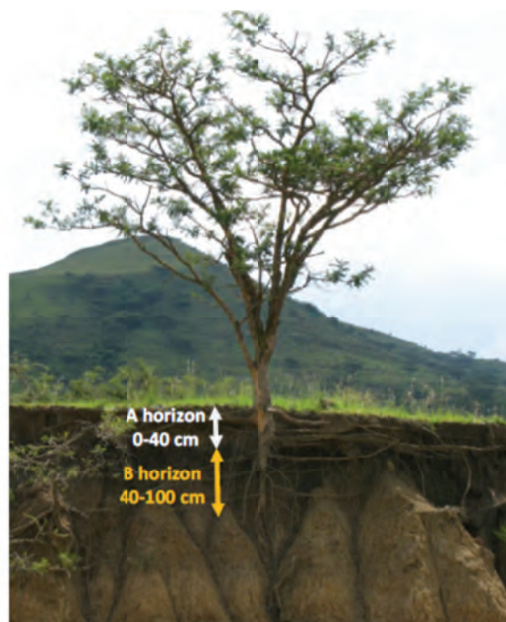
Figure 20: Assumed uptake zones from A and B horizons of the Acacia sieberiana , showing root distribution of a tree on the edge of the gully.
