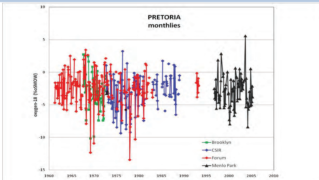
Figure 4: ^{18}\text{O} trend of monthly samples from four sites in Pretoria since 1958.
