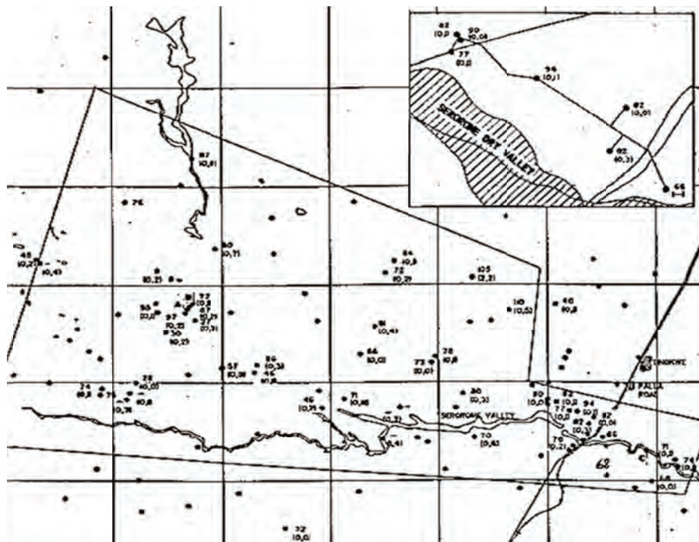
Figure 5: Geographic distribution of 14 C and 3 H values in groundwater. No clear regional trends are observable. Inset: Values for the pre-existing Palla Road wellfield boreholes.
