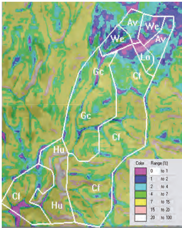
Figure 28: Six dominant soil sequence zones (hillslope types) found in the Mkabela catchment. Colours represent the slope range, (after le Roux et al. , 2006).
