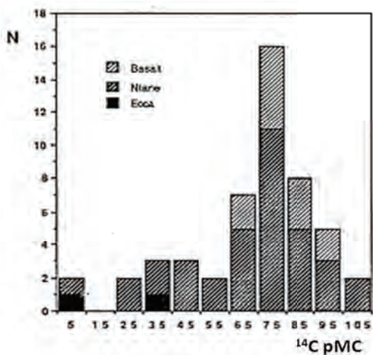
Figure 4: Frequency histogram of 14 C values displayed according to the lithological horizons in which they were sampled
