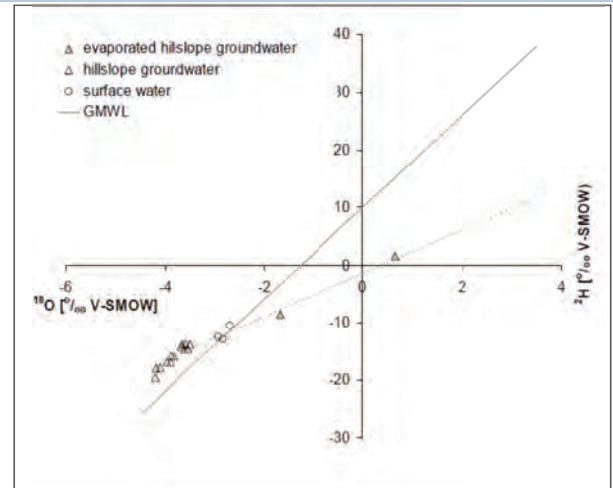
Figure 13: Relationship between \delta^{18}\text{O} and \delta^2\text{H} for rainfall, runoff and hillslope groundwater during August 2004 (After Lorentz et al., 2008).
