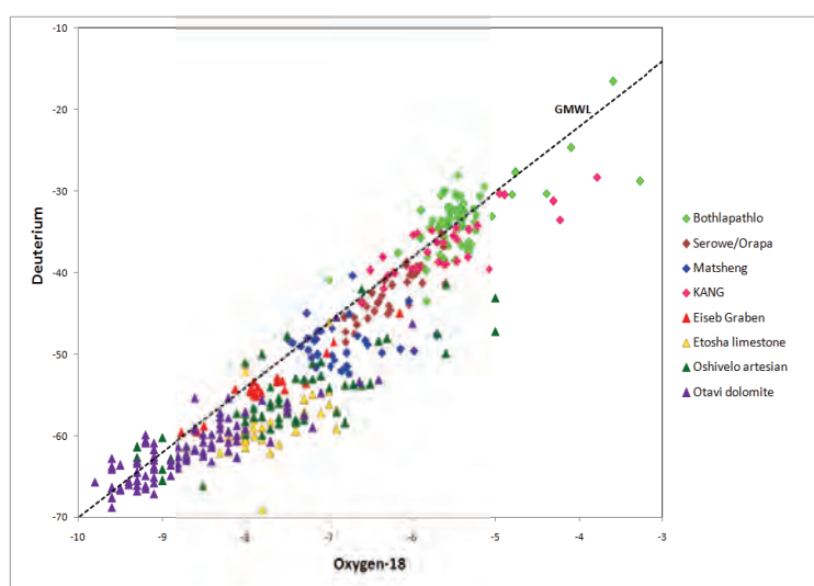
Figure 5: Deuterium- 18 O plot for various projects throughout the Kalahari
