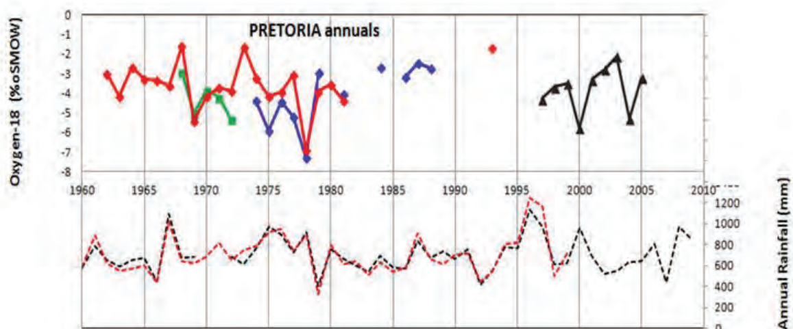
Figure 12: 18 Oxygen trend of annual mean values of data from four sites in Pretoria. The dashed line indicates total annual rainfalls of the same stations.
