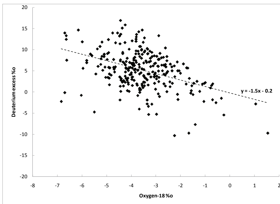
Figure 17: Plot of D_{xs} (deuterium excess) against 18 O of the groundwater samples from the DWA groundwater pollution programme. The RMS linear trend line through the points is shown.
