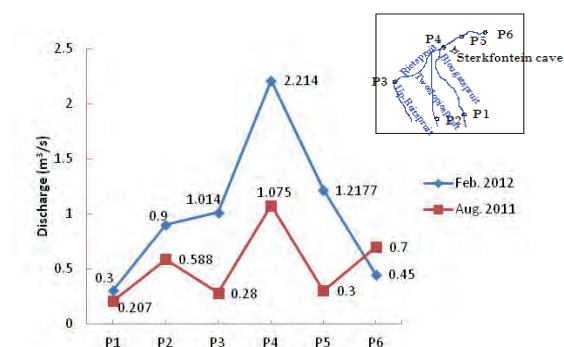
Figure 6: Discharge variation along Rietspruit and its tributaries in the CHKWHS
