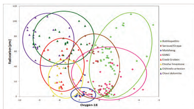
Figure 6: 14 C- 18 O plots for various projects throughout the Kalahari
