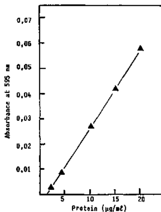
Figure 6.6 : Calibration curve for protein determination.
