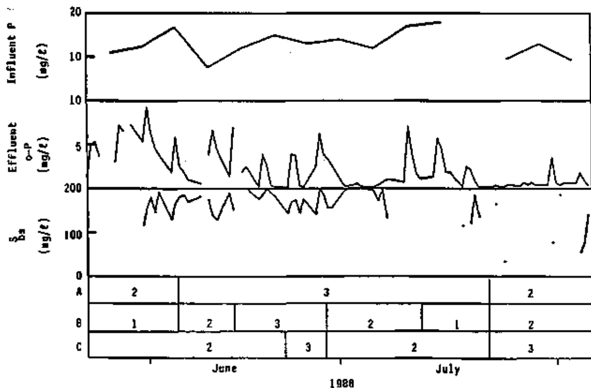
Figure 5.22 : Relationship between S_b , effluent phosphate and PHB accumulation in the anaerobic zone (A); PHB utilisation in the anoxic zone (B) and PHB utilisation in the aerobic zone (C) in Northern Works Module 3
