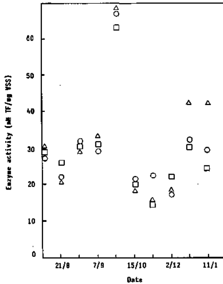
Figure 7.26 : Dehydrogenase activity in the anaerobic: ● ; anoxic: △ ; aerobic: □ ; zones of Beshkoppie with B-HO-butyrate as substrate
