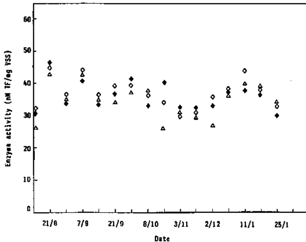
Figure 7.25 : Dehydrogenase activity in the anaerobic: ◇ ; anoxic: △ ; aerobic: ◆ ; zones of Northern Works Module 2 with glucose as substrate
