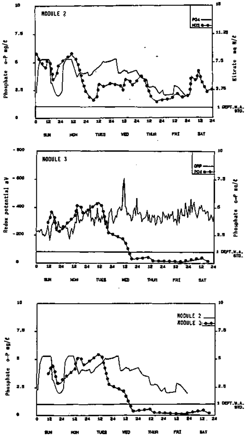
Figure 2.4 : Examples of graphs constructed from data captured by Logger 10-16 April 1988
