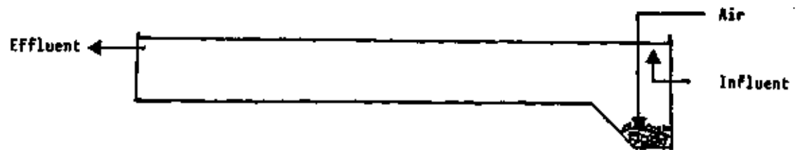
Figure 3.1 : Side elevation of the primary sedimentation tanks at Northern Works
