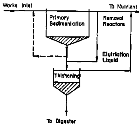
Figure 4.3 : Primary Sludge Accumulation and Extrusion Thickening
