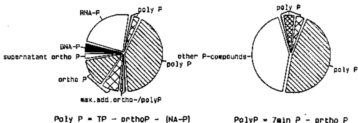
Figure 7.17 : Phosphorus fractionation of activated sludge from Northern Works
