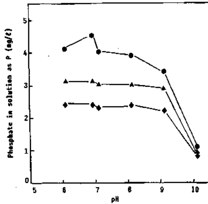
Figure 7.4 : Effect of pH on phosphate precipitation in Goudkoppies influent
