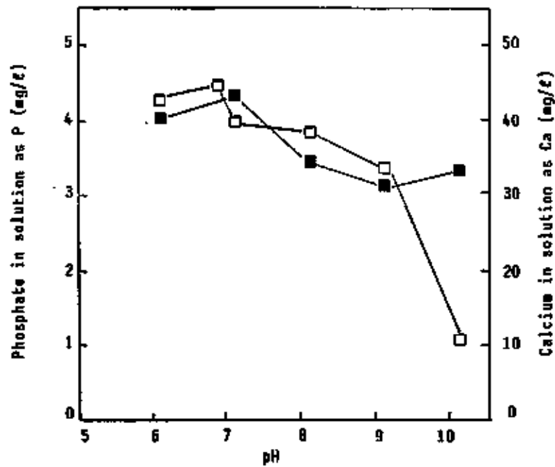
Figure 7.2 : Effect of pH on phosphate and calcium precipitation in Goudkoppies influent ■—■ calcium; □—□ phosphate
