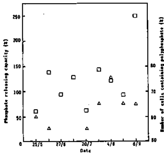
Figure 5.39 : Effect of phosphate releasing capacity: □ ; and intracellular polyphosphate: △ ; Goudkoppies
