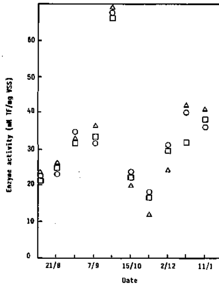
Figure 7.27 : Dehydrogenase activity in the anaerobic: ● ; anoxic: △ ; aerobic: □ ; zones of Beshkoppie with glucose as substrate
