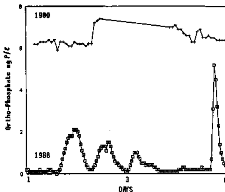
Figure 3.10 : Effluent phosphate concentration over a 5 day period in 1980 and 1988
