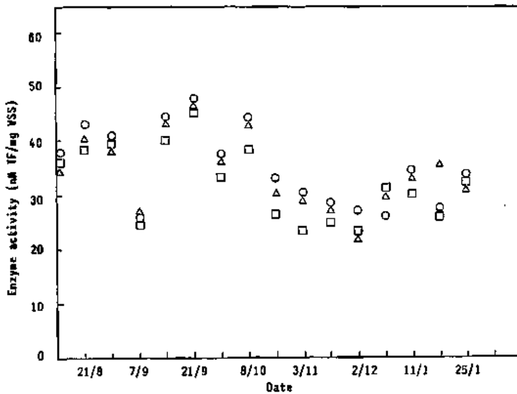
Figure 7.21 : Dehydrogenase activity in the anaerobic : □ ; anoxic : △ ; aerobic : ○ zones of Goudkoppies with \beta -HD-butyrate as substrate.
