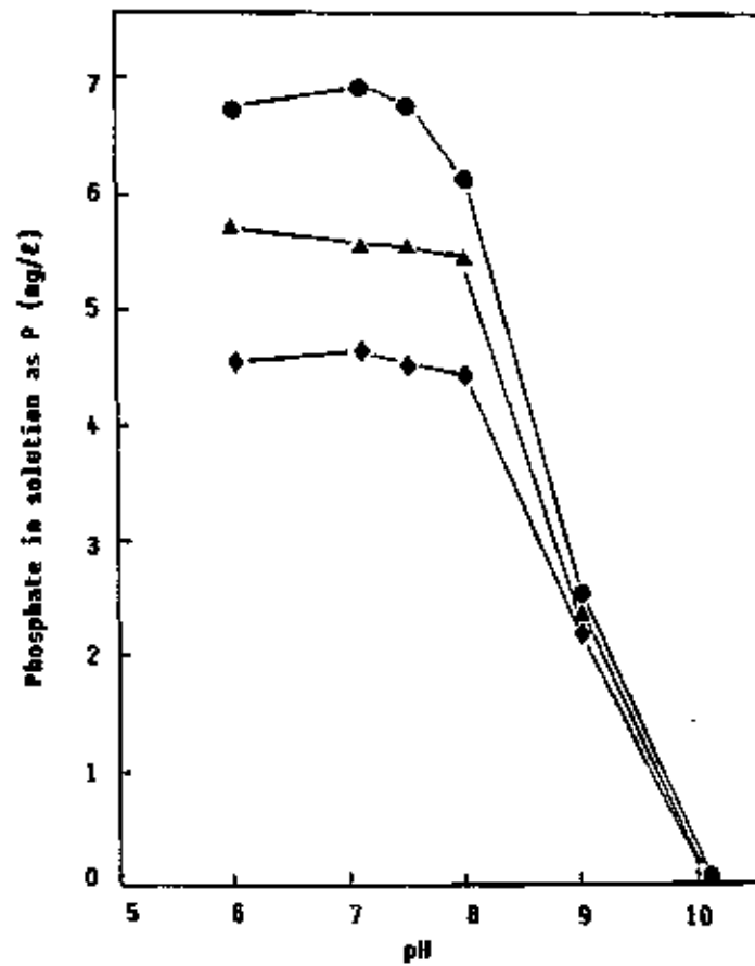
Figure 7.5 : Effect of pH on phosphate precipitation in Goudkoppies influent
