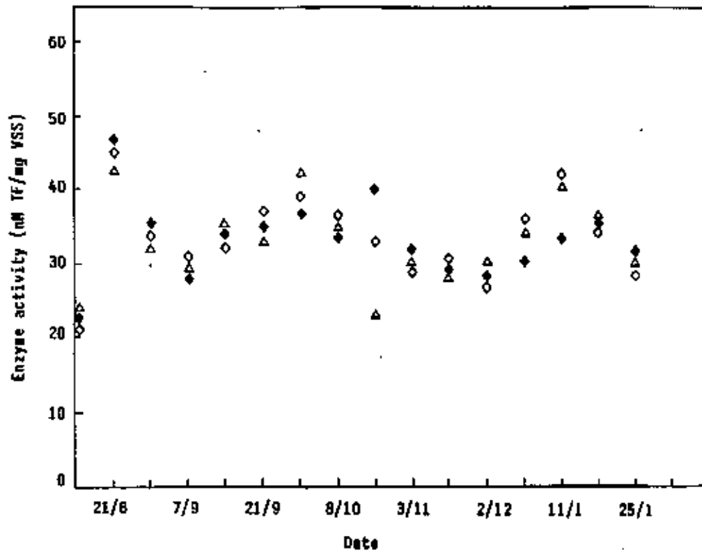
Figure 7.24 : Dehydrogenase activity in the anaerobic: ◇ ; anoxic: △ ; aerobic: ◆ ; zones of Northern Works Module 2 with \beta -HD-butyrate as substrate
