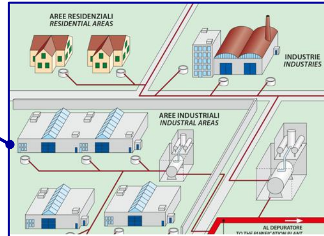
Sewerage Networks
