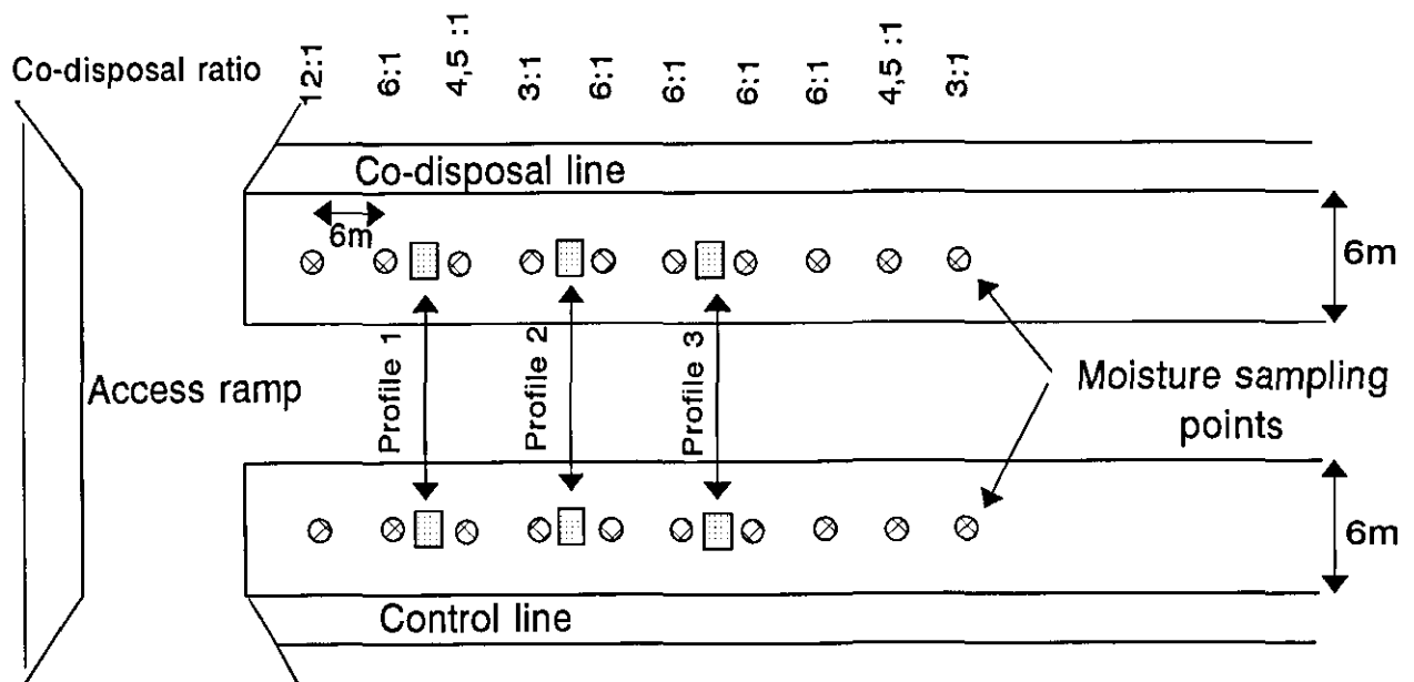
Figure 6.2 Location of the moisture sampling points and moisture profile holes on the experimental lines.
