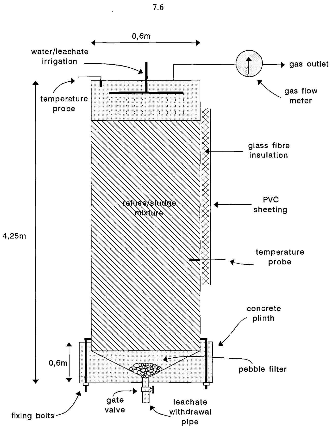
Figure 7.1 Schematic diagram of the lysimeters utilised in the lysimeter research.
