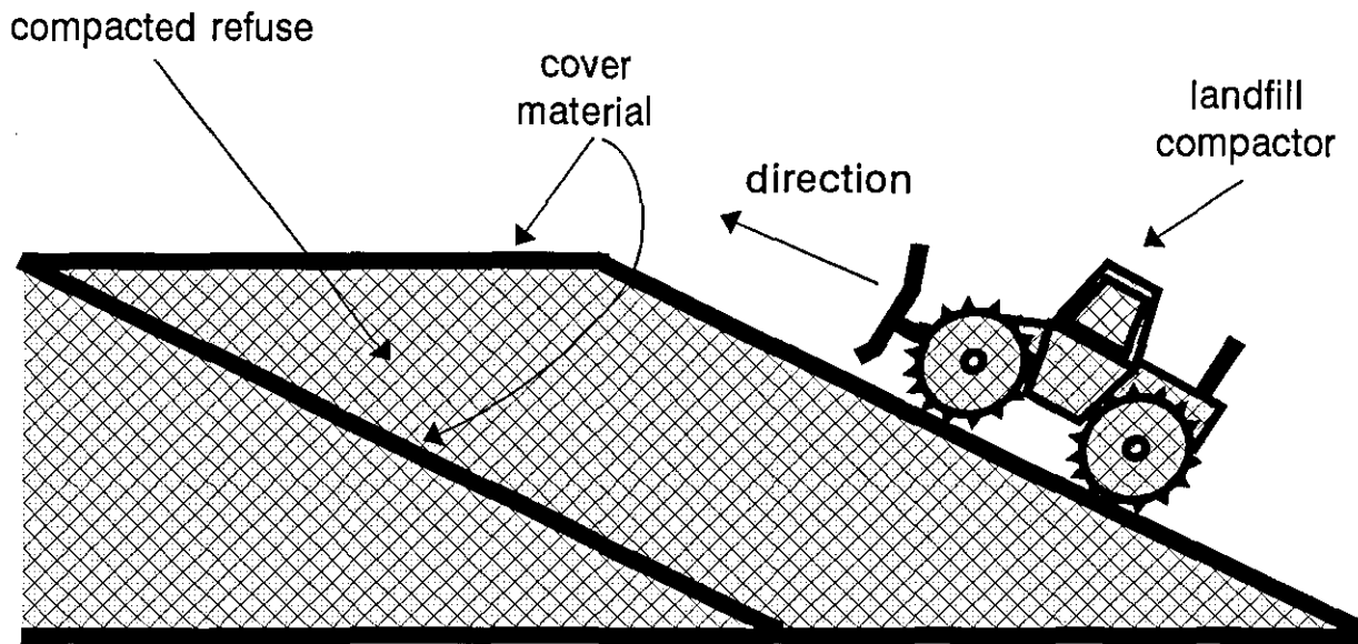
Figure 5.3 Landfill compactor operating up the slope.
