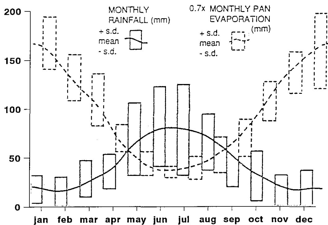
Figure 13.5 Summary of climatic parameters at Coastal Park landfill (Blight et al. , 1990).
