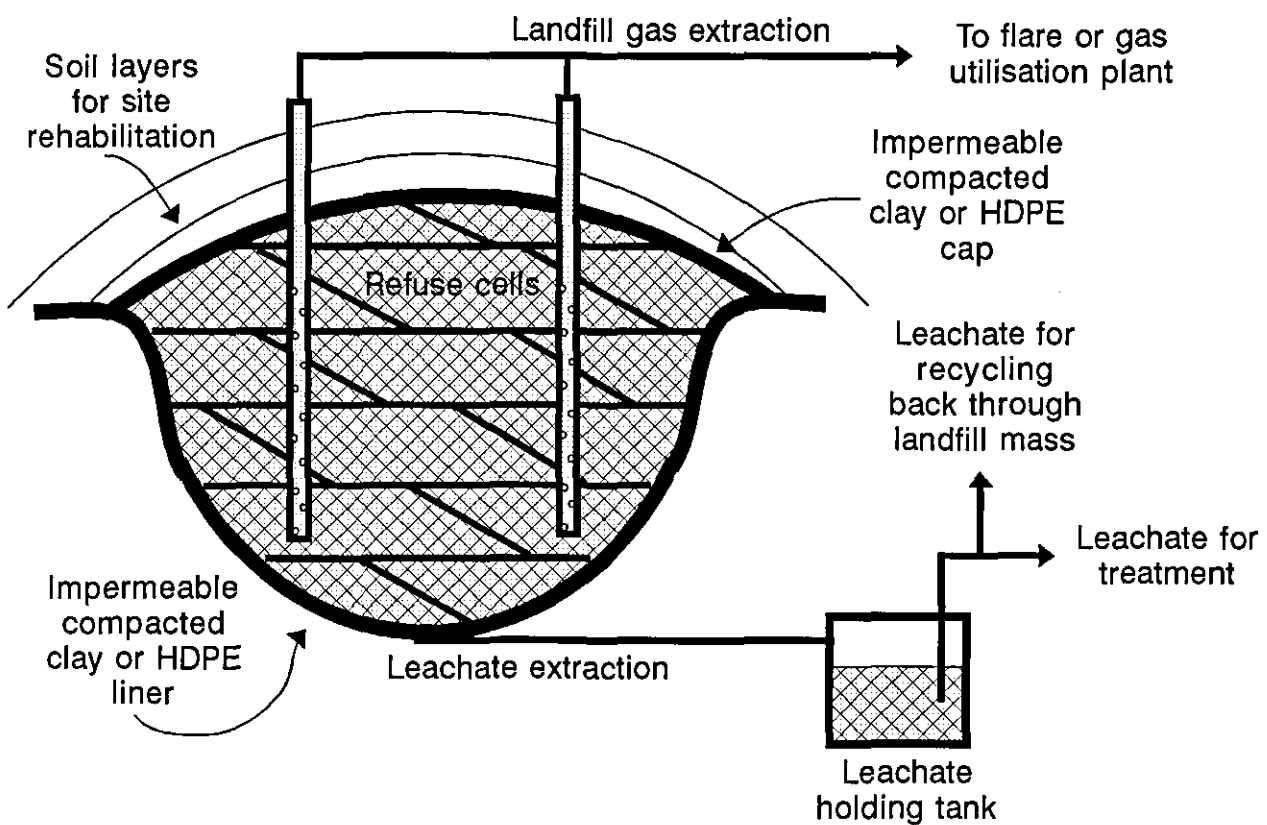
Figure 5.4 Typical containment landfill with the necessary environmental protection.
