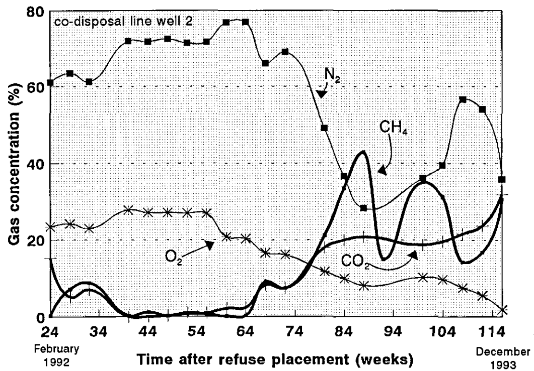
Figure 6.12 Landfill gas concentrations for the second set of gas wells in the control and co-disposal lines.
