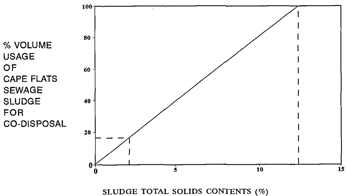
Figure 13.10 Volume usage of available Cape Flats digested sludge for co-diposal with refuse at Coastal Park as a function of the degree of dewatering of the sludge.
