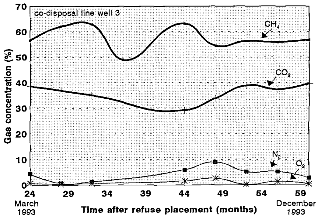
Figure 6.13 Landfill gas concentrations for the third set of gas wells in the control and co-disposal lines.
